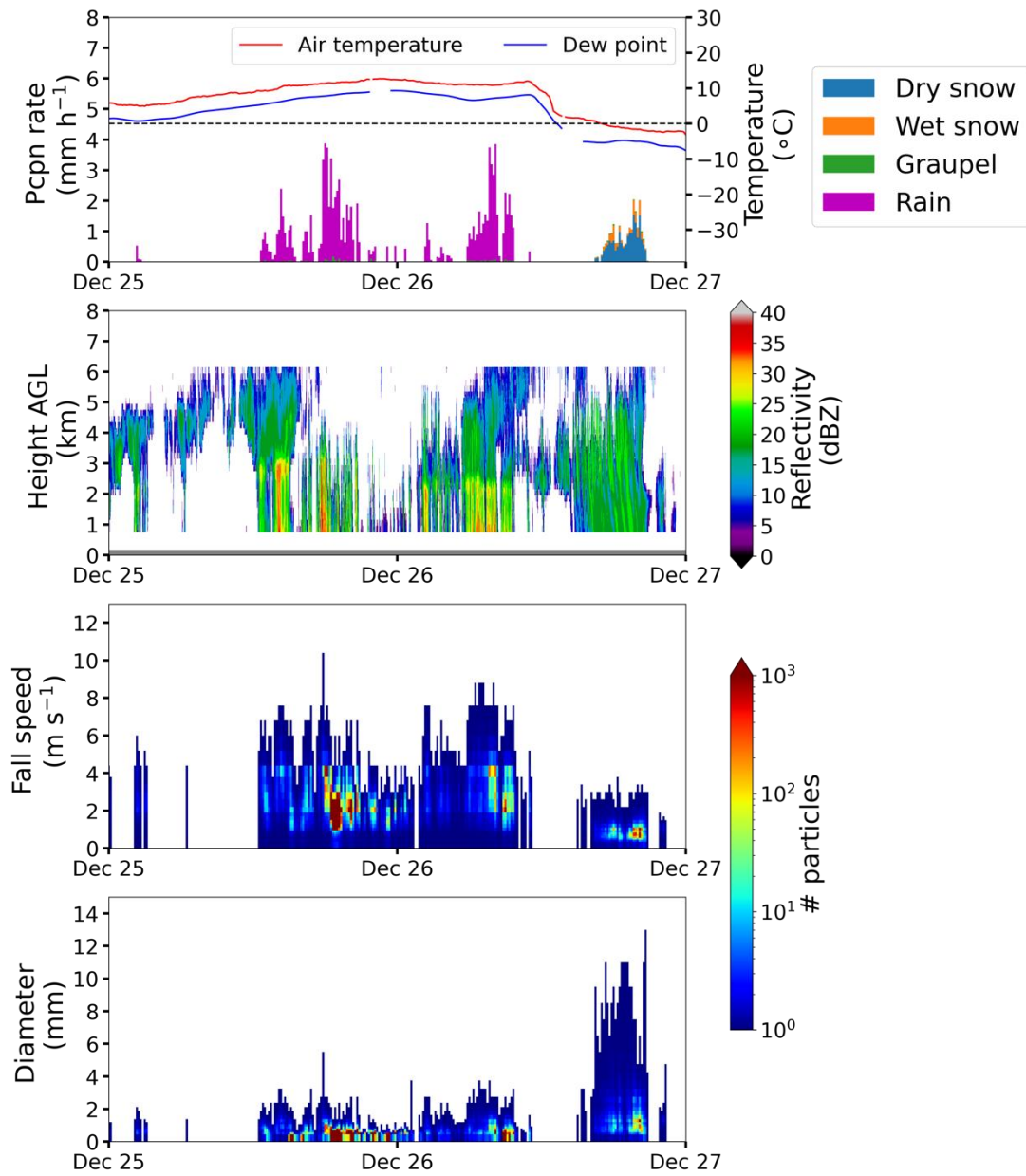
541 Figure 8: Fixed Station storm measurements. From top to bottom, (a) air temperature and precipitation. The 542 precipitation type is derived from disdrometer data using equations in Rasmussen et al. 1999 and Ishizaka et al. 2013, 543 and is not included in the dataset. (b) radar reflectivity, (c) particle fallspeed, and (d) diameter (both from the Parsivel 544 disdrometer), measured at the Fixed Station from 0000 UTC 25 December 2020 to 2359 UTC 26 December 2020. 545 Temperature, dew point, precipitation, and disdrometer data are shown as 10-minute averages. Micro rain radar 546 (MRR) data are at 10 second resolution, with a vertical resolution of 200 m.
