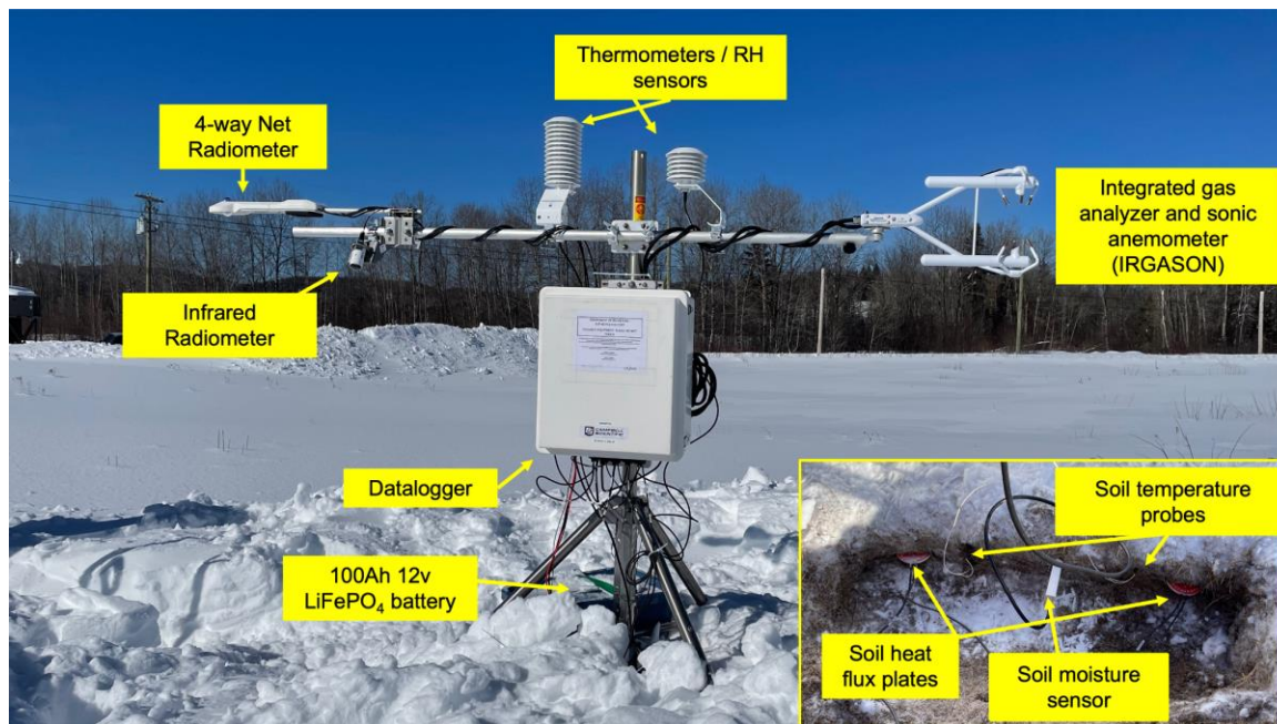
212 Figure 4: The Fixed Station flux tripod. An open-path eddy-covariance system consisting of an Infrared Gas Analyser 213 and Sonic Anemometer (IRGASON), soil temperature probes, a soil moisture sensor, a net radiometer, an infrared 214 radiometer, and temperature/RH sensors. This tripod was installed for the melt period from 5 March to 30 April 2021. 215 Picture taken 5 March 2021.
