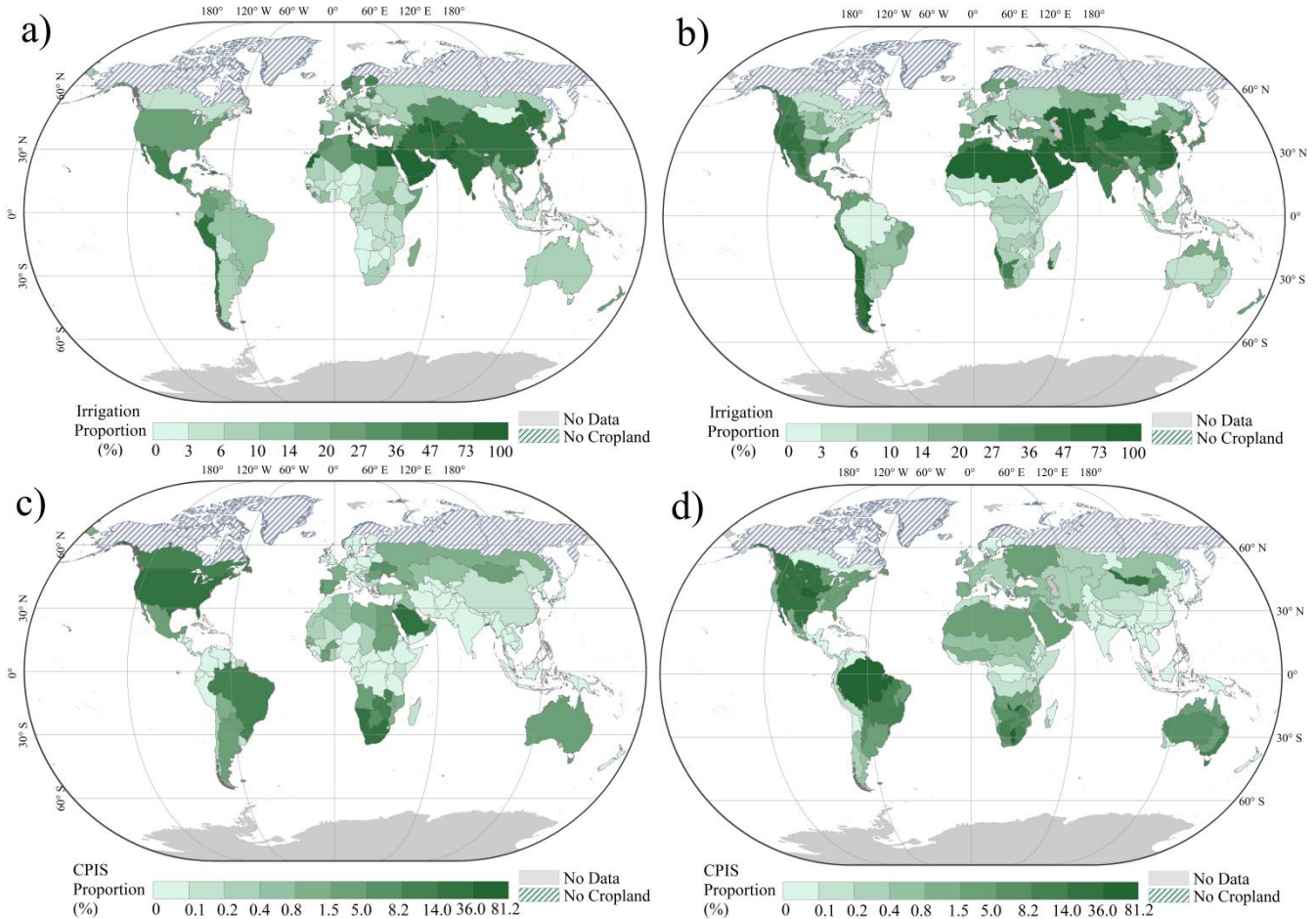
410 Figure 9 The irrigation proportion for each country (a) and IMZ (b) and the CPIS proportion of total irrigated cropland for each country (c) and IMZ (d)
