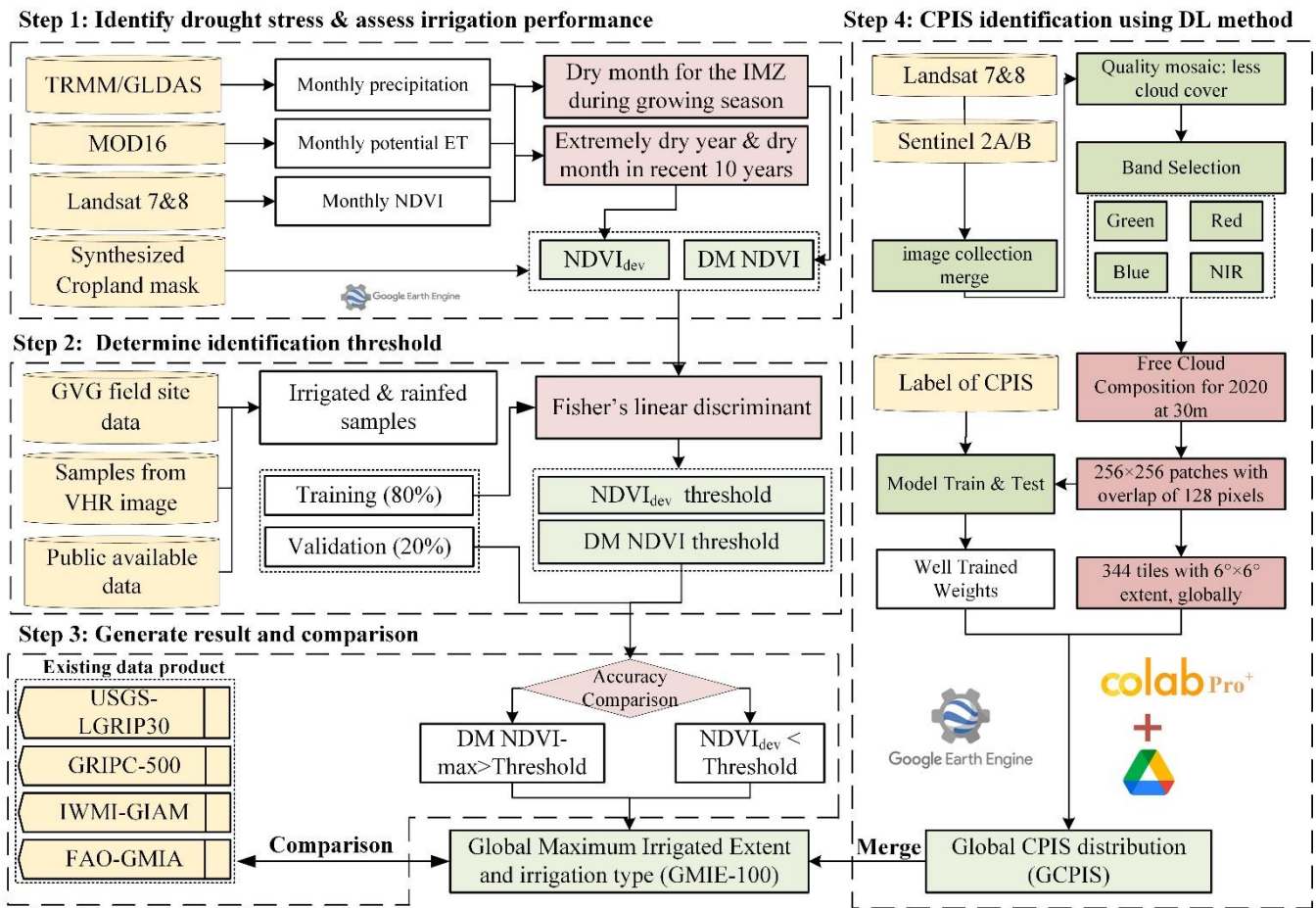
Figure 2 Flow chart of GMIE-100 with a typical irrigation type of CPIS. GVG means GPS, Video, GIS system for collecting field data. VHR means very high resolution. IMZs means Irrigation mapping zones. NDVI dev : NDVI deviation in extremely dry year with 10-year average level. DM-NDVI: NDVI in the dry season.
