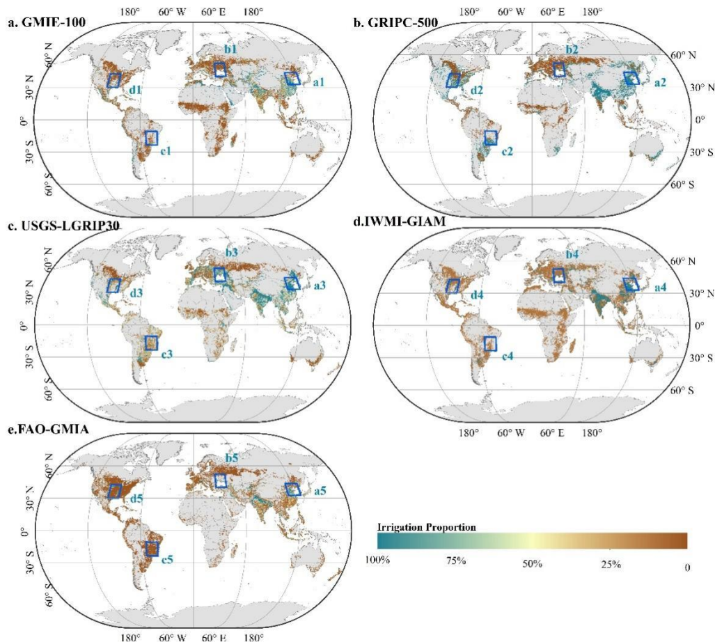
550 Figure 14 Comparison of existing irrigation production at 1 km (GMIE-100, GRIPC-500, USGS-LGRIP30) or 10 km resolution (IWMI-GIAM and FAO-GMIA)
