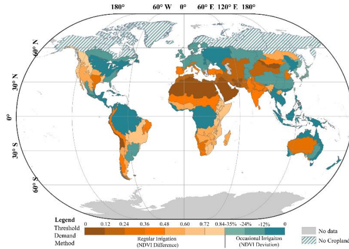
505 Figure 10 The thresholds of the NDVI difference and deviation for each IMZ
