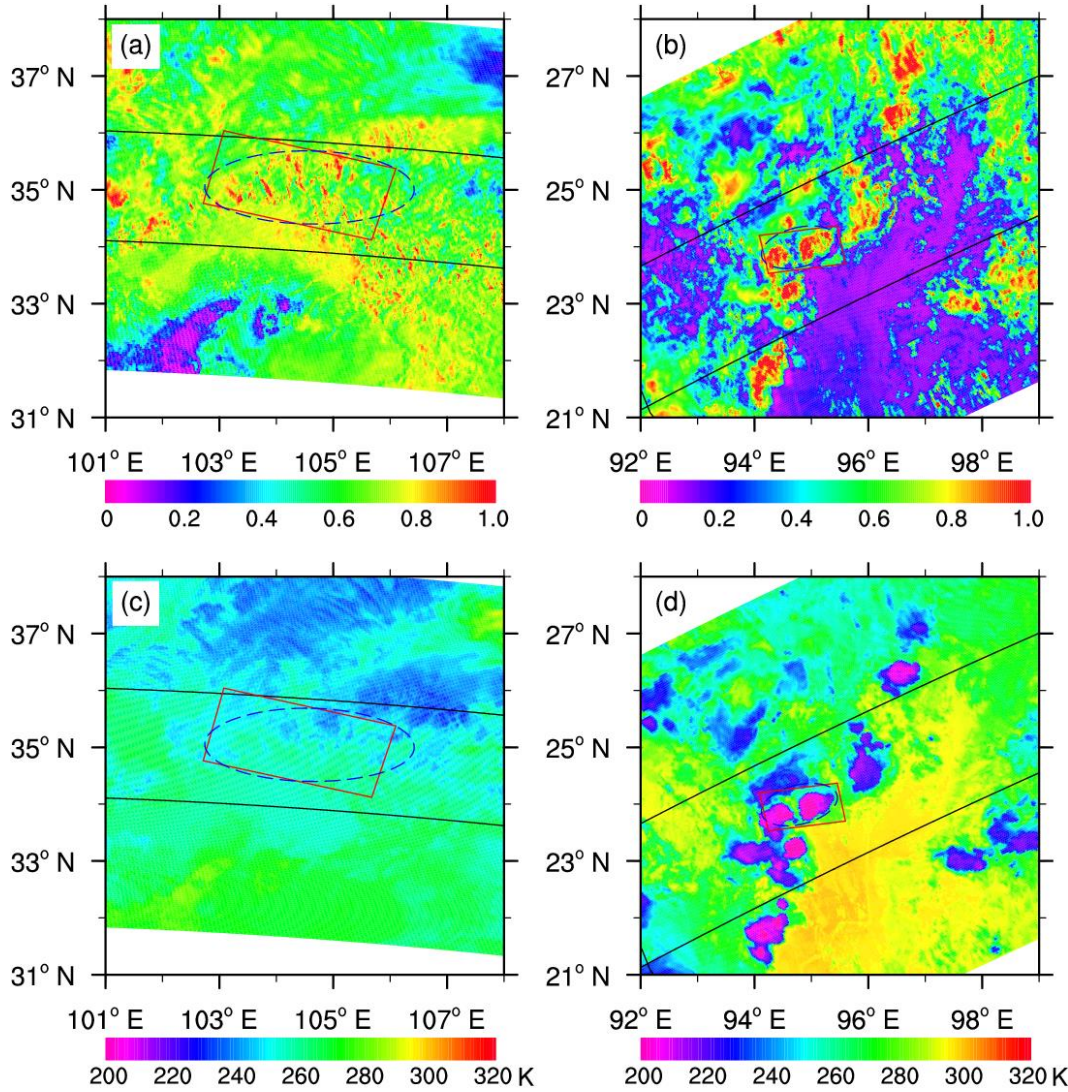
Figure 2. The reflectivity distribution of visible channel at 0.63\ \mu\text{m} (a and b) and brightness temperature distribution of far-infrared channel at 10.8\ \mu\text{m} (c and d) for the two cases observed by VIRS (Visible and Infrared Scanner). The solid black line is PR (Precipitation Radar) scanning track. The red solid rectangle and blue dash ellipse represent for the area of rain cell identified by MBR method and BFE method, respectively.
