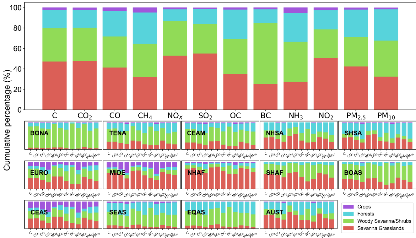
300 Figure 3: Cumulative percentage of annual OBB emissions for each land type in each region during 2020–2022.
