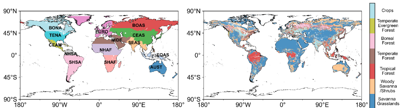
Figure 2 (a) Global geographic regions and its abbreviations. The acronyms on the figure represent the following: BONA: Boreal North America; TENA: Temperate North America; CEAM: Central America; NHSA: Northern Hemisphere South America; SHSA: Southern Hemisphere South America; EURO: Europe; MIDE: Middle East; NHAF: Northern Hemisphere Africa; SHAF: Southern Hemisphere Africa; BOAS: Boreal Asia; CEAS: Central Asia; SEAS: Southeast Asia; EQAS: Equatorial Asia; AUST: Australia and New Zealand; (b) Global land cover type reclassification.
