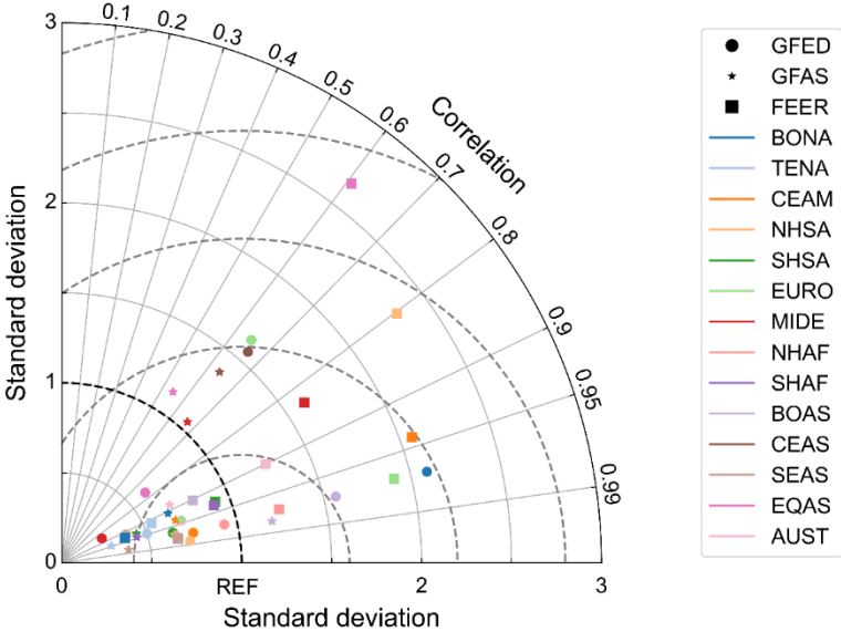
475 Figure 9: Normalized Taylor diagram plot of the comparison between GFED, GFAS, and FEER and this study with monthly OBB carbon emission.
