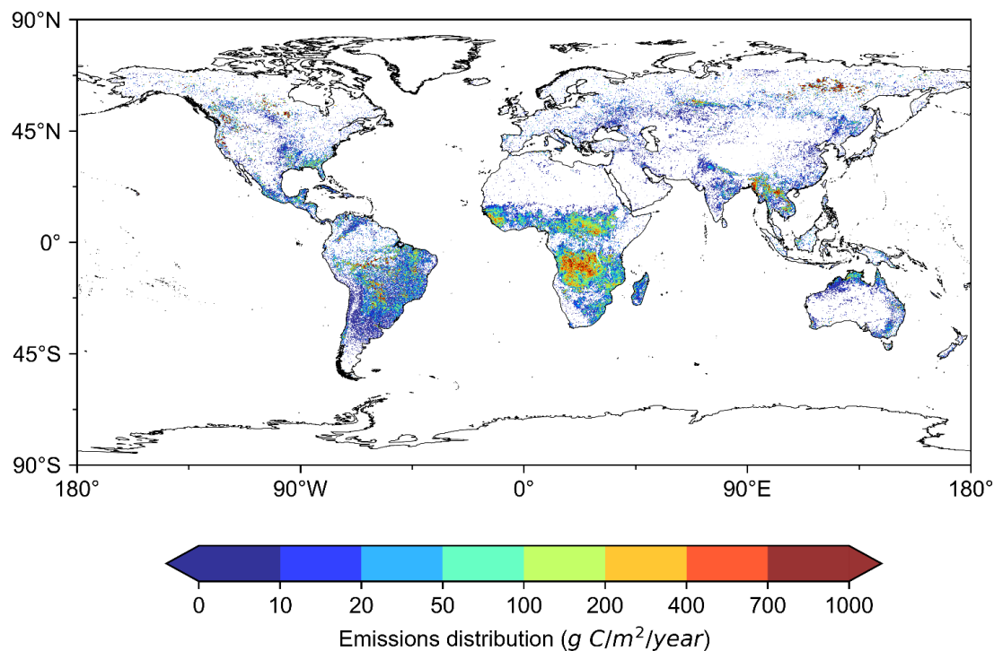
250 Figure 1: Spatial distribution of annual average OBB carbon emissions (1 × 1 km) during 2020–2022.
