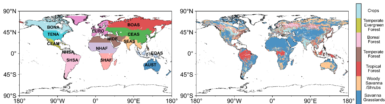
260 Figure 2 (a) Global geographic regions and its abbreviations. The acronyms on the figure represent the following: BONA: Boreal North America; TENA: Temperate North America; CEAM: Central America; NHSA: Northern Hemisphere South America; SHSA: Southern Hemisphere South America; EURO: Europe; MIDE: Middle East; NHAF: Northern Hemisphere Africa; SHAF: Southern Hemisphere Africa; BOAS: Boreal Asia; CEAS: Central Asia; SEAS: Southeast Asia; EQAS: Equatorial Asia; AUST: Australia and New Zealand;(b) Global land cover type reclassification.
