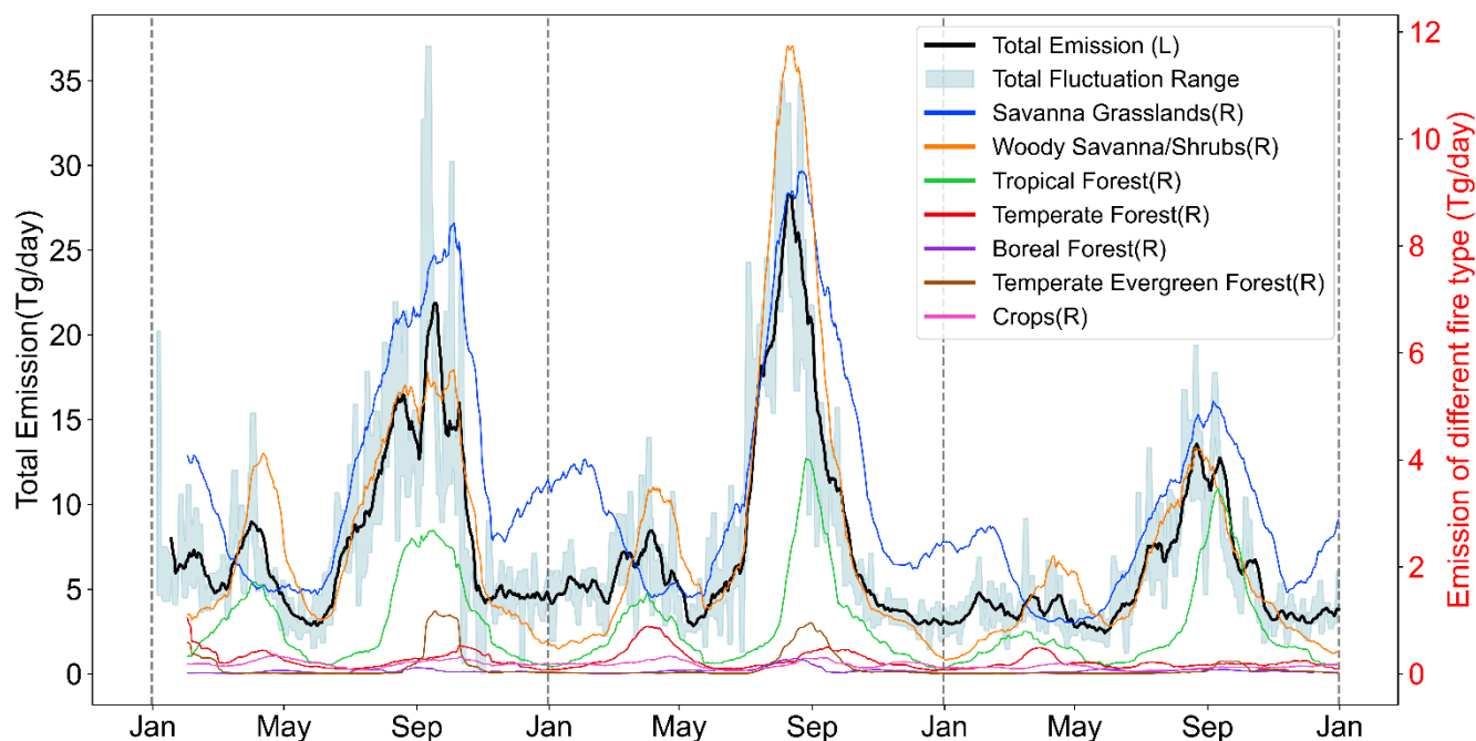
365 Figure 5: Variations in total global OBB carbon emissions and carbon emissions in different fire types across various regions from 2020 to 2022.
