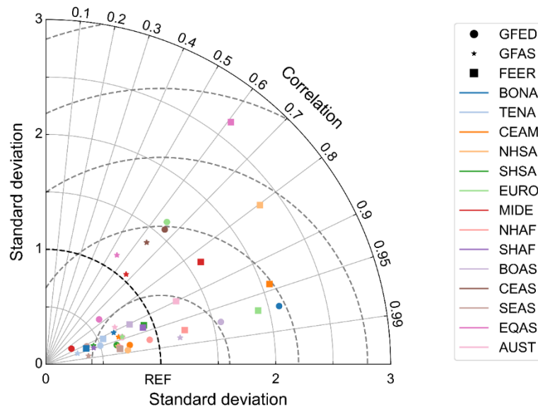
Figure 9: Normalized Taylor diagram plot of the comparison between GFED, GFAS, and FEER and this study with monthly OBB carbon emission.
