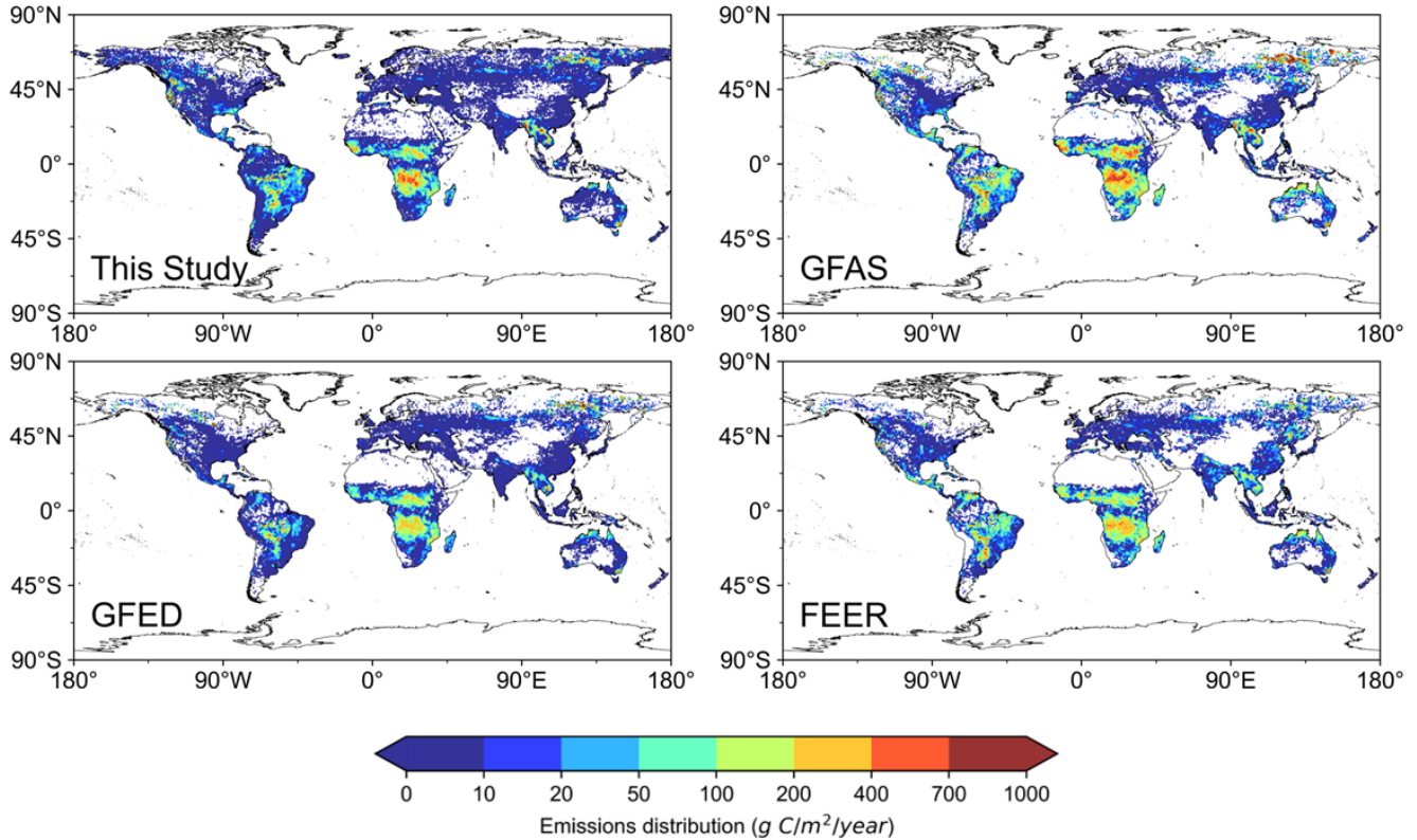
420 Figure 7: Comparison between this study and other emission inventories during 2020–2022 average emissions at 0.5° resolution.
