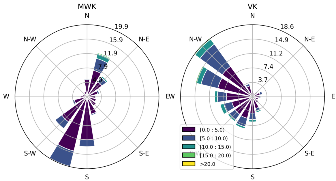
Fig. S4: Wind roses for AWS_MWK and AWS_VK. Colors: Wind speed (m/s). Radial axis: percentage of measurements.
