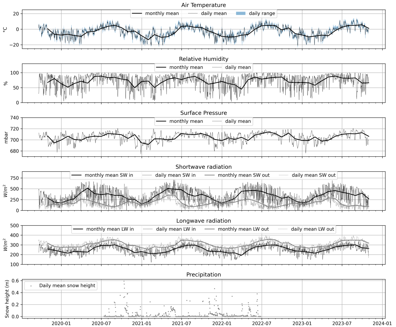
Figure 15. Top panel: Time-series Daily and monthly averages for air temperature, relative humidity, surface air pressure, shortwave and longwave incoming and outgoing radiation, and snow depth for the period of annual-cumulative-positive-degree-day (PDD)-sums-record at AWS_MWK and AWS_VK. Bottom panel: Comparison-Tick marks on the x-axis indicate the start of cumulative PDD for 2021, 2022, 2023.-AWS_MWK the respective months.
