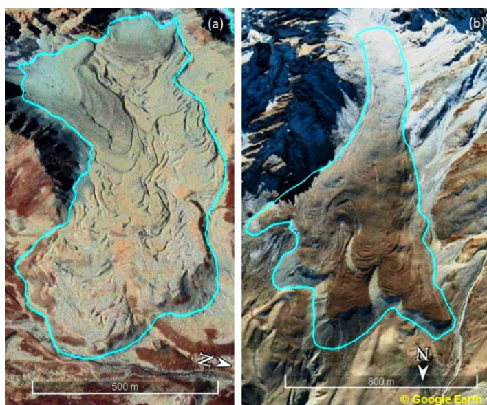
Figure 3. Visual representation of two types of the rock glaciers. (a) Intact rock glacier with RGID-RGU339410N744018E, (b) rock glacier with RGID-RGU351133N763472E.
