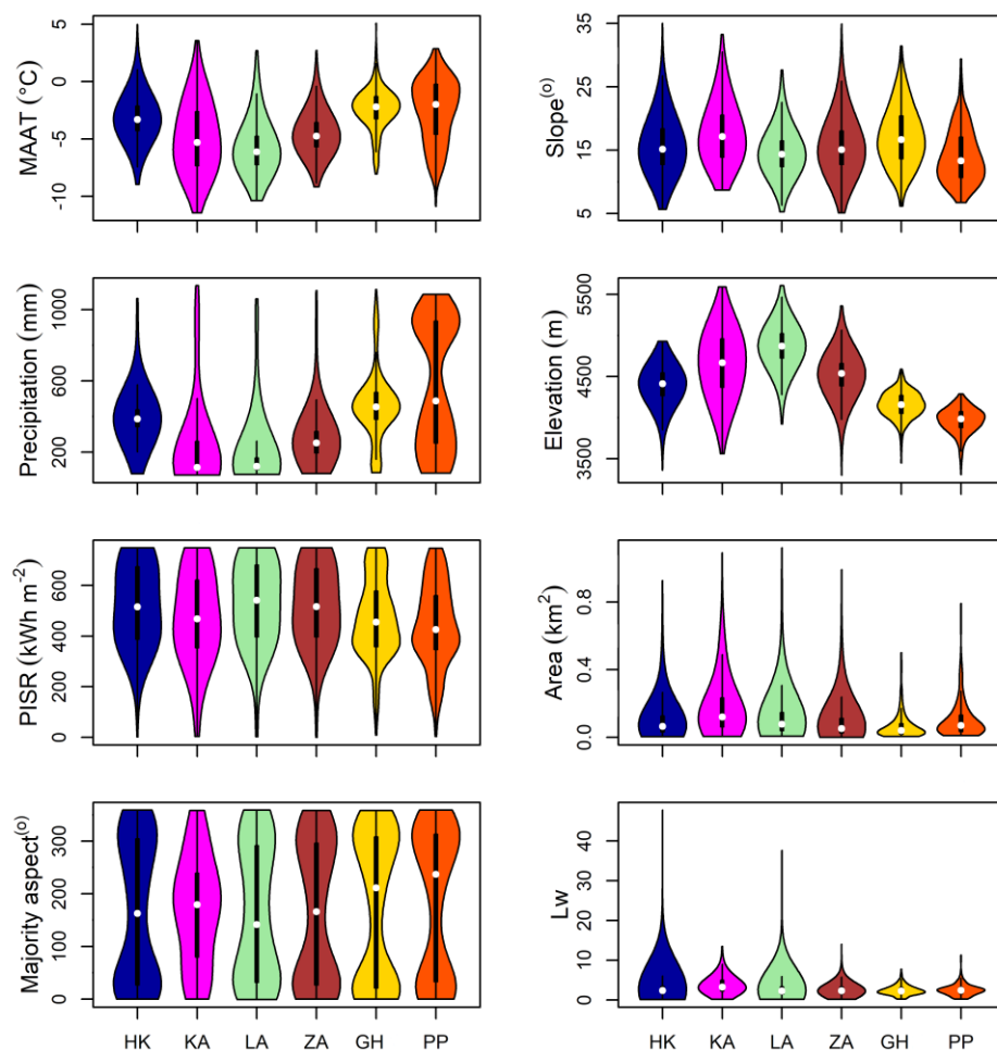
275 Figure 7. Geographic, topographic, and climatic characteristics of the rock glaciers across different mountain ranges in the study area.
