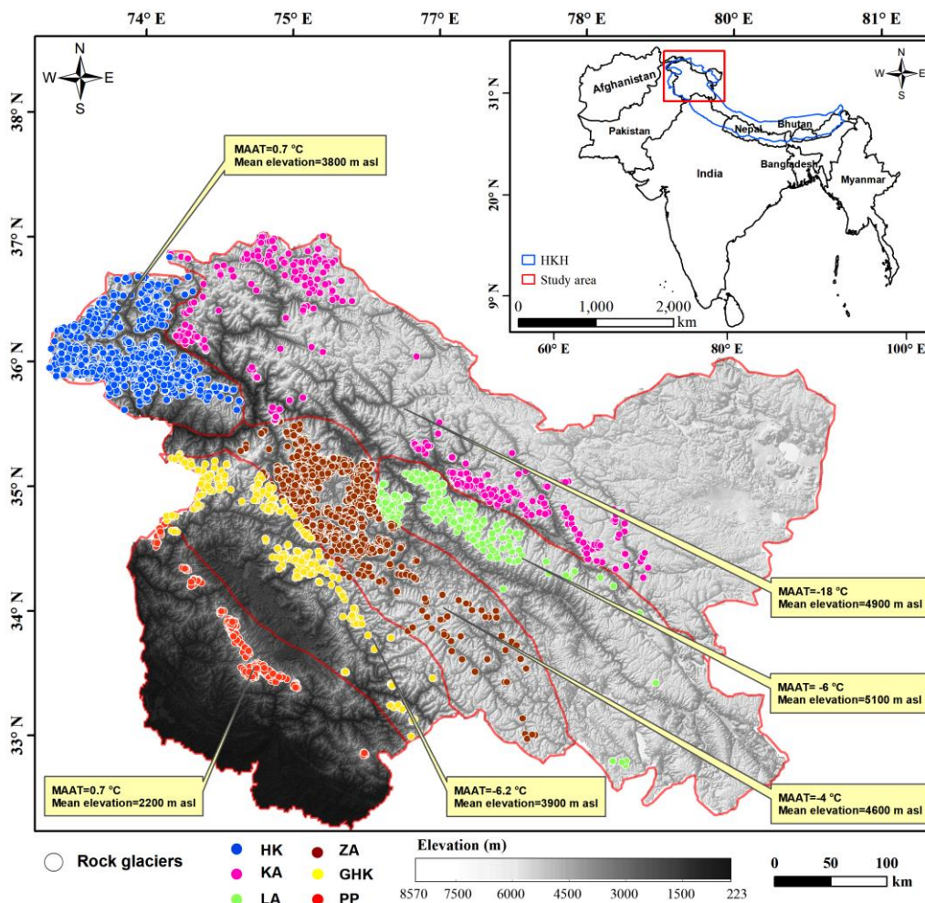
Figure 1. Depicts the study area and emphasizes the different mountain ranges and their climatic and topographic characteristics 95 Hindukush (HK), Karakoram (KA), Ladakh (LA), Zanskar (ZA), Greater Himalaya of Kashmir (GH) and Pir Panjal (PP)
