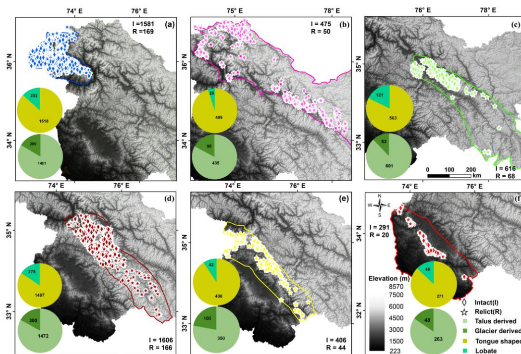
260 Figure 6. Geographical distribution and current status of rock glaciers in various mountain ranges: (a) HK - Hindukush, (b) ZA - Zaskar range, (c) LA - Ladakh range, (d) KA - Karakorum range, (e) GH - Greater Himalaya Kashmir, and (f) PP-Pir Panjal range
