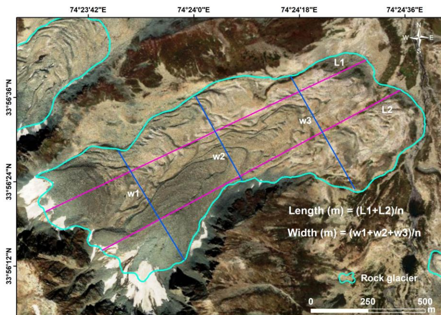
Figure 5. A conceptual representation of computing Lw for each rock glacier in ArcMap 10.1 by considering average measurements of two lengths and three widths. Satellite image credits: ESRI Basemap, ArcMap 10.1.
