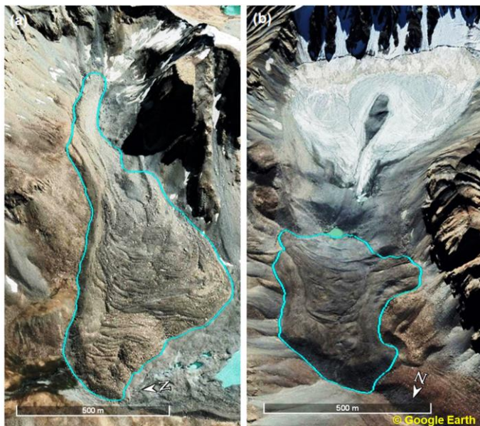
190 Figure 4. Classification of rock glaciers based on source (a) Talus-derived with RGID RGU359030N730756E (b) Glacier-derived with RGID RGU359681N730191E. Satellite image credits: Google Earth.
