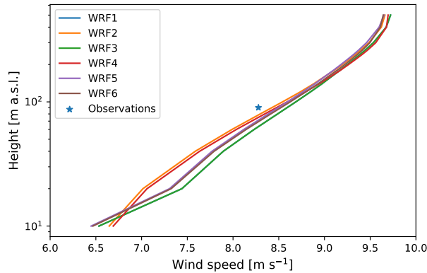
Figure 8. Mean modeled wind speed profiles over from January 1, 2015 to December 31, 2015 from the six WRF model setups considered for the sensitivity analysis, and mean observed winds at 90 m from the DOE Virginia lidar.
