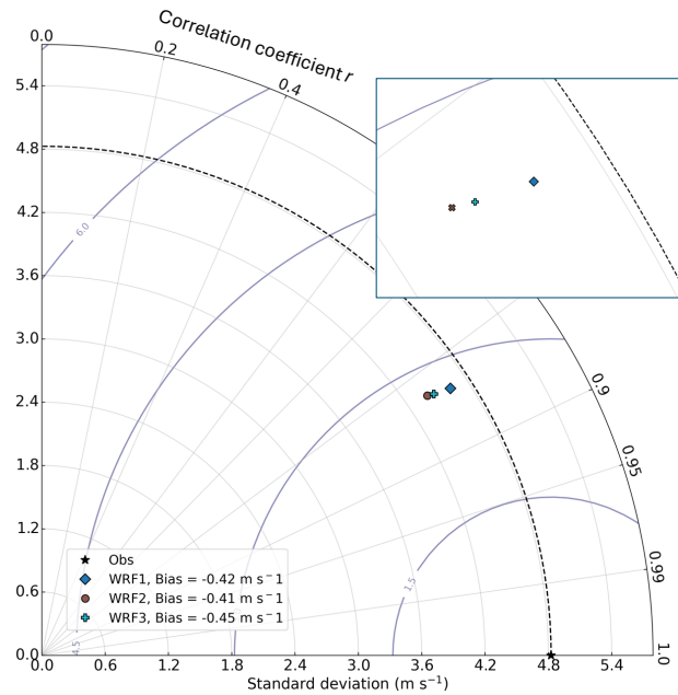
Figure 14. Taylor diagram of the 105 m wind speed from the three WRF model ensemble setups at the location of the Lake Michigan lidar, at 10-minute resolution. Data from May 8, 2012, to December 17, 2012. A zoomed-in inset is also included.
