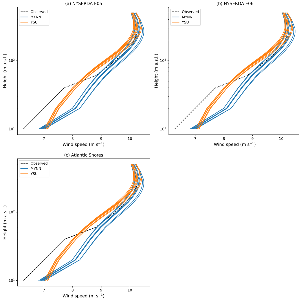
Figure 3. Mean wind speed profiles from the 16 WRF model ensemble members and observed values at the location of the (a) NYSERDA E05 North lidar ( from September 4, 2019 to August 31, 2020 ), (b) NYSERDA E06 South lidar ( from September 4, 2019 to August 31, 2020 ), and (c) Atlantic Shores lidar ( from February 26, 2020 to August 31, 2020 ).
