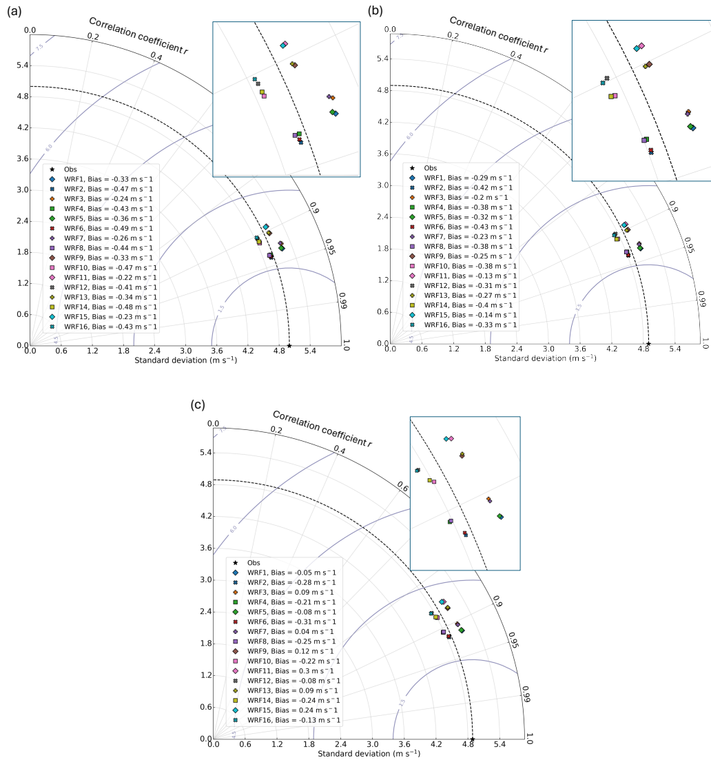
Figure 4. Taylor diagram of the 10-minute REWS from the 16 WRF model ensemble setups at the location of the (a) NYSEERDA E05 North lidar ( from September 4, 2019 to August 31, 2020 ), (b) NYSEERDA E06 South lidar ( from September 4, 2019 to August 31, 2020 ), and (c) Atlantic Shores lidar ( from February 26, 2020 to August 31, 2020 ). For each diagram, a zoomed-in inset is also included.
