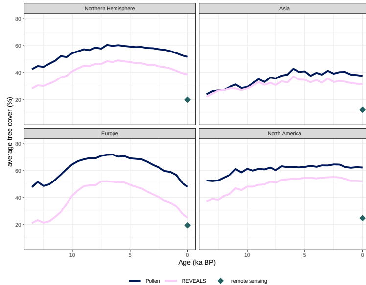
Figure 5. Northern Hemisphere and continental mean tree pollen percentage and mean REVEALS tree cover for 2^{\circ} \times 2^{\circ} grid cells through the Holocene. (Northern Hemisphere and continental averages from different grid cell resolutions are available in S3: Reconstruction results for different spatial resolutions). Remotely sensed average forest cover for the grid cells with valid pollen coverage (at least one large lake or multiple other basins present in the time slice) is indicated with the diamond. Temporal trends are the same, but absolute tree cover is reduced in the REVEALS reconstructions compared to the original pollen data. Both pollen percentages and REVEALS estimates still overestimate tree cover.
