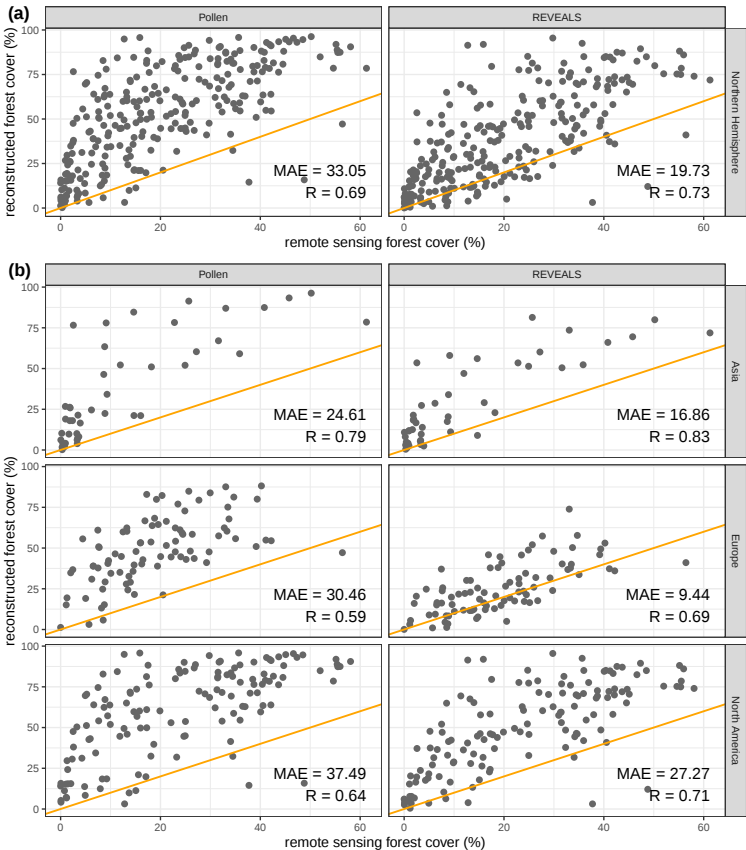
Figure 9. Remote sensing forest cover (LANDSAT) and modern reconstructed forest cover from Pollen and REVEALS with original RPP values , and REVEALS ( < 100 years BP ) in 2x2° grid cells with optimized RPP values globally mean absolute errors (a)MAE and for all continents correlation coefficient (b)R per group . Reconstructed forest cover from the original pollen data tends to overestimate observed (remote sensing) forest cover. This is improved Improvements with the REVEALS run using original RPP values and even more so reconstruction are especially high in Europe . Validations with different grid cell sizes are available in the REVEALS run using optimized RPP values supplement (S3: Validation results for different spatial resolutions) .
