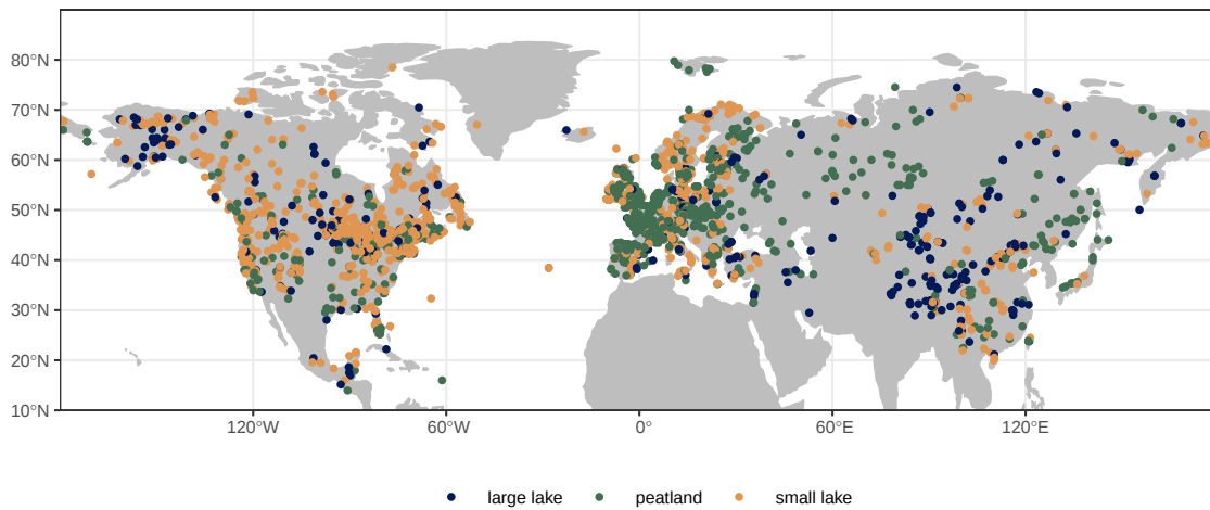
Figure 1. Pollen record locations in the LegacyVegetation dataset. Colors indicate record type (large lake > 50 ha). Record density is highest in Europe and Eastern North America, and lowest in Africa-Northern and Australia and Oceania Central Asia .
