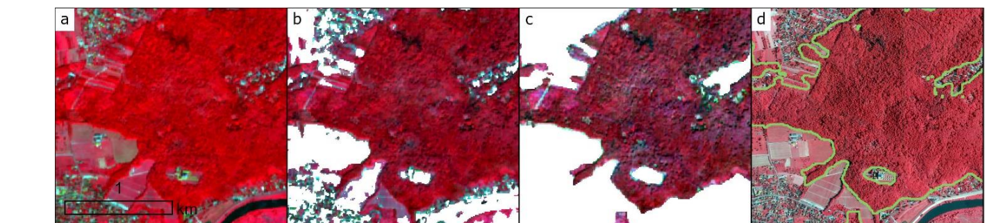
175 Figure 4 Procedure for obtaining forest mask used in this study on the example of part of Kraków, southern Poland: a) Sentinel-2 image (NIR, VIS R, VIS G); b) Sentinel-2 clipped to ESA World Cover v200 dataset extracted tree cover class; 3) Sentinel-2 clipped to ESA World Cover, Dynamic World and NDVI thresholding; 4) high resolution CIR orthoimage with borders of the calculated forest mask.
