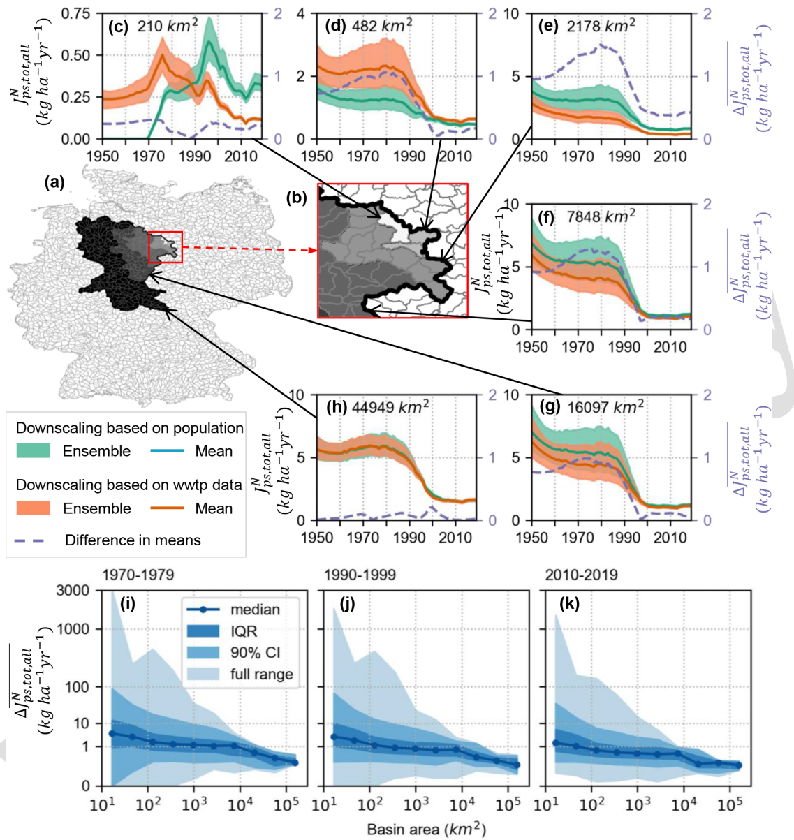
Figure 9. N point sources ( J_{ps,tot,all}^N in kg ha -1 yr -1 ) and absolute differences in the mean of the posterior ensemble between the two downscaling approaches based on population and WWTP data ( \Delta J_{ps,tot,all}^N in kg ha -1 yr -1 ), aggregated at basins level for river basins of the HydroSHEDS database. Panels (a)–(b) report the map of the 3778 basins selected over Germany, including six exemplary nested sub-basins of the Weser River basin reported in grey-shaded areas. Panels (c)–(h) represent the N point sources for the six sub-basins of the Weser River basin. The light-green-shaded and red-shaded areas delineate the minimum and maximum values over the 100 posterior realisations for the downscaling approach for the treated component based on population and WWTP data, respectively. The solid dark-green and red lines represent the mean of the posterior realisations, and the absolute difference between these two means is shown as dashed purple lines (secondary y axis). Panels (i)–(k) report the distribution (median, interquartile range (IQR), 90 % confidence interval (CI), and full range) of the difference in the means ( \Delta J_{ps,tot,all}^N ) against the basin area, which is grouped into 10 classes. The class centres are reported as dark-blue circles along the median line. Distributions are shown for the decades 1970–1979 (i), 1990–1999 (j), and 2010–2019 (k). This figure is distributed under a CC BY-NC-SA 4.0 licence. Data source: basin boundaries come from the HydroBASINS v1.c of the HydroSHEDS database (HydroSHEDS, 2014; Lehner and Grill, 2013) © HydroSHEDS. The map is shown in the WGS84 system in the figure. © Authors 2024.
