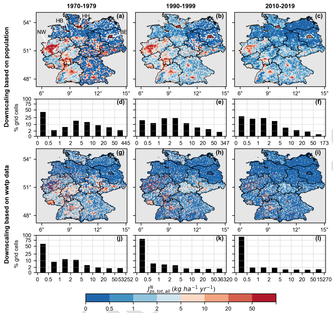
Figure 8. Gridded maps of total N point sources J_{ps,tot,all}^N in \text{kg ha}^{-1} \text{yr}^{-1} ; (a–c and g–i), including both the treated and untreated components, and distribution of the grid cell values of J_{ps,tot,all}^N (d–f and j–l), obtained by downscaling the mean of the posterior realisations from NUTS-1 to grid level using population data (a–f) and WWTP data for the treated component (g–i). The untreated component is always downscaled based on population data. The figure provides the average values in our posterior ensemble over three different decades: 1970–1979 (left panels), 1990–1999 (middle panels), and 2010–2019 (right panels). Panels (a)–(c) show the data at a resolution of 0.015625^\circ , while panels (g)–(i) report aggregated values at a resolution of 0.0625^\circ for depiction purpose (the maps at 0.015625^\circ resolution are reported in Fig S63). Panels (d)–(f) and (j)–(l) all refer to the distribution of the grid cells values at 0.015625^\circ resolution. In all panels, the values of J_{ps,tot,all}^N were grouped into the same eight classes. The last class of values (depicted in dark-red colour in the maps) includes all values higher than 50 \text{ kg ha}^{-1} \text{yr}^{-1} . The figure also reports the boundaries of the 16 NUTS-1 units of Germany and indicates the location of the city states, that is Berlin (BE), Bremen (HB), Hamburg (HH), and North Rhine-Westphalia (NW). P point sources are shown in the Supplement, Fig. S62. Data source: the NUTS-1 map comes from the German Federal Agency for Cartography and Geodesy (BKG, 2020) © GeoBasis-DE/BKG dl-de/by-2-0 licence ( https://www.govdata.de/dl-de/by-2-0 , last access: 21 September 2024). The map is shown in the WGS84 system in the figure. © Authors 2024. This figure is distributed under a CC BY-NC-SA 4.0 licence.
