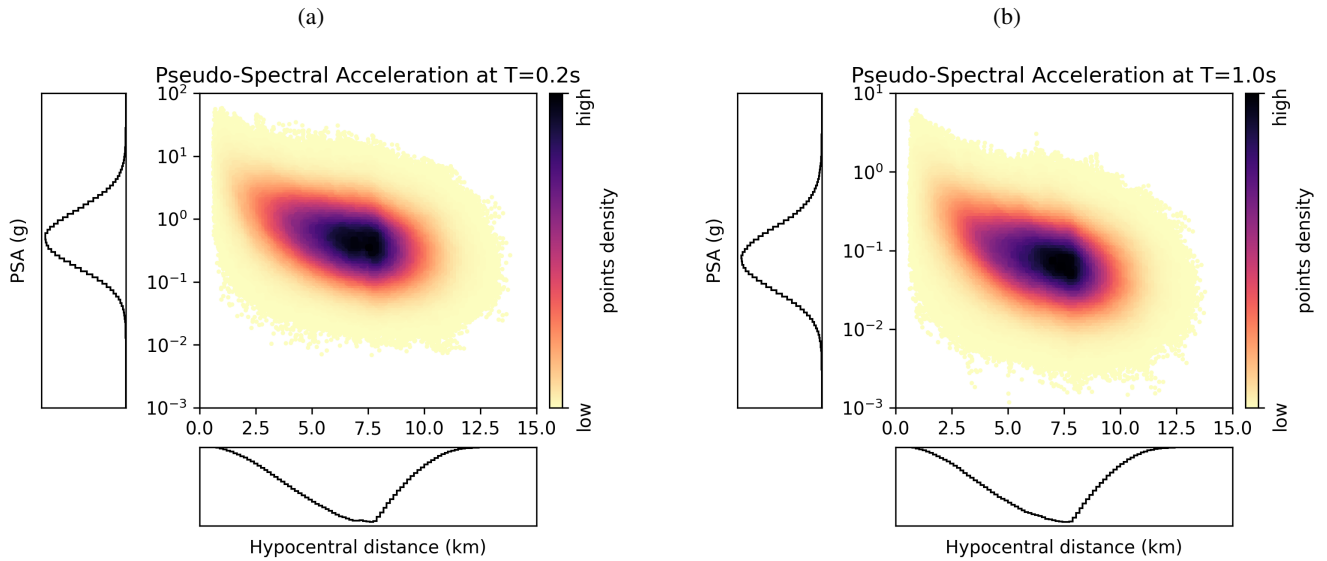
Figure 7. For each sample and each sensor, the Pseudo-Spectral Acceleration is shown against the hypocentral distance at period T=0.2 s (a) and T=1.0 s (b). The PSA is computed on the East-West component, results are very similar for the two other components.
