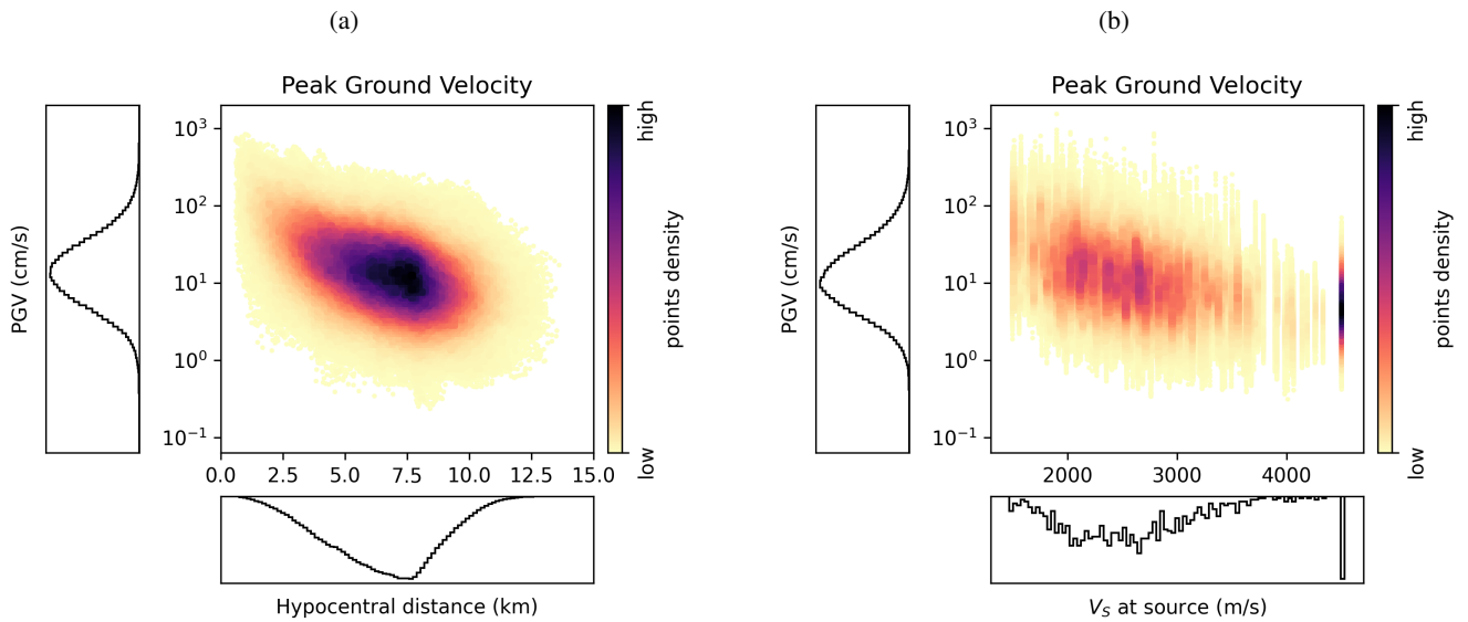
Figure 5. The Peak Ground Velocity (PGV) is computed as the the maximum absolute value over all timesteps separately on each component. There is one value for each of the 32 \times 32 sensors and each of the 30000 samples.
