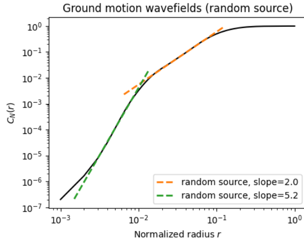
(c) Correlation dimension for 30000 ground motion wavefields with a random source (HEMEW S database)
