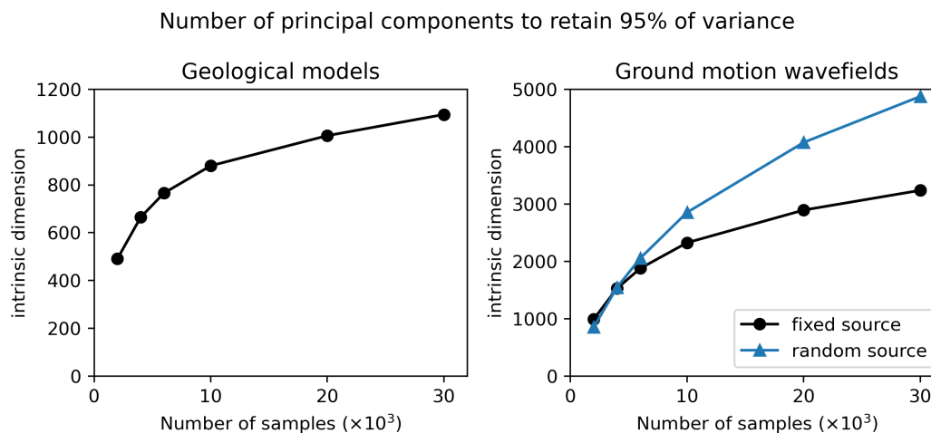
Figure B1. Number of principal components ( y -axis) required to represent 95% of the variance in data as a function of the dataset size ( x -axis) for geological models (left) and ground motion wavefields (right). For ground motion, the HEMEW-3D database is used for the fixed source (black line) and the HEMEW S database corresponds to the blue line.
