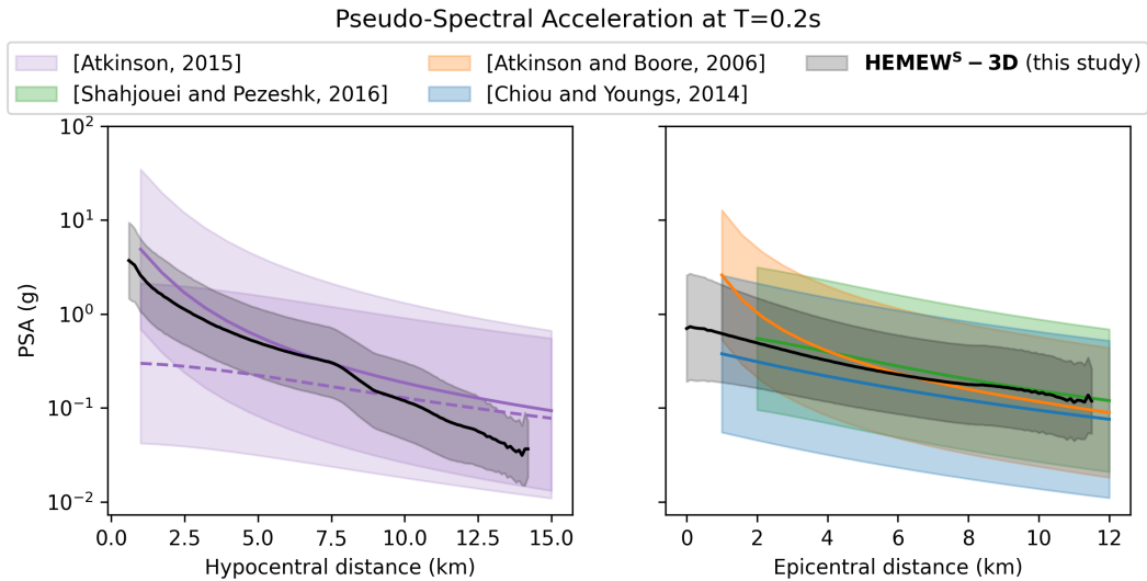
Figure 8. Horizontal PSA at period T=0.2s as a function of hypocentral distance (left) and epicentral distance (right) for GMMs by Atkinson (2015) with a depth of 1 km (purple solid line, left), Atkinson (2015) with a depth of 7.5 km (purple dashed line, left), Atkinson and Boore (2006) (orange, right), Chiou and Youngs (2014) (blue, right), Shahjouei and Pezeshk (2016) (green, right), and our HEMEW S -3D database (black). Solid lines correspond to the mean PSA and shaded areas to one standard deviation. Horizontal PSA is computed as the geometrical mean of East-West and North-South components.
