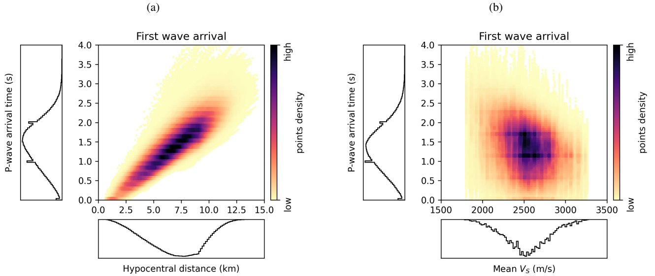
Figure 4. For each sample and each sensor, the P-wave arrival time is shown against (a) the hypocentral distance, (b) the mean S-wave velocity in the 3D domain.
