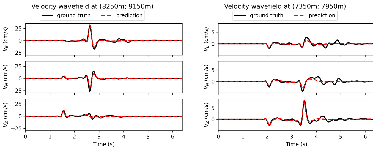
Figure 10. For two spatial points, the velocity field predicted by the MIFNO (red dashed line) is compared with the reference from the HEMEW S -3D database (black line).
