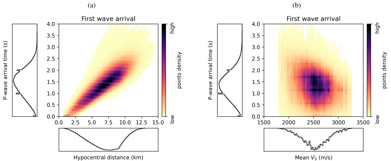
Figure 4. For each sample and each sensor, the P-wave arrival time is shown against (a) the hypocentral distance, (b) the mean S-wave velocity in the 3D domain.
