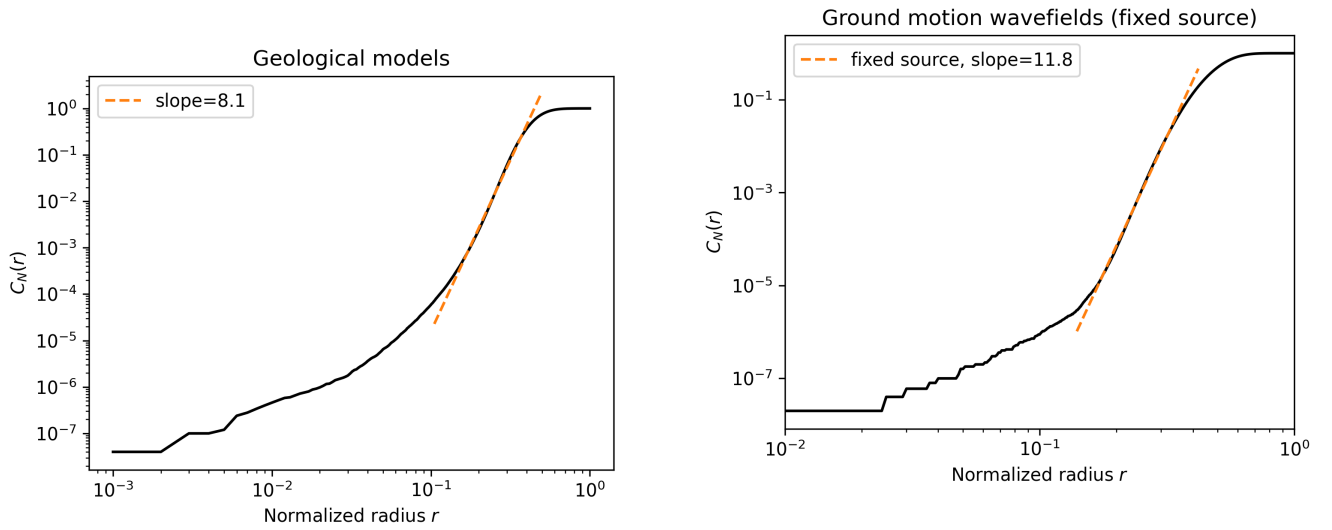
(b) Correlation dimension for 30000 ground motion wavefields with a fixed source (HEMEW-3D database)
