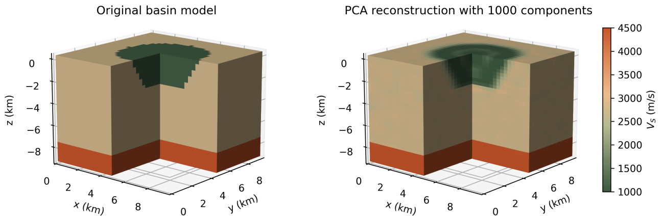
Figure 9. The original geological model (left) contains two homogeneous layers and a circular basin inserted inside the top layer. The PCA reconstruction was obtained with 1000 PCA components (right).
