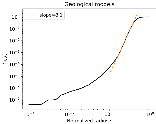
(a) Correlation dimension for 30000 geological models
