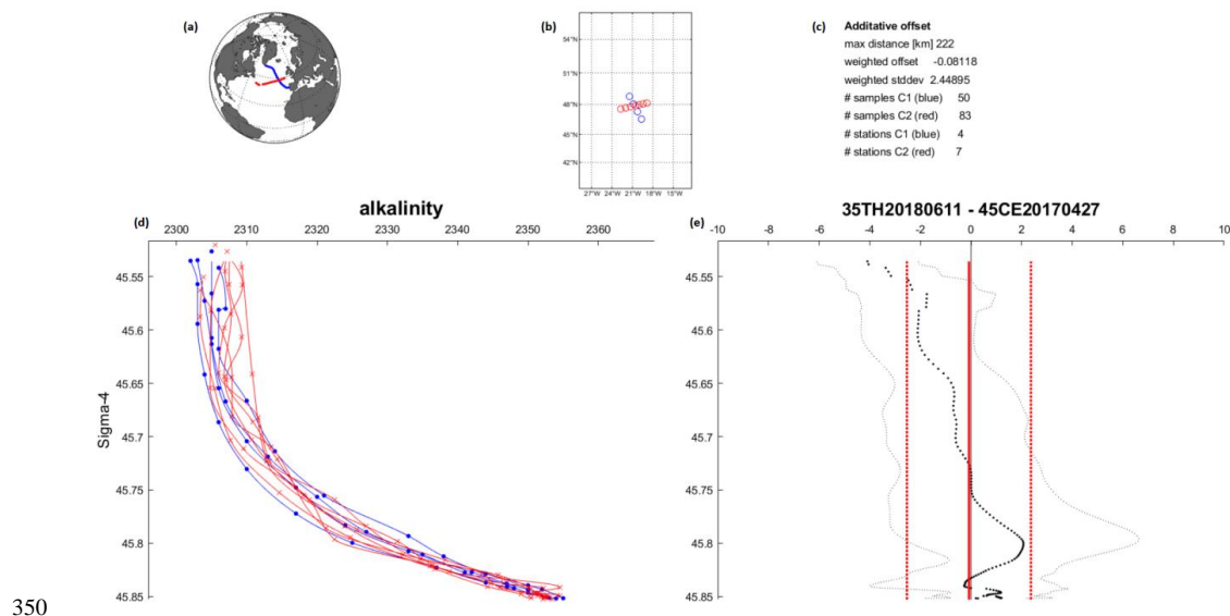
Figure 3. Example crossover figure for alkalinity for cruises 35TH20180611 (blue) and 45CE20170427 (red), as was generated during the crossover analysis. Panel (a) shows all station positions for the two cruises, and (b) shows the specific stations used for the crossover analysis. Panel (d) shows the data of alkalinity ( \mu\text{mol kg}^{-1} ) below the upper depth limit (in this case 2000 dbar) versus potential density anomaly referenced to 4000 dbar as points and the interpolated profiles as lines. Non-interpolated data either did not meet minimum depth separation requirements (Table 4 in Key et al., 2010) or are the deepest sampling depth. The interpolation does not extrapolate. Panel (e) shows the mean alkalinity difference profile (black, dots) with its standard deviation, as well as also the weighted mean offset (straight red lines) and weighted standard deviation. Summary statistics are provided in (c).
