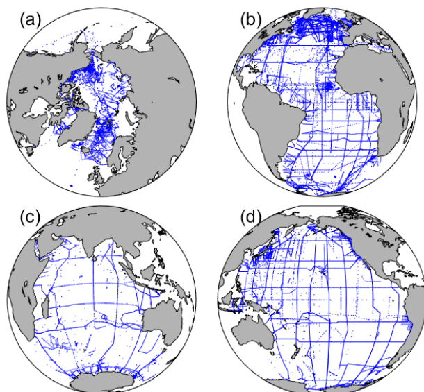
590 Figure 9. Locations of stations included in the (a) Arctic, (b) Atlantic, (c) Indian, and (d) Pacific ocean product files for the complete GLODAPv2.2023 dataset.
