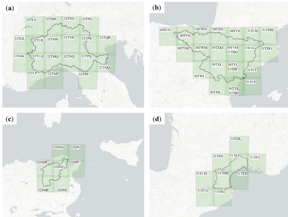
Fig. B4C1: Spatial coverage of Sentinel-2 tiles together with their overlapping areas for (a) Po, (b) Ebro, (c) Medjerda, (d) Hérault basins. Each tile (in green) contains respective identification number corresponding to Sentinel-2 tiling system as explained at https://sentinels.copernicus.eu/web/sentinel/missions/sentinel-2/data-products .
