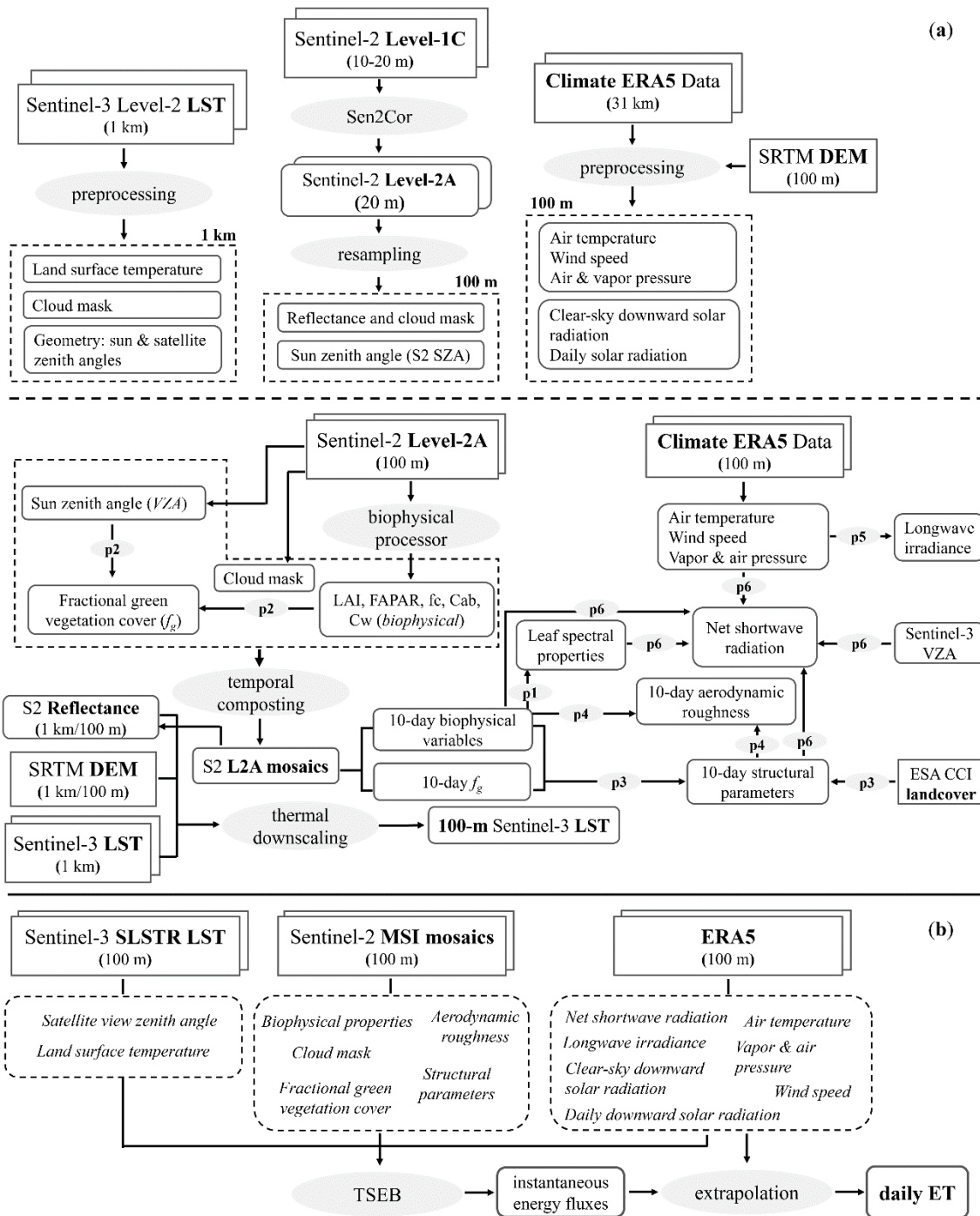
Figure 2: Schematic flowchart of the entire ET processing including (a) source data preprocessing (the top row) and input retrievals for the Priestley-Taylor Two-Source Energy Balance (TSEB)-modeling (the lower line), (b) daily ET estimation at 100 m resolution. While processes are represented by ovals (e.g., preprocessing, thermal downscaling, TSEB-PT modeling, and intermediate p1-p6), rectangles stand for source parameters, and round rectangles indicate intermediate and final results.
