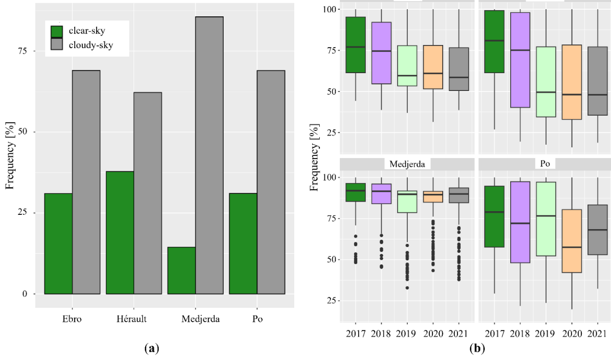
580 Figure 5: General overview on the sky conditions for the final ET mosaics over each basin (EB, HB, MB, PB) considering: (a) clear and overcast conditions at Sentinel-3 and Sentinel-2 overpass time for the period 2017-2021, (b) the distribution of cloudy-sky conditions for each separate year. Note that non-vegetated surfaces are excluded from this analysis. In order to minimize other disturbing factors such as a seasonal snow cover, our time of interest covers the period during growing season.
