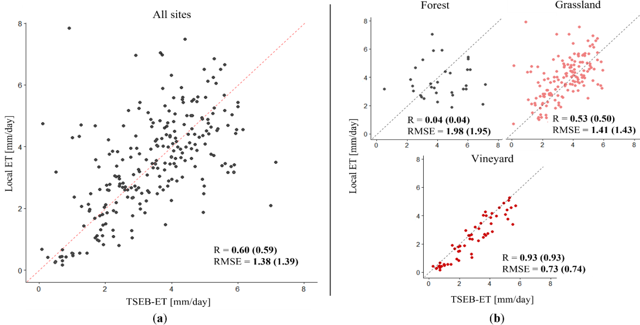
460 Figure 3: Scatterplots between ground-derived ET observations and TSEB-PT-ET simulations for: (a) all Eddy Covariance sites included, (b) separated landcovers: forest grassland, and vineyard. Note that values in brackets indicate accuracy statistics obtained within 50-m buffer, while records without parentheses represent pixelwise validation strategy.
