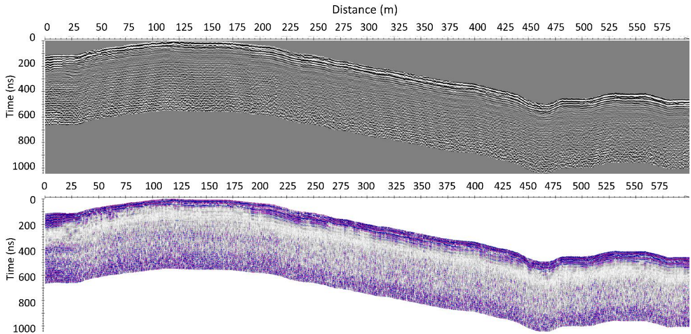
500 Figure 11: Example of a processed 2D radargram for GPR_long_40 MHz radargram. The radargram is shown in two different color scales.
