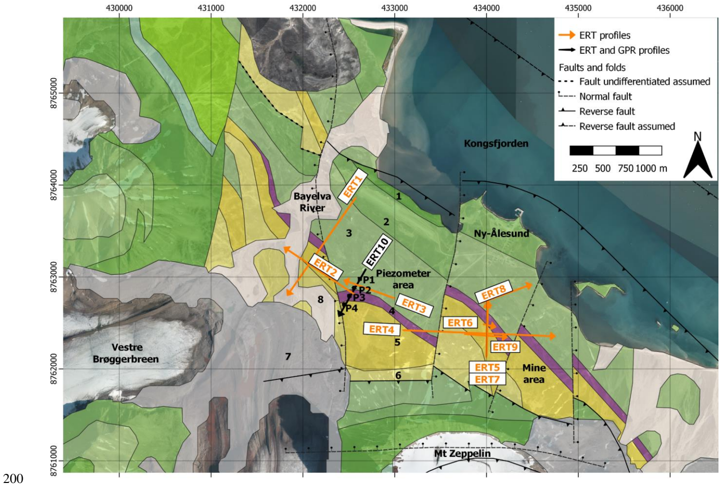
Figure 2: Geological map (data from NPI, WMS geological map at 1:250.000): 1) Carbonate rocks of Wordiekammen Formation (Moscovian-Sakmarian); 2) Carbonate rocks of Gipshuken Formation (Sakmarian - Artinskian); 3) Chert, shale, sandstone and limestone of Kapp Starostin Formation (late Artinskian - Late Permian); 4) Shale, siltstone, sandstone of Vardebukta Formation (Induan); 5) Sandstone, shale, coal of Kongsfjorden Formation (paleocene ?); 6) Sandstone, shale, conglomerate of Brøggerbreen Formation (Paleocene?); 7) Moraine (Holocene); 8) Glacio-fluvial deposits (Holocene); NF) Normal fault; RF) Reverse fault. The coordinate system is WGS84-UTM33N. The geological map was exported from the WebGIS tool by ©Norwegian Polar Institute ( https://geokart.npolar.no/Html5Viewer/index.html?viewer=Svalbardkartet ).
