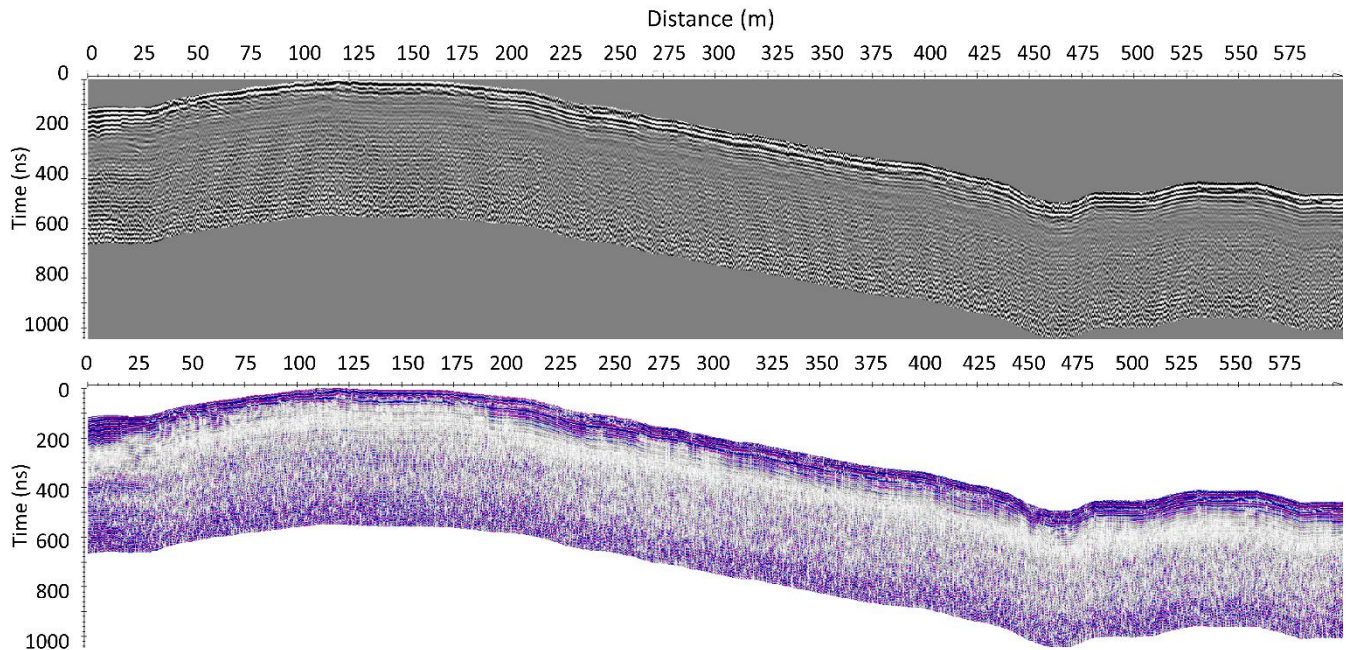
495 Figure 11: Example of a processed 2D radargram for GPR_long_40 MHz radargram. The radargram is shown in two different color scales.
