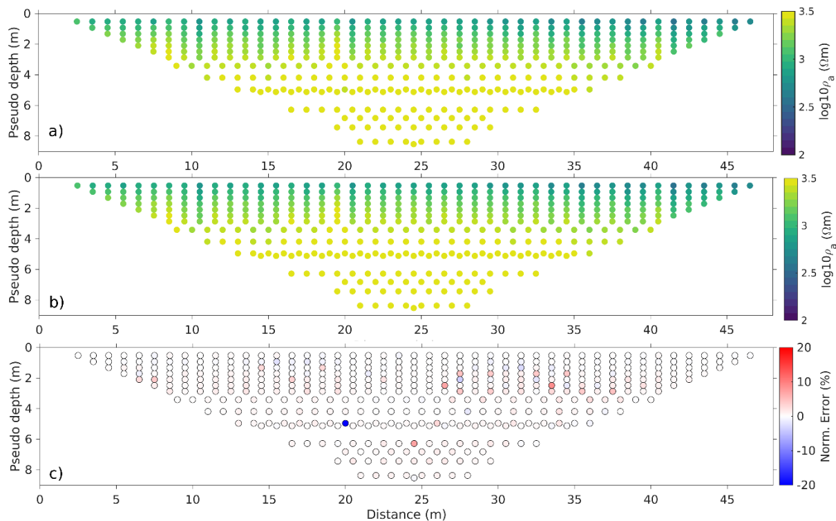
Figure 9: Post-processing analysis of the ResIPy inversion result for ERT_P1_Par, WS configuration: a) observed data ( \rho_a ); b) calculated response ( \rho_a ); c) misfit between them, calculated as normalized error in percentage.
