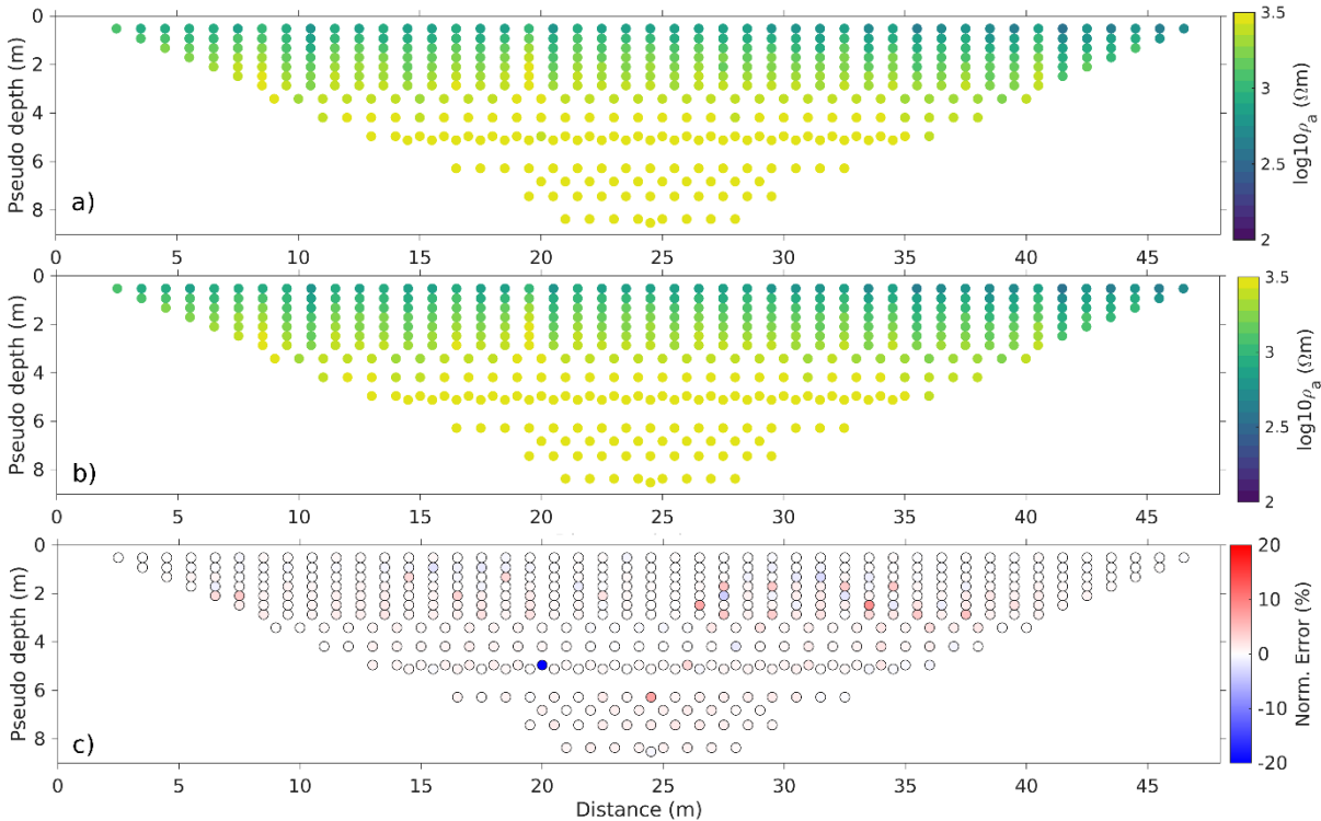
480 Figure 9: Post-processing analysis of the ResIPy inversion result for ERT_P1_Par, WS configuration: a) observed data ( \rho_a ); b) calculated response ( \rho_a ); c) misfit between them, calculated as normalized error in percentage.
