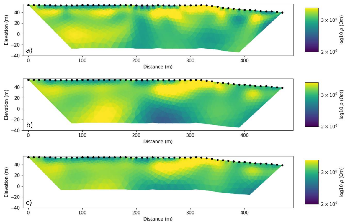
Figure 7: Resistivity model obtained from the inversion of ERT9. Different acquisition configurations: a) DD; b) WS; c) WE. The minimum and maximum boundaries of the color bar are 100 and 3000 Ωm, respectively.
