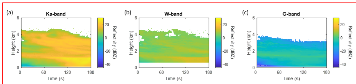
160 Figure 4: Example of CloudCube data on March 30, starting time 17:12:52 UTC, showing calibrated reflectivity at Ka (a), W (b) and G-band (c). The W-band plot (b) shows no data for approximately the first 500 m, corresponding to the blind range of the radar.
