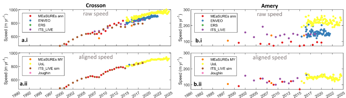
Figure C2. Velocity alignment example two. Panels (a.i) and (b.i) show the raw speed from a single pixel on our most seaward flux gate. Panels (a.ii) and (b.ii) show the final aligned speed.
