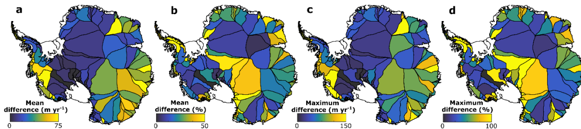
Figure C3. Velocity alignment overview. Each panel shows the differences between all velocity data sources in all flux gate pixels in each MEaSUREs glacier basin. The individual data sources are as described in the main text. Differences between velocity data sources are calculated in 1-year moving windows prior to alignment and averaged through time in each flux gate pixel, prior to calculating basin-scale statistics. (a) The mean velocity difference, in meters per year. (b) The mean difference as a percentage of the basin- and time-averaged post-aligned speed. (c) The maximum time-averaged difference. (d) As for panel (c), as a percentage of the basin- and time-averaged post-aligned speed.
