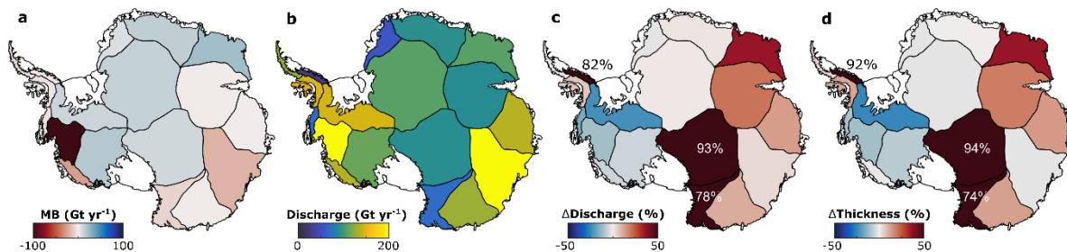
Figure A2. Creating BM+HF14 Adj . (a) Observed rate of mass change from 1996 to 2021 based on the observed rates of ice surface elevation change in Figure A1. (b) Grounding line discharge, within each MEaSUREs regional basin, implied by the observed rates of mass change, given the surface mass balance from the mean of three regional climate models (described in text). (c) The percentage difference between the discharge in panel (b) and our average 1996-2021 discharge derived from BM+HF14. (d) The change in BM+HF14 thickness required at the most downstream flux gate in order to reproduce panel (b).
