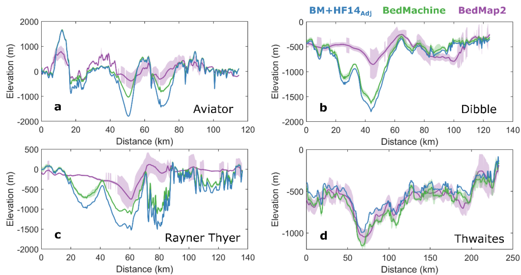
Figure A3. Bed elevation profiles. Each panel shows bed elevation in BedMachine v3 (green), BedMap2 (magenta) and BM+HF14 Adj at our most seaward flux gate (blue) in example basins.
