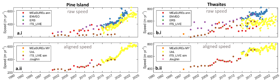
Figure C1. Velocity alignment example one. Panels (a.i) and (b.i) show the raw speed from a single pixel on our most seaward flux gate. Panels (a.ii) and (b.ii) show the final aligned speed.
