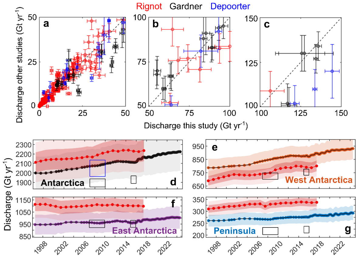
Figure 13. Comparison to existing grounding line discharge estimates. Panels (a) to (c) show comparisons with Rignot et al. (2019), Gardner et al. (2018) and Depoorter et al. (2013) for equivalent basins and during overlapping time-periods. Each point shows the discharge for a single basin, with errors provided where available. Panels (d) to (g) show time-series of our primary discharge estimate (using BM+HF14) compared to other estimates – data from Rignot et al. (2019) are shown as red dots, with dark shading indicating 5 % uncertainty and pale shading indicating 10 % uncertainty. The black boxes in panels (d) to (g) show data from Gardner et al. (2018) and the blue box in panel (d) shows data from Depoorter et al. (2013).
