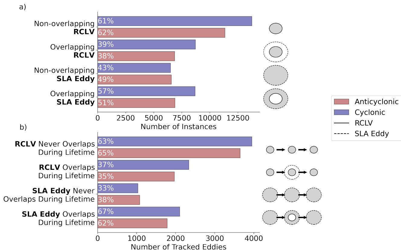
Figure 4. (a) The number of eddy contours that are concurrent (“overlapping”) and not concurrent (“non-overlapping”) with contours in the other atlas. The percentages of eddies exhibiting the given characteristic compared to the total number of eddies of each polarity are overlaid in white. For overlapping eddies, the numbers are the same since this is a mutual metric, but the percentages of the total eddy counts differ. The schematics on the right-hand side show the referenced feature in gray. (b) The number of eddies that overlap and never overlap throughout the lifetimes of the tracked features.
