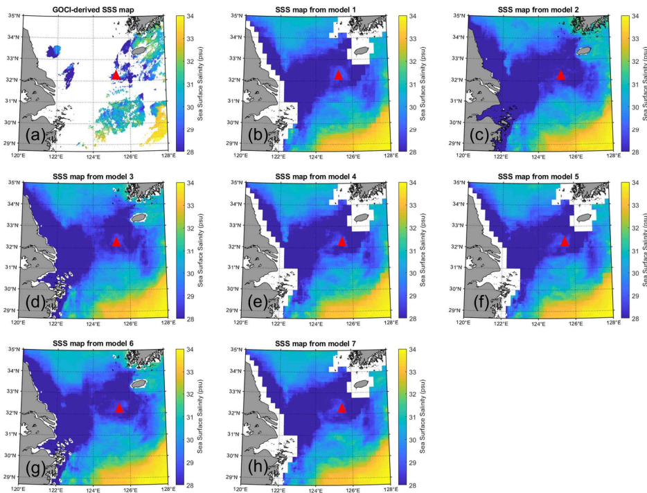
Figure 56: (a) GOCI-derived SSS map on 27 July 2016. (b)–(h) SSS maps estimated from seven models with the bagged trees. The estimated SSS maps were generated from input data on the same day as the GOCI-derived SSS map. The red triangle represents the I-ORS location.
