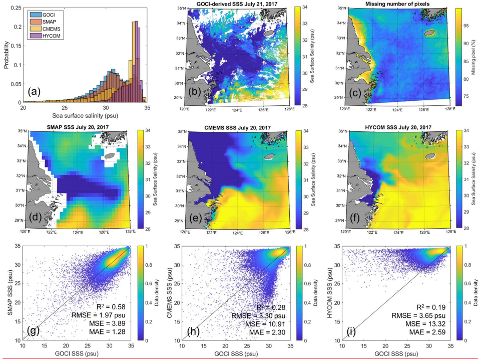
Figure 3: (a) Histogram of the GOCI-derived, SMAP, CMEMS, and HYCOM sea surface salinity (SSS) products in the study area. Spatial distributions of the (b) GOCI-derived, (d) SMAP, (e) CMEMS, and (f) HYCOM SSS data in the study area. (c) Spatial masking ratio of the GOCI-derived SSS maps based on the pixel unit. Scatter plots showing the consistency patterns between the GOCI-derived SSS and (g) SMAP, (h) CMEMS, and (i) HYCOM SSS data using the entire SSS range. Statistical indices: coefficient of determination ( R^2 ), root mean squared error (RMSE), mean squared errors (MSE), and mean absolute error (MAE).
