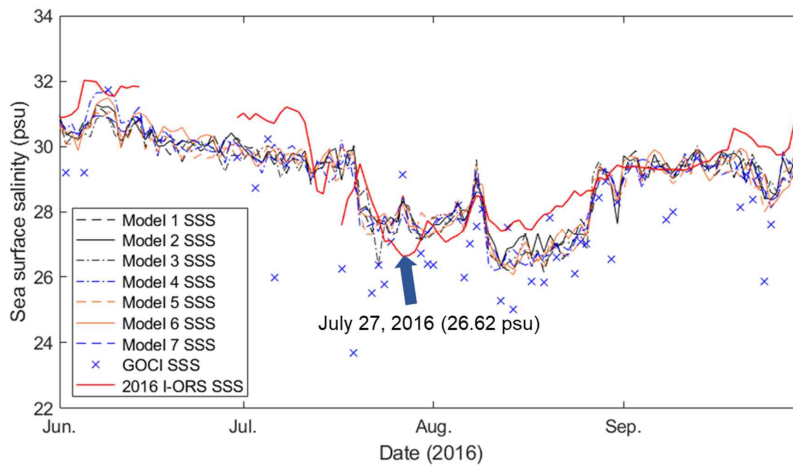
Figure 54: (a) SSS time series estimated from seven models with bagged trees and the GOCI-derived and in situ I-ORS SSS data over 122 days from 1 June 2016 to 30 September 2016.
