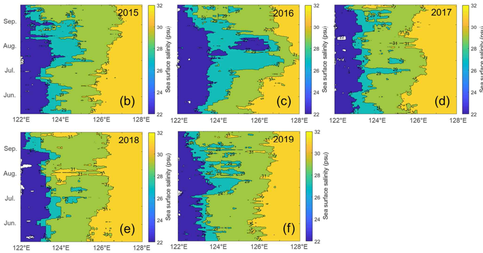
560 Figure 7: (a) SSS time series estimated by Model 1 (2015, 2016, 2017, and 2018) and Model 2 (2019) with bagged trees at the I-ORS location during the summer of 2015–2019. (Phase I) Beginning phase, (Phase II) development phase, and (Phase III) recovery phase of the CDW. In 2019, it was not possible to estimate the SSS with Model 1 because the SMAP SSS was not provided due to safe mode; therefore, Model 2 was used instead. (b)–(f) Time series of the 122–128°E horizontal transect (A–A' in Fig. 8a) during summer in each year. The plots were applied for the 27, 29, and 31 psu isohalines. The cross section in A–A' is located at 32.12°N.
