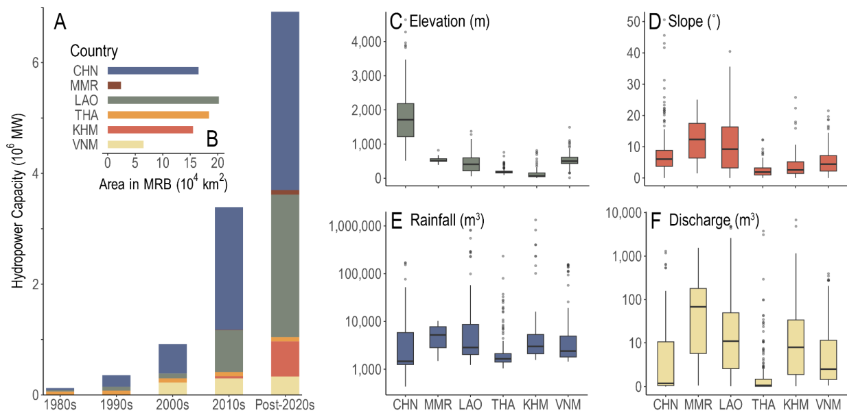
335 Figure 4: A. Total hydropower capacity of dams per country in each decade, from the 1980s to post-2020s, of which 36,058 MW is the total hydropower capacity of currently operational dams. The color and order of each country is indicated in B. B. Area of each country within the Mekong River Basin (MRB) (Rossi et al., 2009). C-F. Box plots per country showing the distribution of dam elevation, dam slope angle, mean total annual rainfall volume within each dam's nested catchment (2011-2015), and mean annual discharge at each dam (2011-2015) (Dang et al., 2022). Countries are labeled by their three-letter codes, ordered from upstream to downstream (similarly in Fig. 6 and 7).
