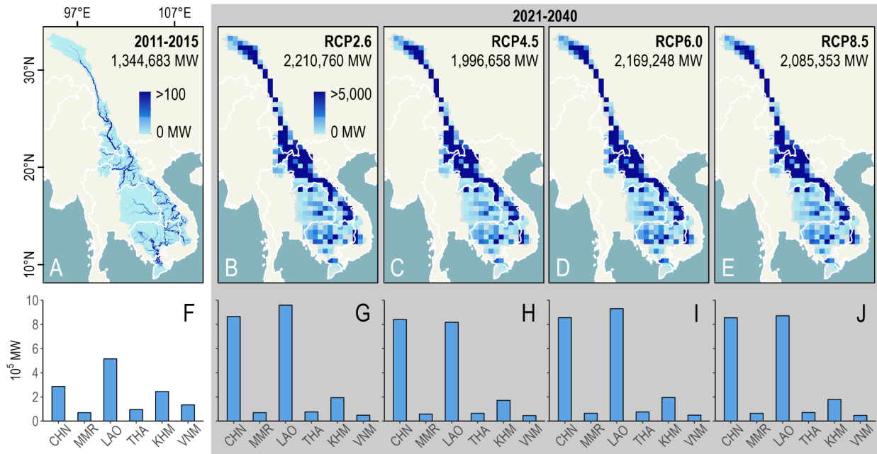
400 Figure 6: A. Theoretical hydropower potential in the Mekong Basin, estimated from gravity, elevation (relative to the downstream cell), and average annual discharge in 2011 to 2015. B-E. Hydropower potential estimated from average annual discharge in 2021 to 2040, modeled based on four Representative Concentration Pathways (B: 2.6, C: 4.5, D: 6.0, E: 8.5). F-J. Bar graph of the total hydropower potential in each country, corresponding to A-E.
