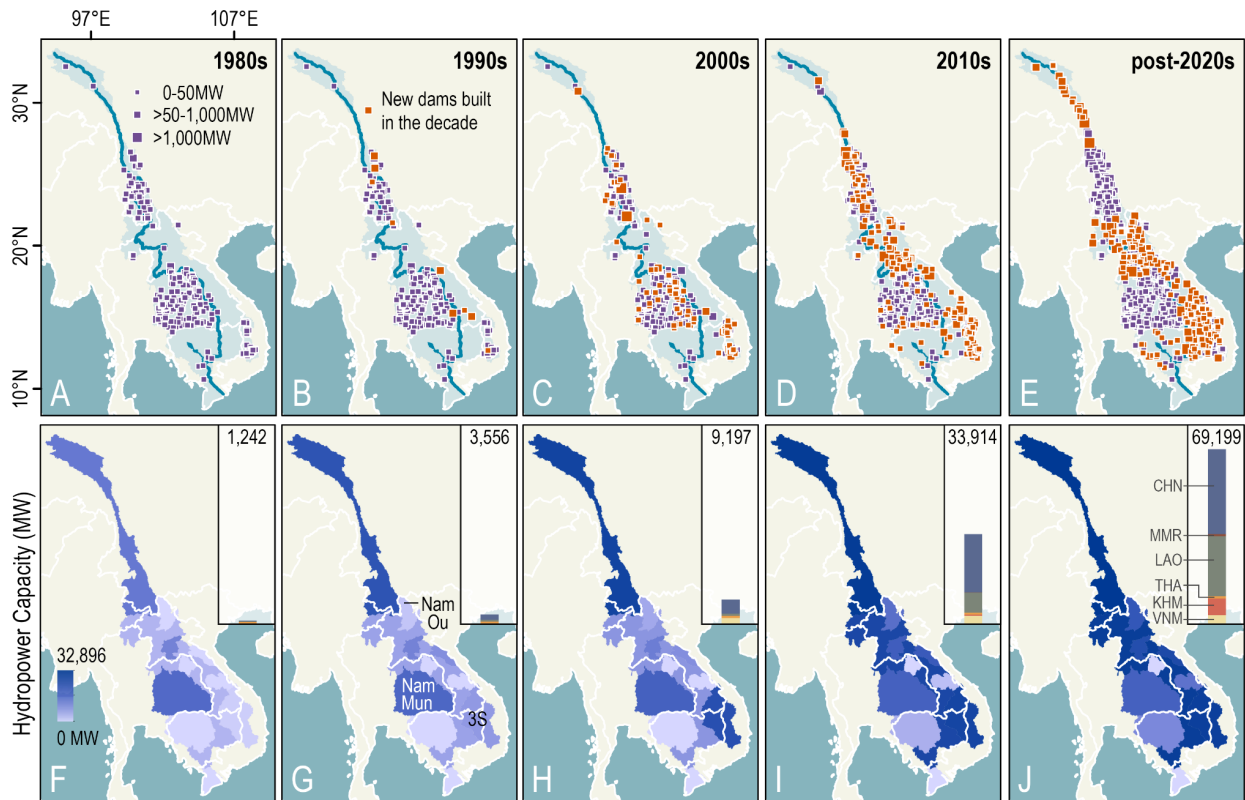
360 Figure 5: A-E. Distribution of the dams in each decade from the 1980s to post-2020s. Newly built dams in each decade are indicated in red. F-J. Total hydropower capacity of operating dams per major sub-basin, in each decade from the 1980s to post-2020s, with three notable basins labeled (Nam Ou, Nam Mun, 3S). Each sub-figure corresponds to each bar plot in Fig. 4A, labeled with the total hydropower capacity of the Mekong basin per decade.
