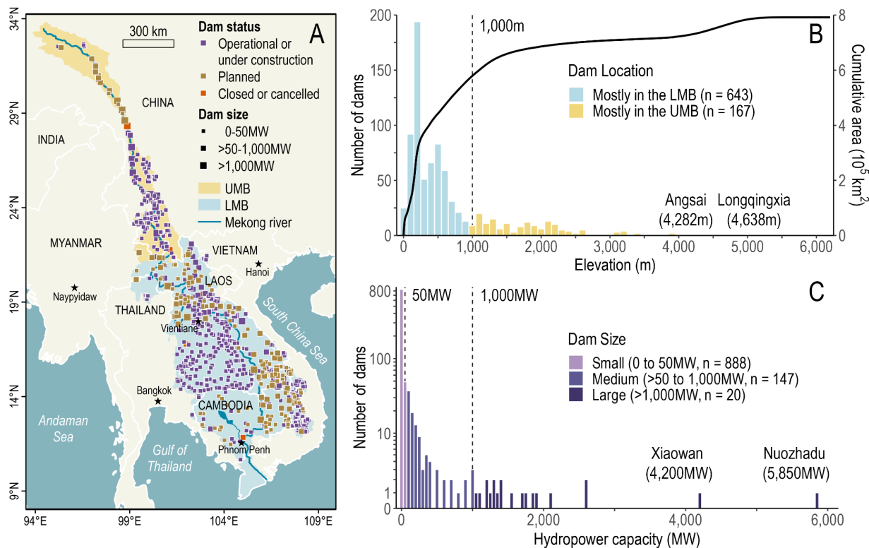
Figure 3: A. Map of the current dam network, with operational dams or dams under construction in purple, planned dams in yellow, and closed or canceled dams in red. B. Distribution of dams based on their elevation. Most dams of elevation below 1,000m lie in the Lower Mekong Basin (LMB), while most dams of elevation above 1000m lie in the Upper Mekong Basin (UMB). Around 75% of the Mekong Basin is below 1,000m, as shown by the hypsometric curve of cumulative area in the basin against elevation, derived from the 30m SRTM DEM. C. Distribution of hydropower dams based on their size (hydropower capacity), including the 245 dams without known specific coordinates. Small dams are 0 to 50 MW, medium dams are over 50 to 1,000 MW, while large dams are over 1,000 MW.
