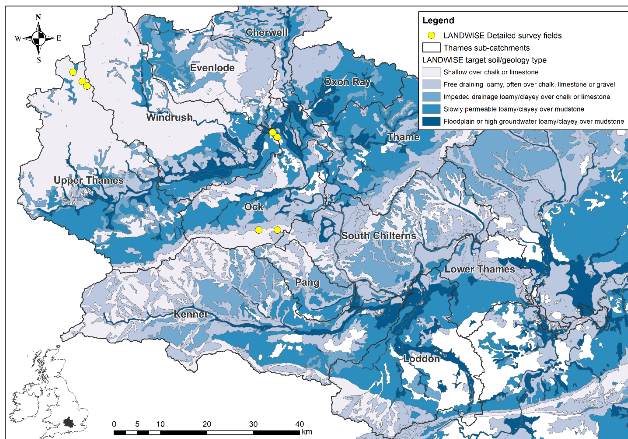
80 Figure 1: Locations and soil/geology types of the LANDWISE Detailed survey field sites within the Thames catchment, UK. Field locations are displayed to the nearest 1 km for participant anonymity purposes. See Table 1 for further details. Soils Data © Cranfield University (NSRI) and for the Controller of HMSO 2023. Map colours based on ColourBrewer: Color Advice for Maps (2023) by Cynthia A. Brewer, Geography, Pennsylvania State University.
