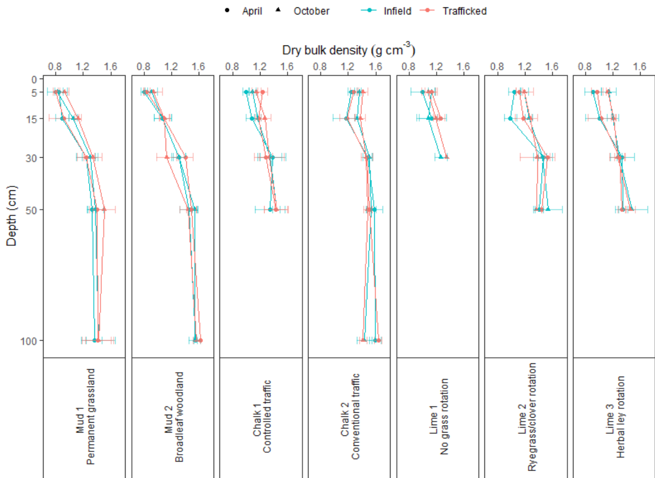
Figure 5: Changes in mean soil dry bulk density ( \text{g cm}^{-3} ) with depth (cm) at infield and trafficked locations sampled in April and October. Error bars represent standard deviations. Plotting on “Depth” axis is at lower limit of sampled depth, e.g. 45-50 cm samples are plotted at 50 cm.
