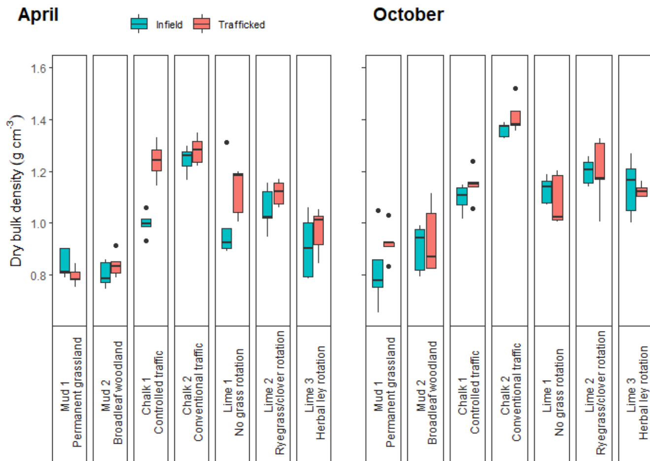
Figure 6: Box plots of soil surface (0-5 cm depth) dry bulk density ( \text{g cm}^{-3} ) sampled at infield and trafficked locations in April and October (pre- and post-harvest respectively for the arable sites).
