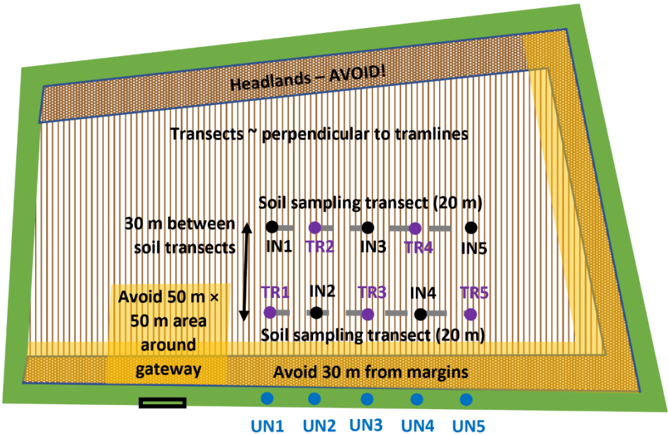
Figure 2: Schematic of the LANDWISE detailed survey transects and sampling locations within a typical field. IN = Infield; TR = Trafficked; UN = Untrafficked margin.
