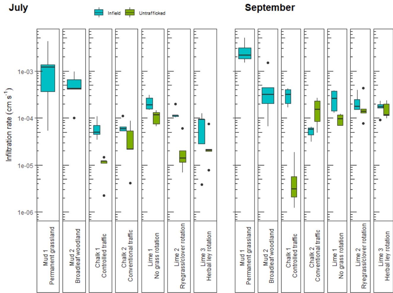
Figure 3: Box plots of infiltration rate ( \text{cm s}^{-1} ) measurements taken at infield and untrafficked margin locations in July and September (pre- and post-harvest respectively for the arable sites). Bold lines indicate median values. Note the log scale.
