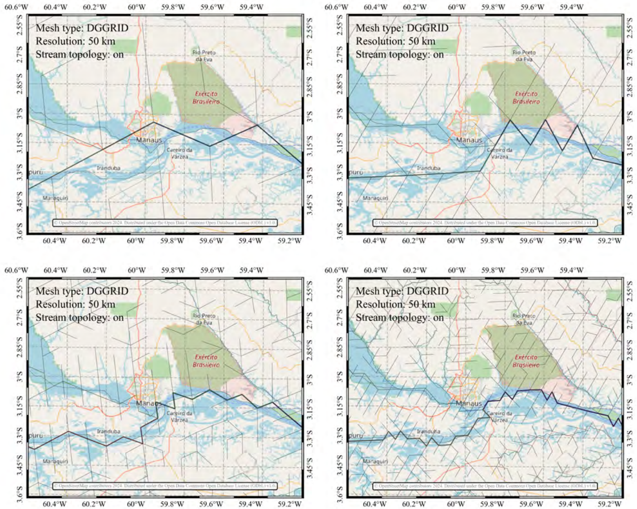
Figure C4. Zoom-in views of modeled flow direction at DGGRID ISEA3H level 10 to 13 resolutions in the Amazon Basin near Manaus. Black lines are cell-to-cell flow direction. Line thickness is scaled with drainage area. Colored and detailed black lines are conceptual and simplified HydroSHEDS river networks. The base images are Openstreet Map contributors 2024. Distributed under the Open Data Commons Open Database License (ODbL) v1.0.
