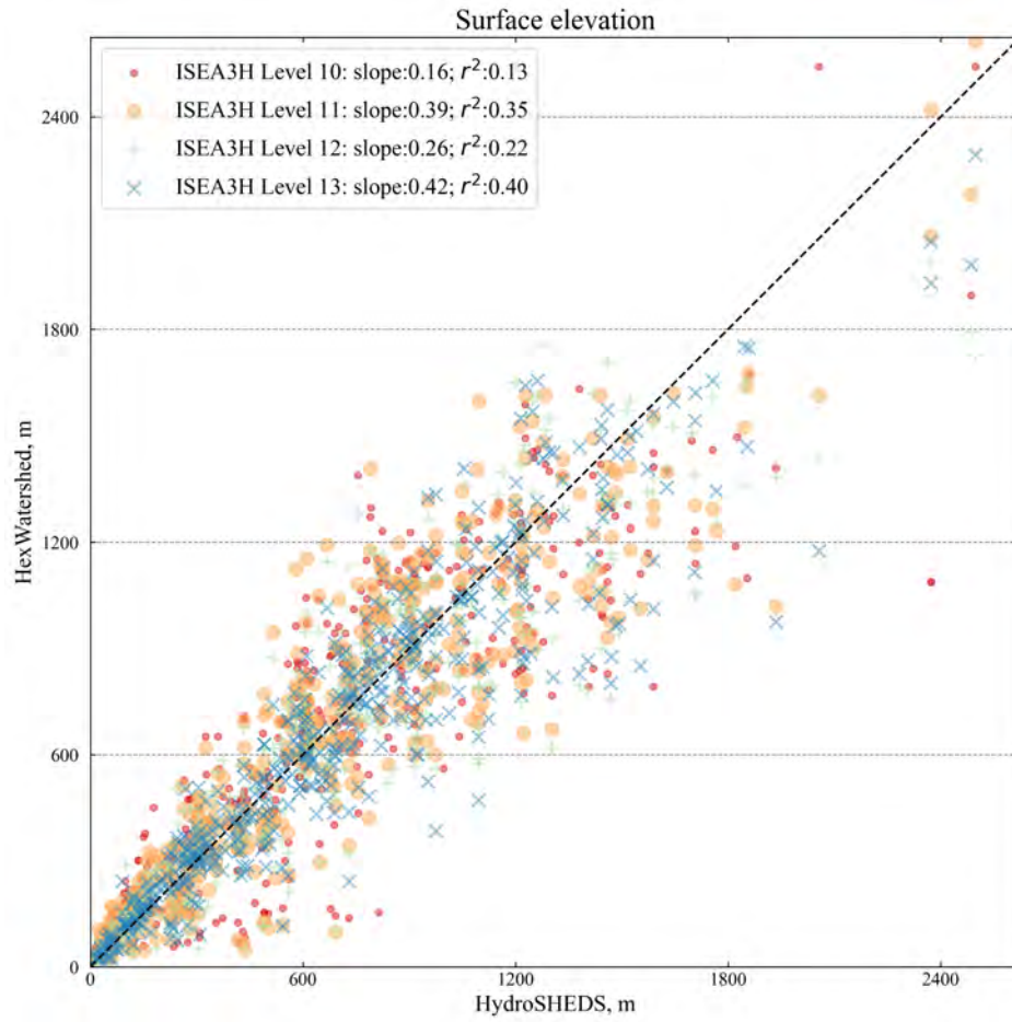
Figure 16. Validation of modeled surface elevation in the Yukon Basin from four DGGRID mesh resolutions. The x-axis X-axis is the sampled elevation from the HydroSHEDS DEM datasets. The y-axis Y-axis is the sampled surface elevation from our records (unit: m).
