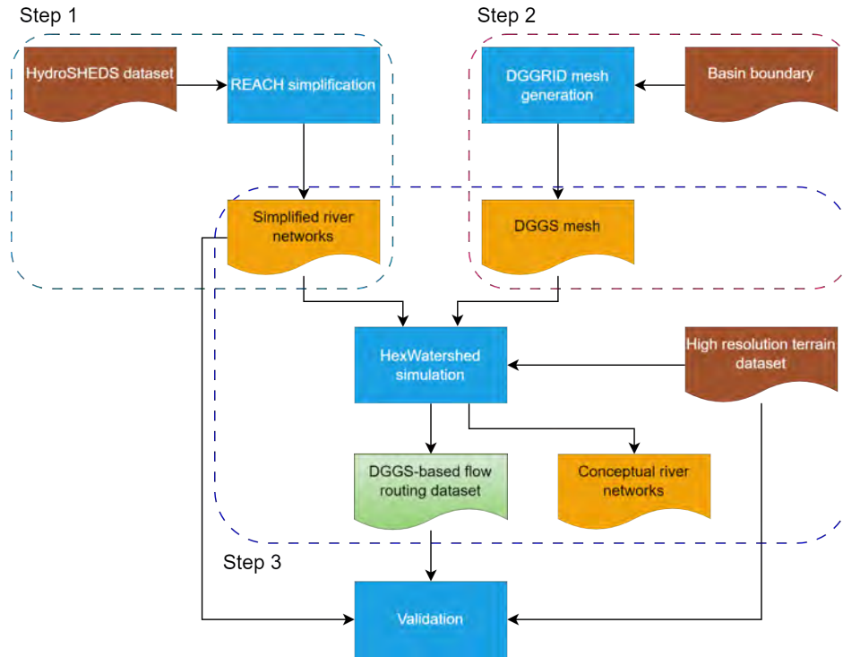
Figure 1. Workflow diagram demonstrating the DGGs-based DGGS-based flow routing dataset generation process using three steps (dashed boxes). Step 1: river network simplification using REACH; Step 2: DGGs DGGS mesh generation using DGGRID; Step 3: Flow routing direction modeling using HexWatershed ( including PyFlowline ). Brown boxes are user-provided datasets. Orange boxes are intermediate results ( e.g., conceptual river networks modeled by PyFlowline ). The light green box is the final data product.
