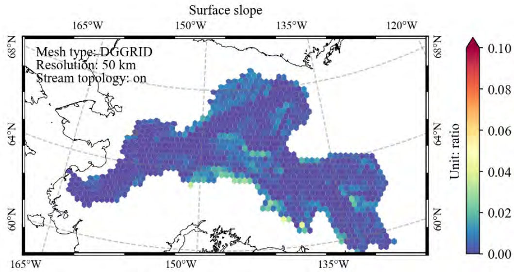
Figure 6. Spatial distribution of modeled mesh cell center to cell center slope at DGGRID ISEA3H level 10 resolution in the Yukon Basin (unit: percentratio ).
