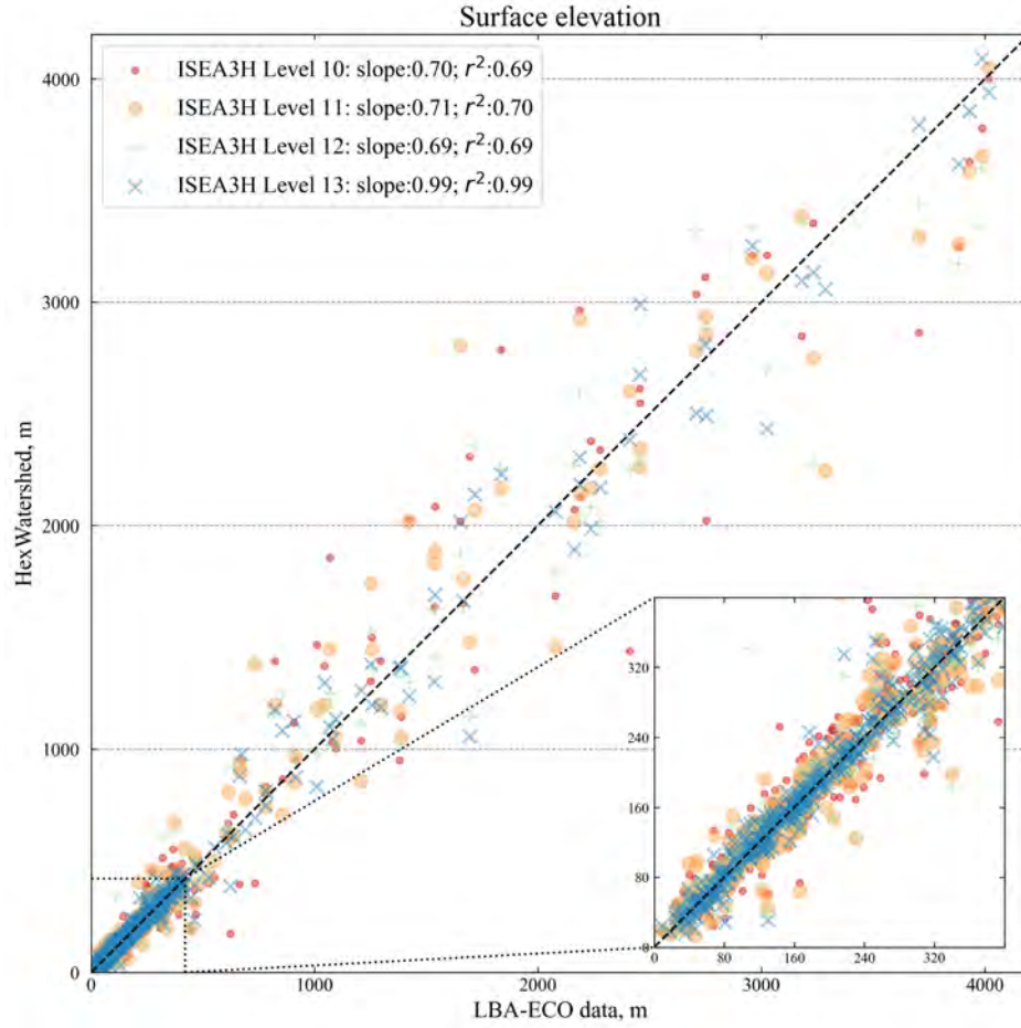
Figure 15. Validation of modeled surface elevation in the Amazon Basin from four DGGRID mesh resolutions. The x-axis is the sampled elevation from the LBA-ECO DEM datasets. The y-axis is the sampled surface elevation from our records (unit: m). The mini-plot is a zoom-in view of the lower left.
