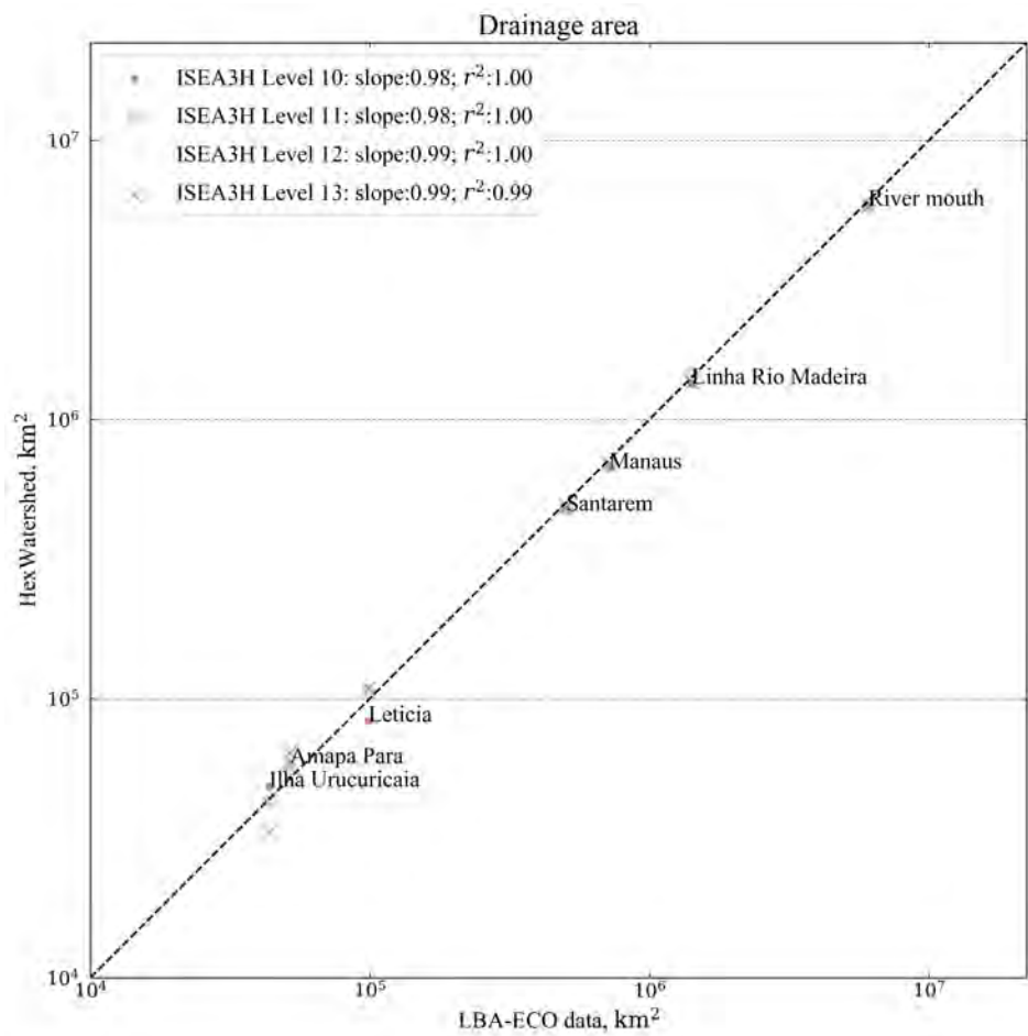
Figure 17. Validation of modeled drainage area of seven tributaries (including the river mouth) along the Amazon River from four DGGRID mesh resolutions. The x -axis- X -axis is the drainage area from the LBA-ECO CD-06 Amazon River Basin Land and Stream Drainage Direction datesets (converted from flow accumulation). The y -axis- Y -axis is the modeled drainage area (units: km 2 ). Both the x - X and y - Y axes are in the log scale.
