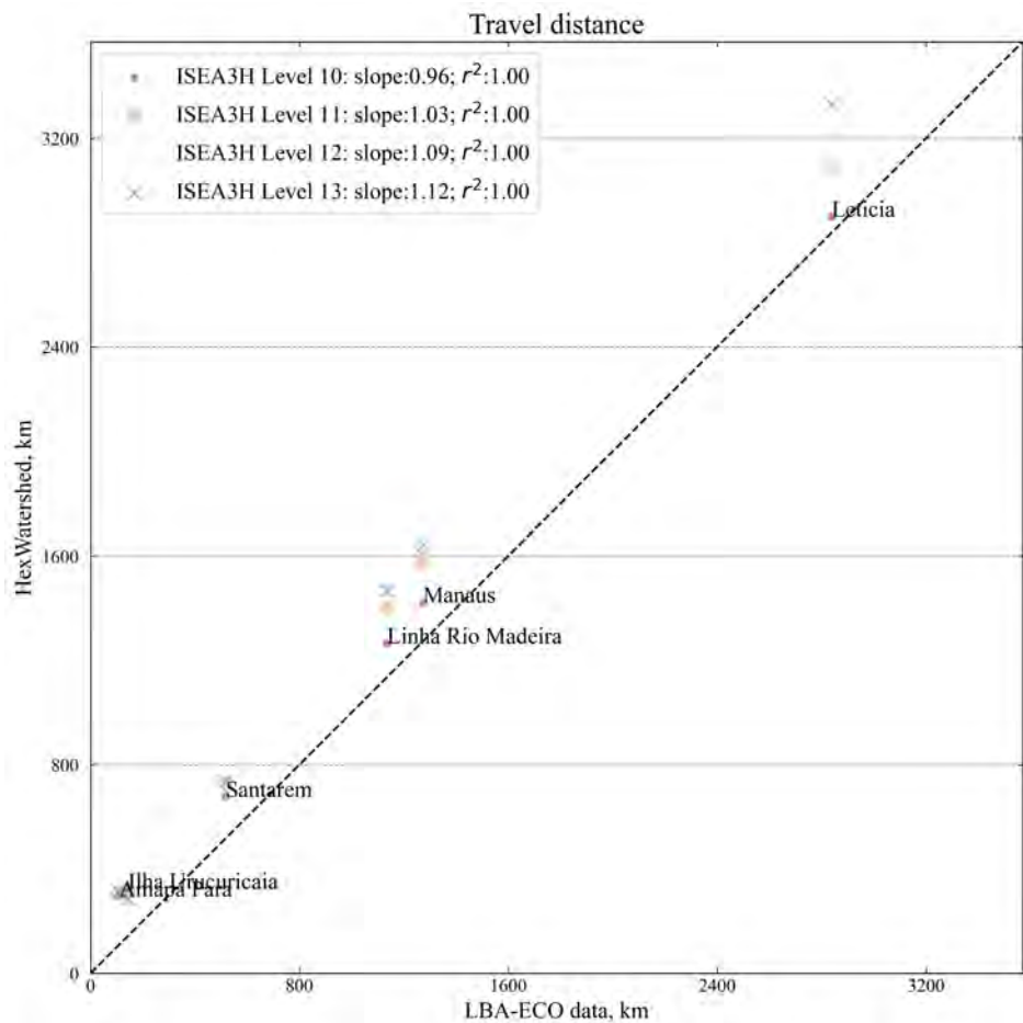
Figure 19. Validation of modeled travel distance of six tributaries along the Amazon River from four DGGRID mesh resolutions. The x-axis X-axis is the travel distance from the LBA-ECO CD-06 Amazon River Basin Land and Stream Drainage Direction datesets. The y-axis Y-axis is the modeled travel distance (unit: km).
