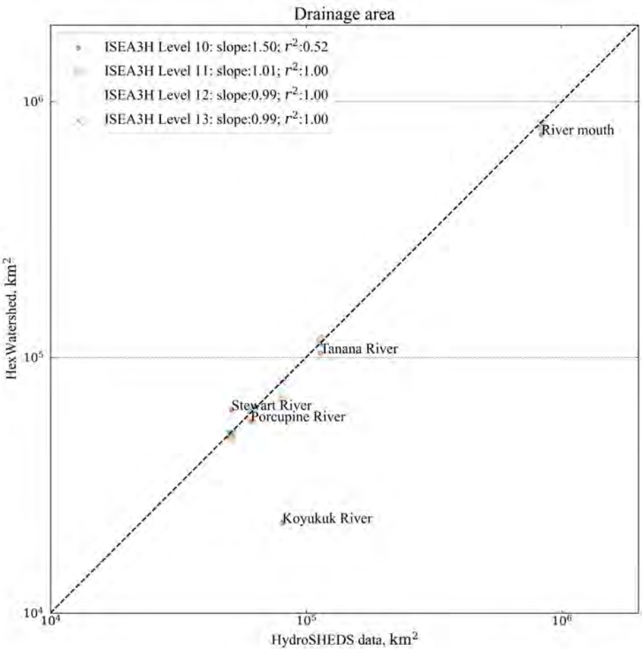
Figure 18. Validation of modeled drainage area of six tributaries along the Yukon River from four DGGRID mesh resolutions. The x -axis X-axis is the drainage area from the HydroSHEDS datasets. The y -axis Y-axis is the modeled drainage area (units: km 2 ). Both the x - X and y - Y axes are in the log scale.
