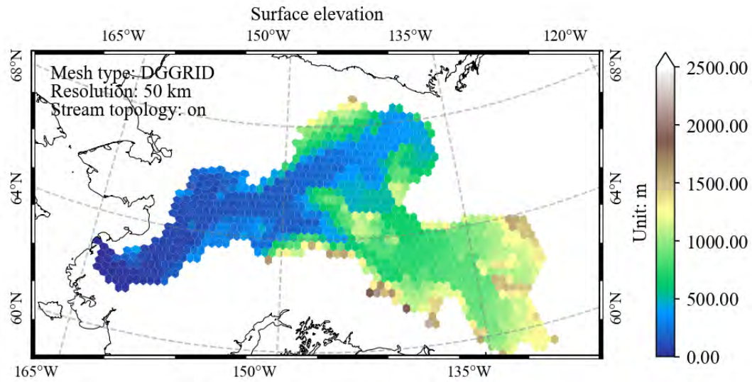
Figure 4. Spatial distribution of modeled surface elevation at DGGRID ISEA3H level 10 resolution in the Yukon Basin (unit: m).
