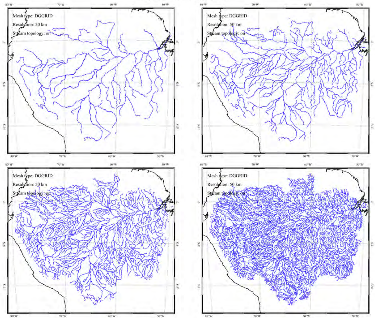
Figure 2. Simplified river networks using the REACH library at DGGRID ISEA3H level 10 to 13 resolutions in the Amazon Basin ( Table 1 ). Black and blue lines are coastlines and river networks, respectively. As these datasets are extracted using the Amazon watershed boundary from the global HydroSHEDS river networks, there may be isolated river segments near the boundary of the basin, which are automatically excluded in the HexWatershed model.
