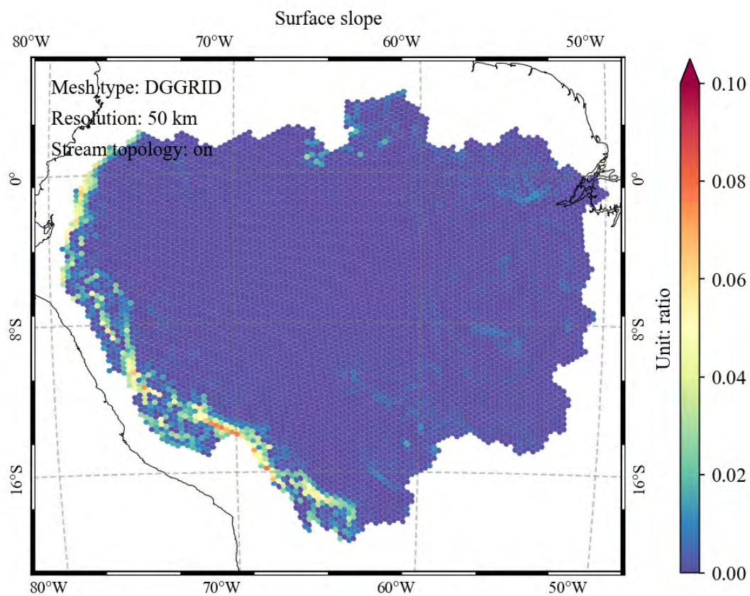
Figure 5. Spatial distribution of modeled mesh cell center to cell center slope at DGGRID ISEA3H level 10 resolution in the Amazon Basin (unit: percentratio ).
