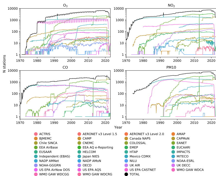
Figure 8. Evolution of the number of stations in GHOST, in each month across the time record (1970-2023), for 4 key components: O_3 , NO_2 , CO, and PM_{10} . The differing number of stations per reporting network are represented by different coloured lines. The total number of stations across all networks is shown in black.
