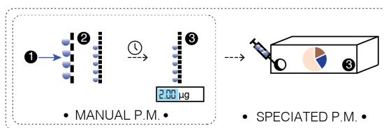
Figure 3. Visual illustration of the 3 GHOST standard measurement process steps, and how those steps are combined in the most typical measurement configurations. The 3 standard steps are sampling, preparation, and measurement.
