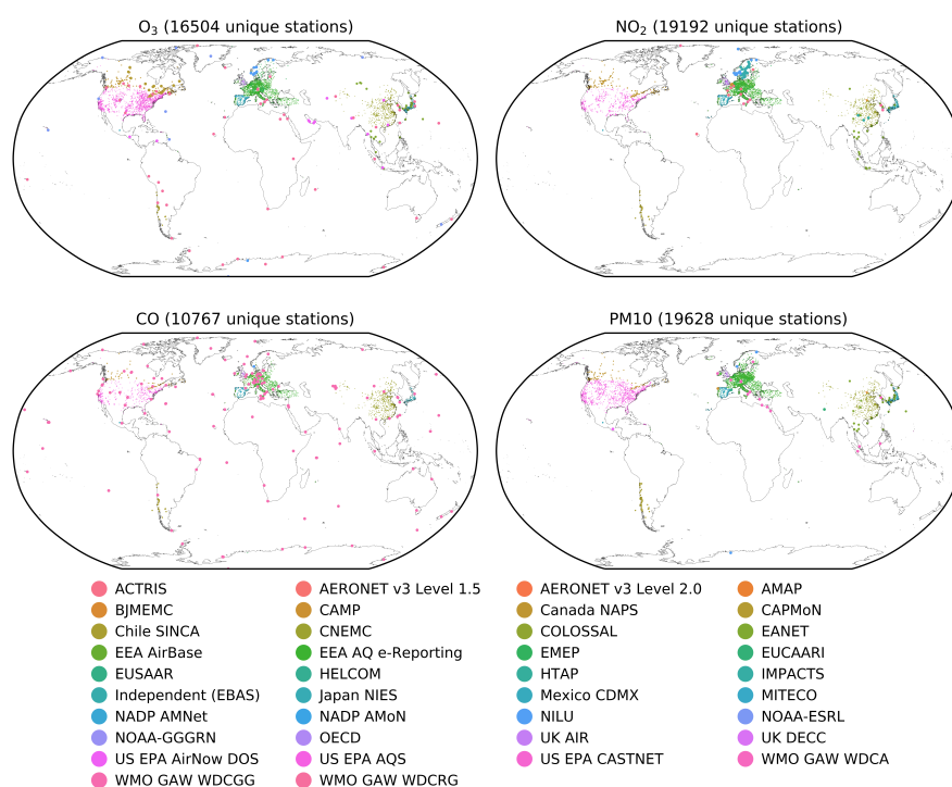
Figure 9. Spatial distribution of all unique stations in GHOST, across the time record (1970-2023), for 4 key components: O 3 , NO 2 , CO, and PM 10 . The stations are coloured by reporting network. The number of unique stations across the time record, per component, are given in the map titles.
