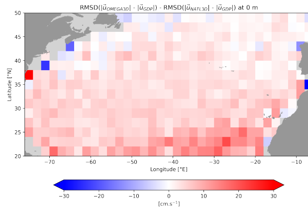
Figure 9. Difference between WOC-NATL3D RMSD (Fig. 2b) and OMEGA3D RMSD (Fig. 8b) at the surface, over the period 2010-2016. The RMSDs are computed from GDP drifter velocities.
