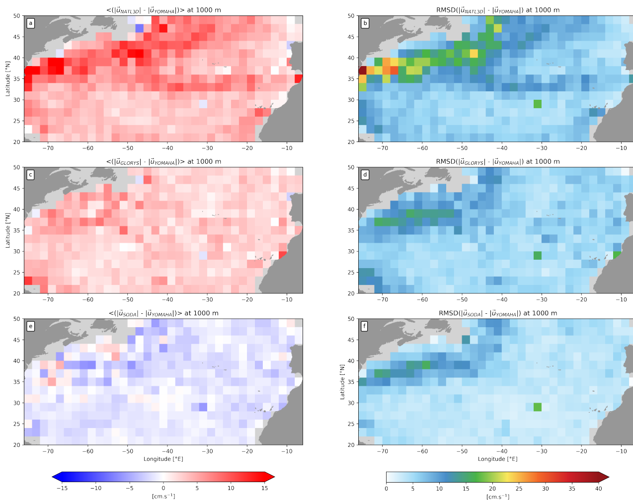
Figure 6. Mean biases (left panels) and RMSDs (right panels) between YOMAHA drifters and WOC-NATL3D (a,b), GLORYS (c,d) and SODA (e,f) currents at 1000 m in 2^\circ \times 2^\circ bins, computed over the period 2010-2016.
