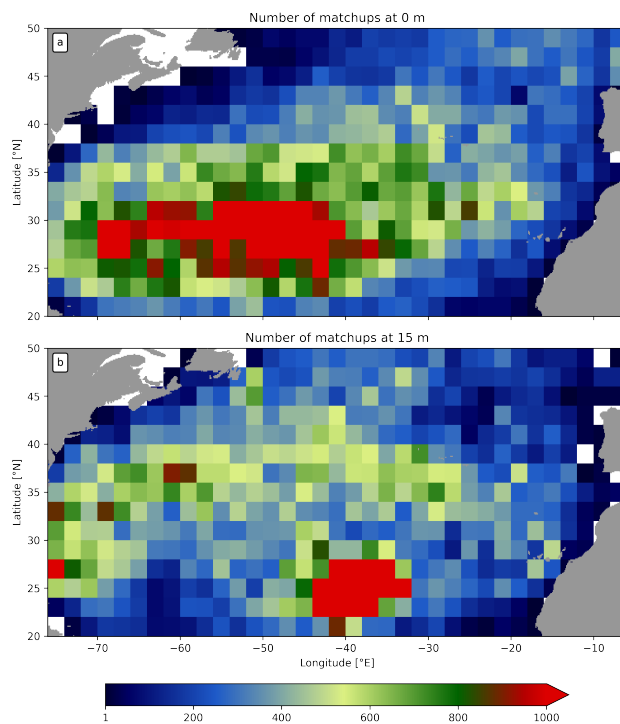
Figure A1. Number of matchups between WOC-NATL3D, DUACS, GLORYS, SODA and GDP drifters at 0 m (a) and between WOC-NATL3D, GLORYS, SODA and GDP drifters at 15 m (b). These matchups numbers are computed over the period 2010-2016 and within 2^\circ \times 2^\circ bins.
