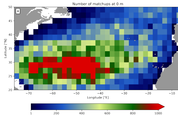
Figure C1. Number of matchups between WOC-NATL3D, OMEGA3D and GDP drifters at 0 m, computed over the period 2010-2016 and within 2^\circ \times 2^\circ bins.
