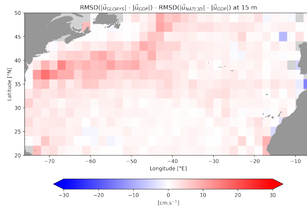
Figure 5. Difference between WOC-NATL3D RMSD (Fig. 4b) and GLORYS (Fig. 4d) at 15 m depth, over the period 2010-2016. The RMSDs are computed from GDP drifter velocities.
