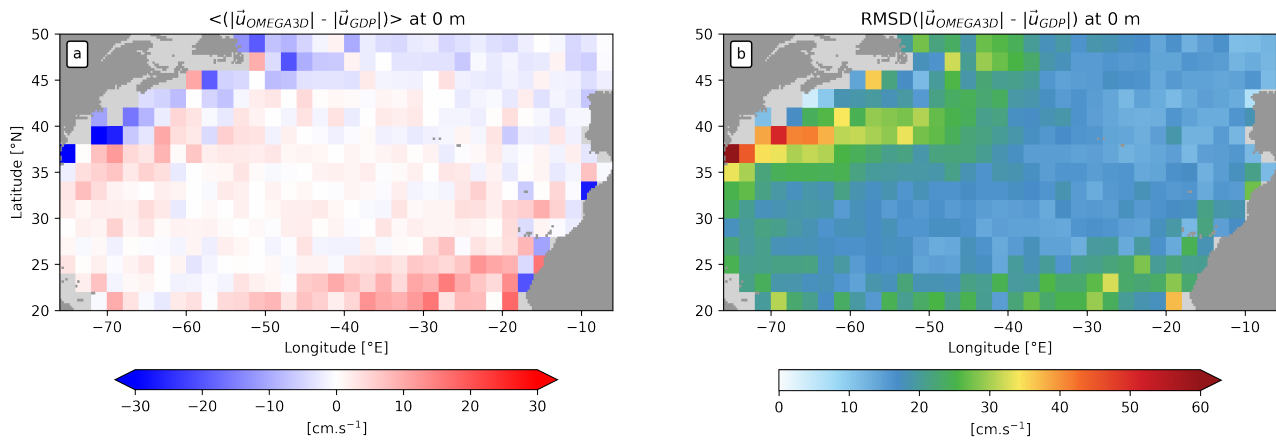
Figure 8. Mean bias (a) and RMSD (b) between GDP drifters and OMEGA3D surface currents in 2°x2° bins, computed over the period 2010-2016.
