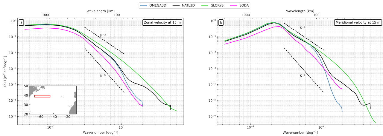
Figure 10. Power spectra density ( \text{m}^2 \text{s}^{-2} \text{deg}^{-1} ) of horizontal velocity at 15 m depth averaged over 2010–2016: zonal component (a) and meridional component (b). The spectra are performed in the box shown in the inset map. Dashed lines indicate slopes of -3 and -5 .
