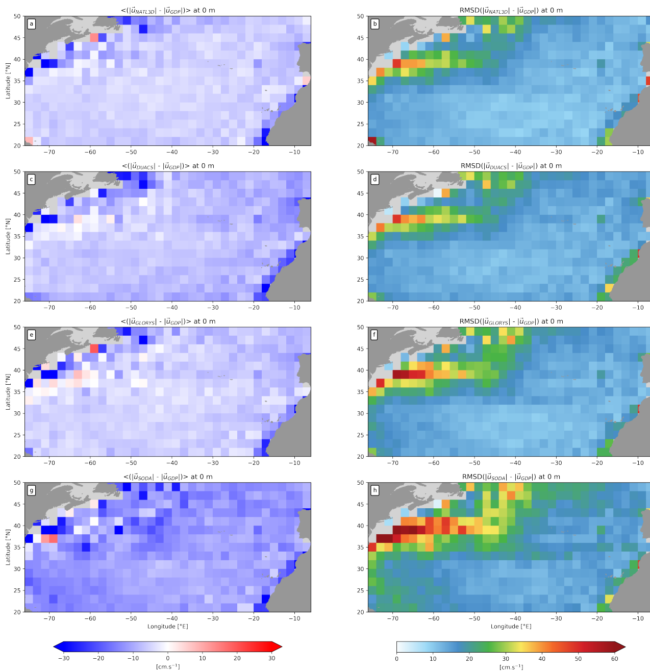
Figure 2. Mean biases (left panels) and RMSDs (right panels) between GDP drifters and WOC-NATL3D (a,b), DUACS (c,d), GLORYS (e,f) and SODA (g,h) surface currents in 2^\circ \times 2^\circ bins, computed over the period 2010-2016.
