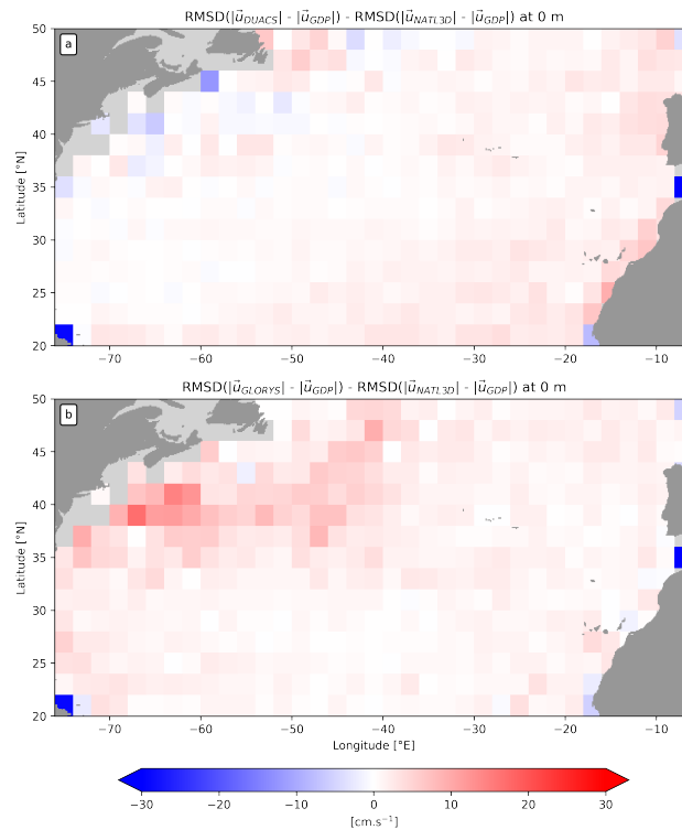
Figure 3. The top panel is the difference between WOC-NATL3D RMSD (Fig. 2b) and DUACS RMSD (Fig. 2c) and the bottom panel is the difference between WOC-NATL3D RMSD (Fig. 2b) and GLORYS (Fig. 2d). They are computed at the surface over the period 2010-2016. The RMSDs are computed from GDP drifter velocities.
