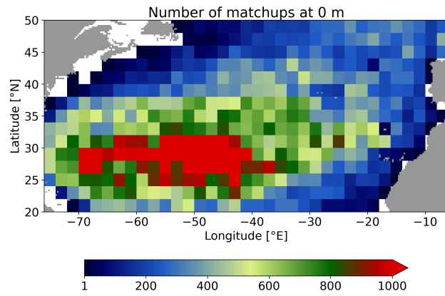
Figure C1. Number of matchups between WOC-NATL3D, OMEGA3D and GDP drifters at 0 m, computed computed over the period 2010-2016 and within 2^\circ \times 2^\circ bins.
