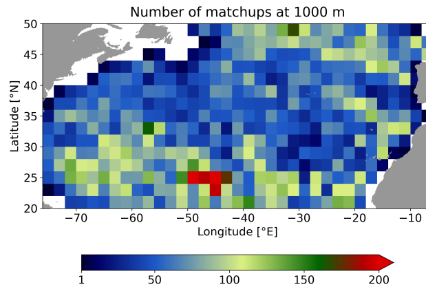
Figure B1. Number of matchups between WOC-NATL3D, GLORYS, SODA and YOMAHA drifters at 1000 m, computed computed over the period 2010-2016 and within 2^\circ \times 2^\circ bins.
