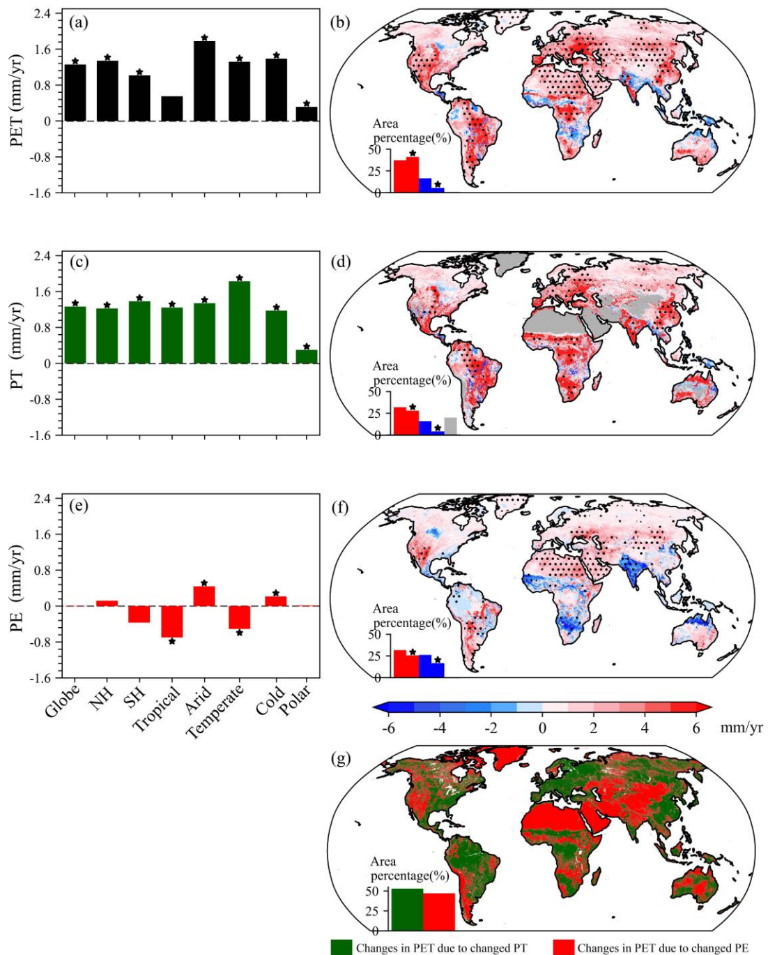
1190 Figure 11: Characteristics of annual PET, PT and PE trends, and major contributors to annual PET trends. (a): Trends for annual PET averaged over the globe, each hemisphere, and each KG climate region. (b): Spatial distribution of annual PET trends. (c): Trends for annual PT averaged over the globe, each hemisphere, and each KG climate region. (d): Spatial distribution of annual PT trends. (e): Trends for annual PE averaged over the globe, each hemisphere, and each KG climate region. (f): Spatial distribution of annual PE trends. (g): Spatial distribution of major contributors 1195 to annual PET trends. In (a), (c) and (e), the star indicates that the trend is significant ( p < 0.05 ). In (b), (d) and (f), the inset histogram suggests area percentage of insignificant increases (red bar without star), significant increases (red bar with star; p < 0.05 ), insignificant decreases (blue bar without star), and significant decreases (blue bar with star; p < 0.05 ).
