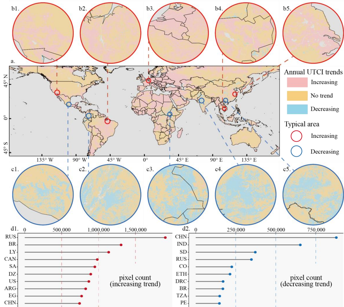
390 Figure 8. Significant trends in annual UTCI for global pixels: (a) spatial distribution; (b1) - (b5) typical areas with increasing trend in annual UTCI; (c1) - (c5) typical areas with decreasing trend in annual UTCI; (d1) top 10 countries with the highest number of pixels showing an increasing trend in the annual UTCI; and (d2) top 10 countries with the highest number of pixels showing a decreasing trend in the annual UTCI.
