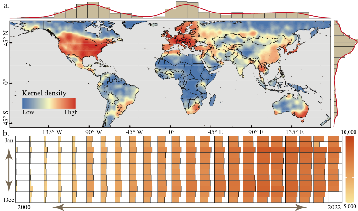
Figure 1. Global monthly meteorological observation samples from 2000 to 2022: (a) kernel density; and (b) quantitative statistics.
