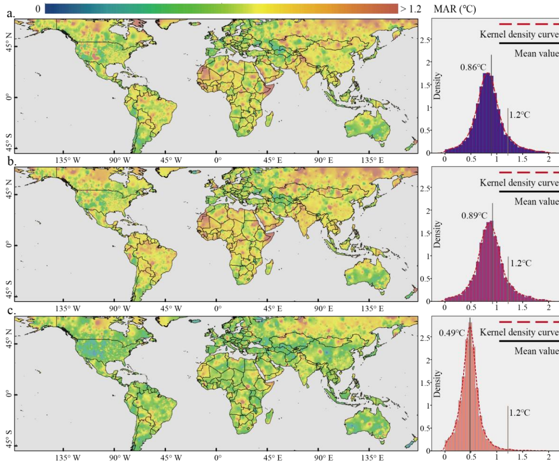
Figure 4. Spatially interpolated distribution and statistics of MAR between predicted UTCI and observed UTCI for global meteorological stations: (a) XGBoost; (b) LightGBM; and (c) CatBoost.
