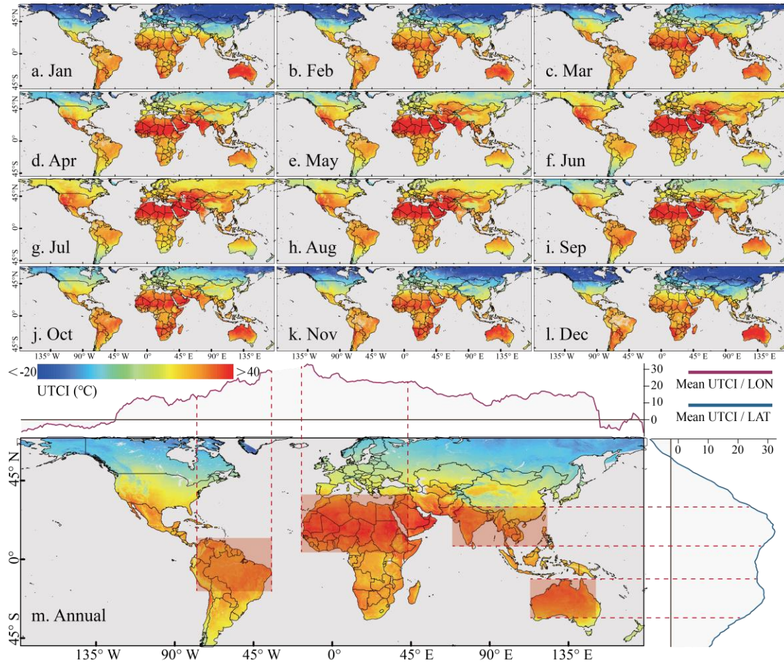
Figure 5. Global distribution of monthly and annual UTCI in 2021.
