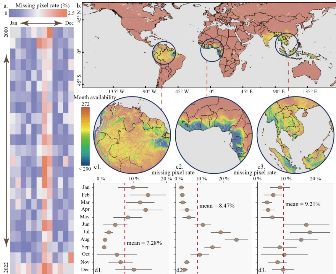
Figure 10. Month availability of pixels for GloUTCI-M data: (a) global missing pixel rate for each month; (b) spatial distribution of month availability; (c1) - (c3) areas of densely missing pixels for monthly data; and (d1) - (d3) missing pixel rate by month for areas of densely missing pixels.
