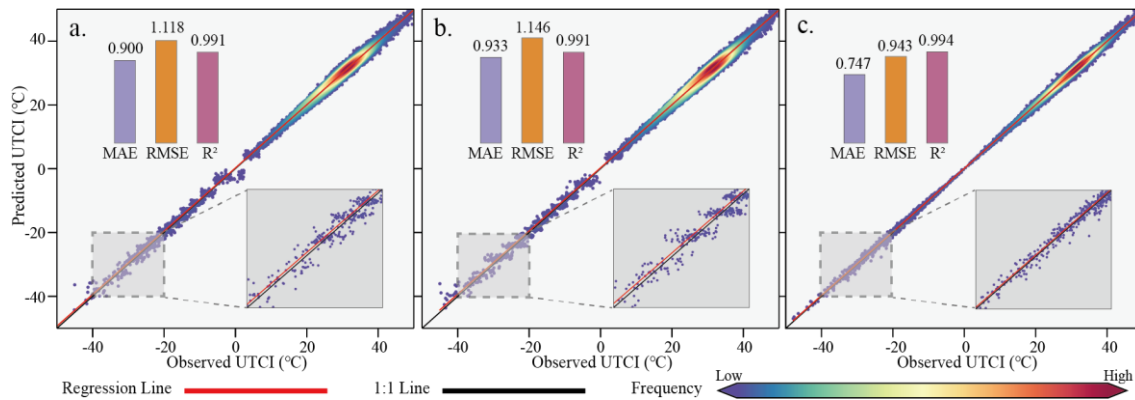
Figure 3. Comparison of predicted UTCI derived from machine learning models with observed UTCI obtained from meteorological station samples: (a) XGBoost; (b) LightGBM; and (c) CatBoost.
