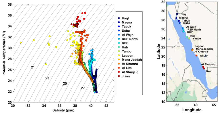
Figure 2: T–S diagram encompassing all data taken (averaged every 1 m) in the Red Sea. Dots of the same colour indicate measurements taken at the same site as shown on the map on the right (© Google Maps, 2021).
