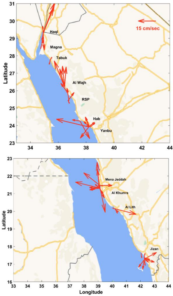
Figure 4: Current vectors at 12 m at specific areas along the Saudi Arabian coast of Aqaba and Red Sea. Scale vector of a westward current with a speed of 15 cm/s appears in the upper right of the top panel (© Google Maps, 2021).
