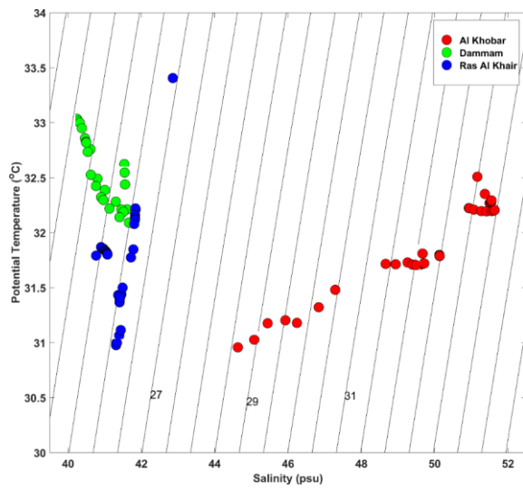
Figure 11: T-S diagram for all measured stations in the Arabian Gulf. The three colours of dots represent the three hotspot sites. Measurements are averaged every 1 m in the water column up to 0.5 m from the sea bottom.
