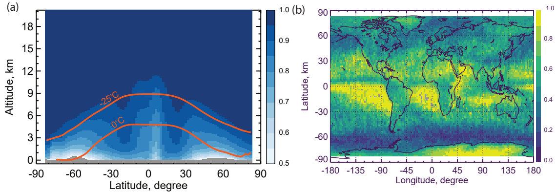
Figure 11. (a): Fraction of Level 2 5 km profiles reaching a given altitude before becoming fully attenuated, annual average for 2008; (b) fraction of cloudy profiles where cloud optical depth above the freezing level is less than 2, for 2008.
