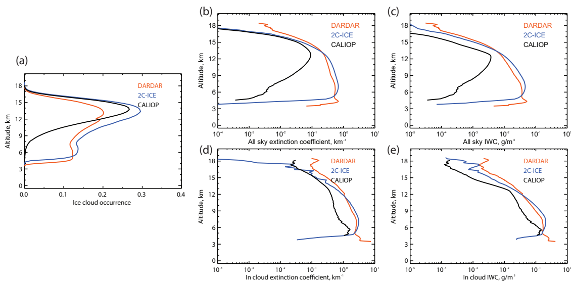
Figure 19. Comparison of ice cloud occurrence (a), extinction coefficient (b, d) and IWC (c, e) profiles from L3-ICE, DARDAR, and 2C-ICE radar/lidar products in the northern tropics ( 0^\circ - 30^\circ \text{ N} ) for July 2008. Mean all-sky extinction coefficient and IWC plotted in (b) and (c) are calculated using Equation 6. Mean in-cloud extinction coefficient and IWC plotted in (d) and (e) are calculated using Equation 5.
