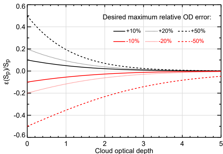
Figure 3. Lidar ratio accuracy required to achieve optical depth accuracy of 10%, 20% or 50%, based on Eq. 41 in Young et al., (2013).
