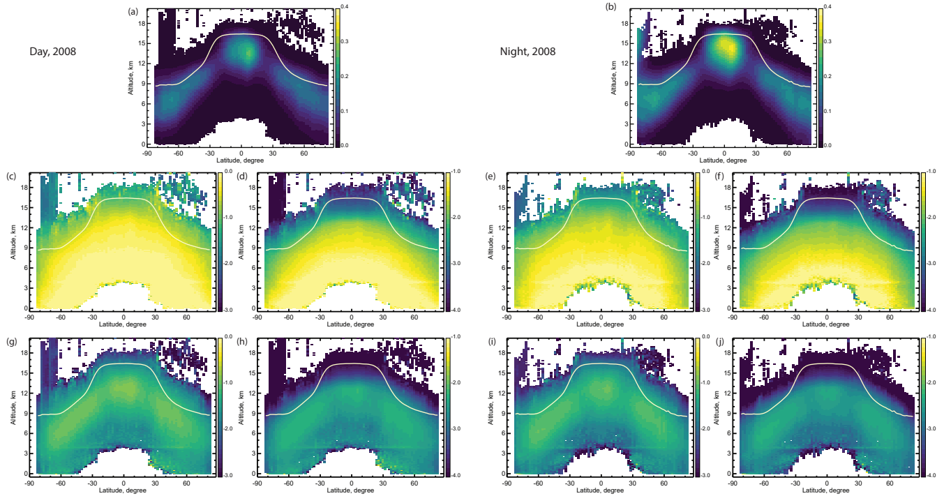
Figure 7. Annual zonal mean ice cloud occurrence (a, b), in-cloud extinction coefficient (c, e), in-cloud IWC (d, f), all-sky extinction coefficient (g, i), and all-sky IWC (h, j) for 2008 at the L3-ICE resolution of 2.0^\circ latitude and 120 m altitude. Color bars for extinction coefficient and IWC are logarithmic. The white line indicates zonal annual mean tropopause height. Left: day; right: night.
