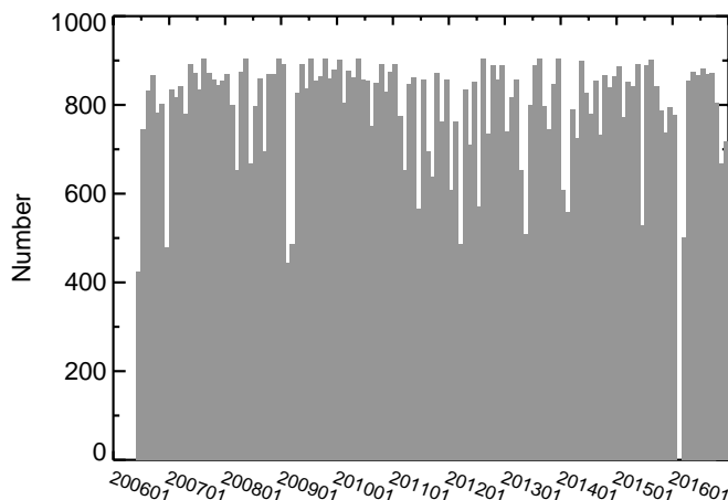
Figure 6. The total numbers of processed L2 5 km cloud profile product files, including both daytime and nighttime granules, used in the V1.00 L3-ICE product.
