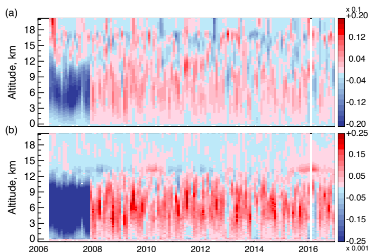
Figure 10. Deseasonalized time series of monthly global anomalies of (a) ice cloud occurrence and (b) all-sky IWC from 2006 to 2016. Color coding indicates relative variation from the mean with a range of \pm 2\% for ice cloud occurrence and \pm 0.25 \times 10^{-3} \text{ g m}^{-3} for IWC. The blue regions below 12 km and prior to December 2007 show the impact of the different sensitivities of CALIOP to HOI at view angles of 0.3^\circ (prior to December 2007) and at 3.0^\circ .
