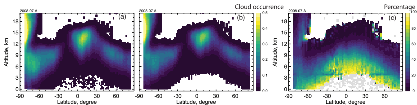
Figure 8. Zonal ice cloud occurrence for July 2008 (night) before (a) and after (b) filtering. Cloud occurrence from 0 to 0.5 is coded in color. Panel (c) plots the percentage of samples removed by filtering ((100 \times N_{rej}/N_{ice})\%) with gray representing 100% removal.
