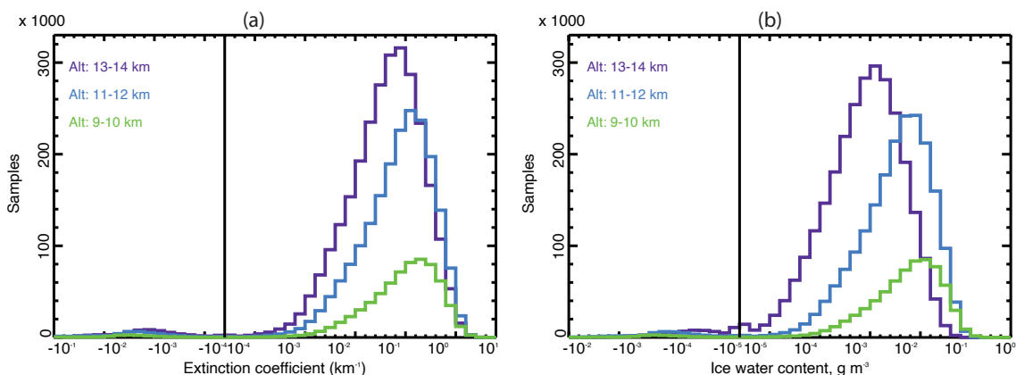
Figure 4. Histograms of night-time ice cloud 532 nm channel extinction coefficients (a) and IWC (b) observed at three altitudes in the tropics (23.5° S - 23.5° N) in July 2008. The X-axis is a split logarithmic scale to show both positive and negative values. The vertical solid line separates negative and positive values.
