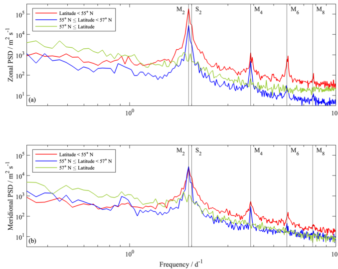
435 Figure 8: Mean power spectral density on (a) the zonal u and (b) the meridional v drifter velocities in the North Sea averaged over all trajectories. The periods of the semidiurnal and shallow water tidal components are indicated by the vertical lines.
