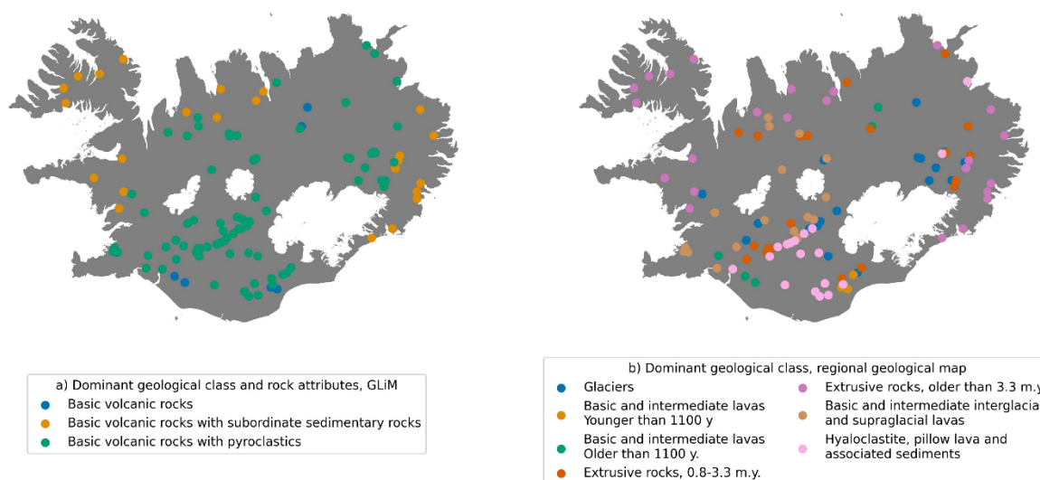
Figure 10: The dominant geological class of each catchment in LamaH-Ice, as depicted in a) the GLiM global lithological map, levels 2 and 3 (Hartmann et al., 2012), and b) a regional geological map of Iceland (Icelandic Institute of Natural History, 2014). M.y. stands for million years. Basemap source: Hijmans, 2015.
