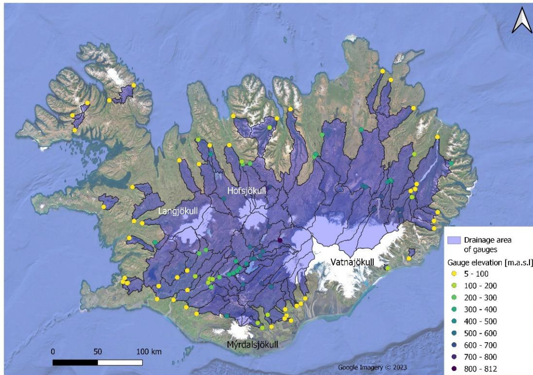
Figure 1: Locations of gauges included in LamaH-Ice and their drainage areas. The elevation of each gauge is indicated with colors. Made with QGIS. Source of background map: Google, 2023.
