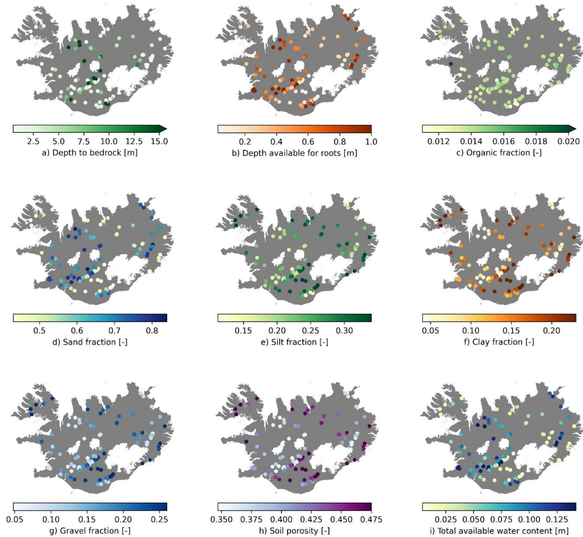
485 Figure 9: Spatial distribution of soil attributes for the catchments in LamaH-Ice. Basemap source: Hijmans, 2015.
