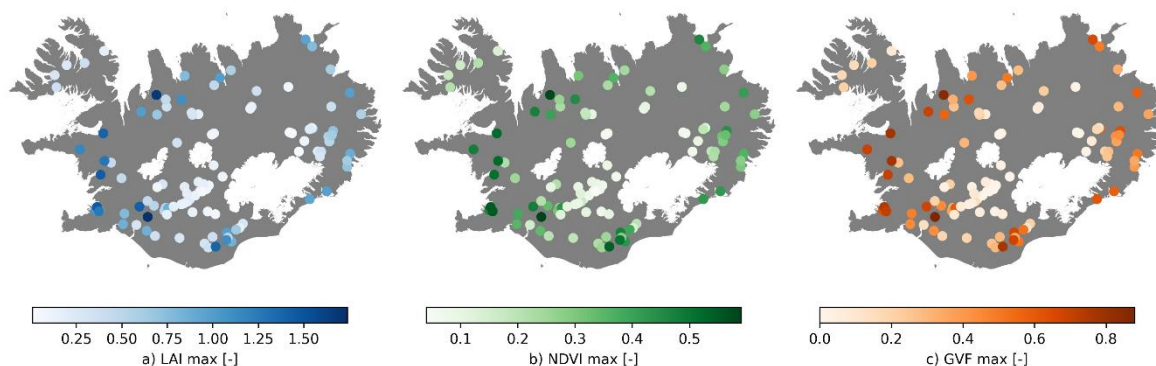
460 Figure 8: The spatial distribution of static vegetation indices for the catchments in LamaH-Ice. Basemap source: Hijmans, 2015.
