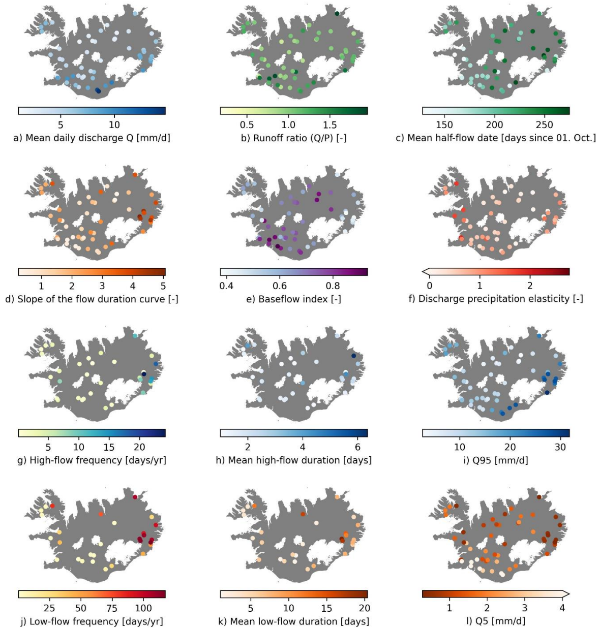
Figure 6: Spatial distribution of hydrological signatures. The signatures were calculated using measured streamflow series and RAV-II precipitation for the 37-year period between October 1, 1981 and September 30, 2018. Only hydrological years with at least 90% temporal coverage during this period were considered. Gauges with less than three years of 90% coverage were omitted. The total number of gauges shown is 54. Panels g, h, j, and k describe the frequency and duration of high- and low-flows. The number of gauges shown in these panels is lower since high- and low-flows, as they are defined here, do not occur in all gauges. Basemap source: Hijmans, 2015.
