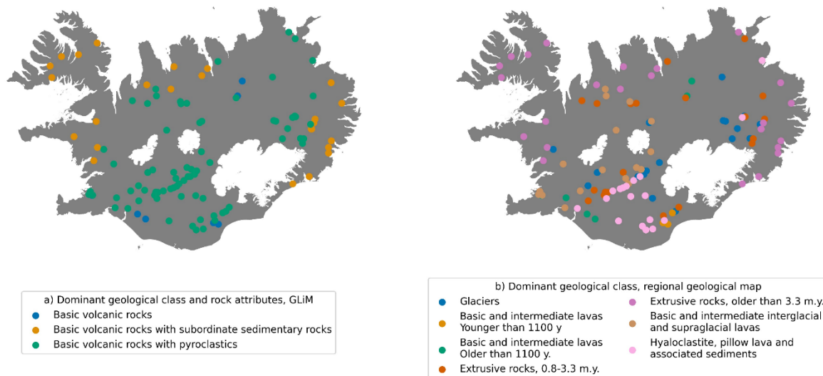
510 Figure 10: The dominant geological class of each catchment in LamaH-Ice, as depicted in a) the GLiM global lithological map, levels 2 and 3 (Hartmann et al., 2012), and b) a regional geological map of Iceland (Icelandic Institute of Natural History, 2014). M.y. stands for million years. Basemap source: Hijmans, 2015.
