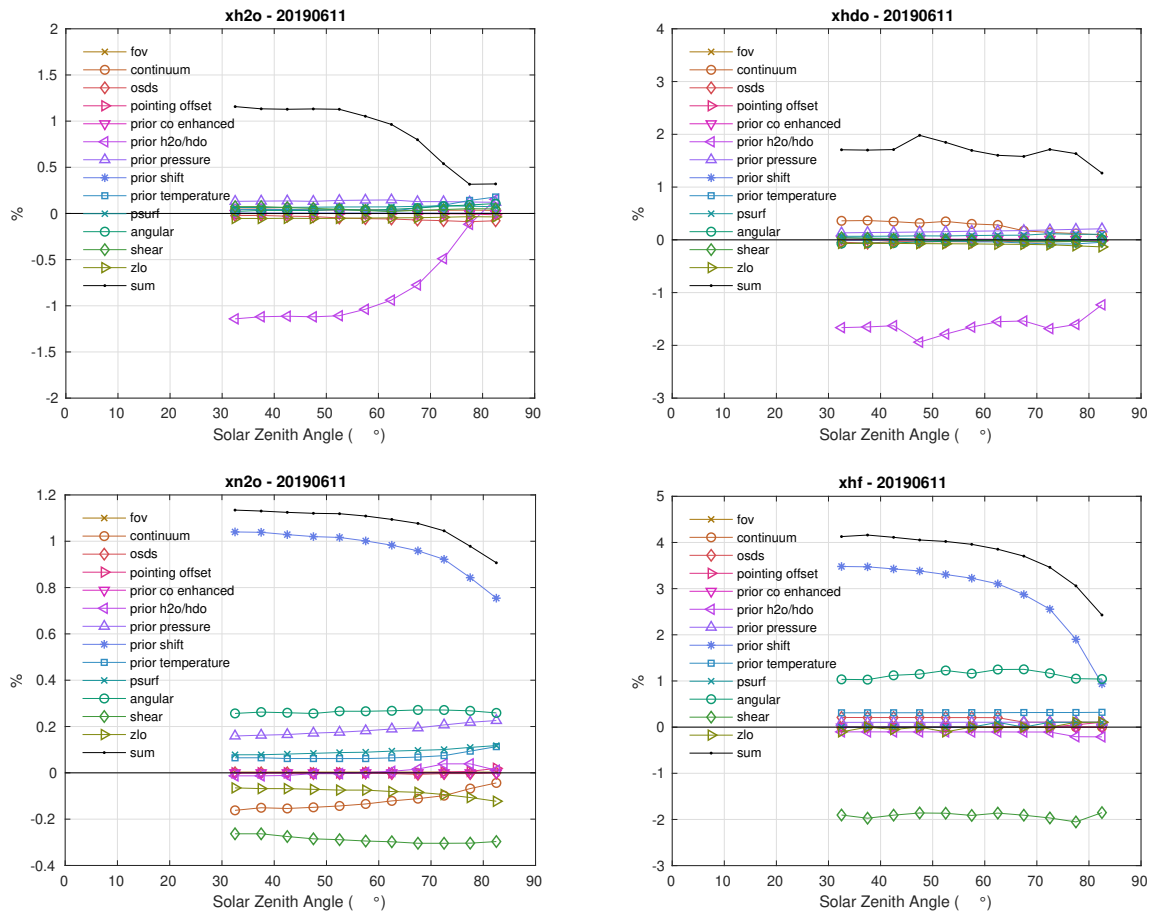
Figure 24. As in Figure 23, but for X_{H_2O} , X_{HDO} , X_{N_2O} , and X_{HF} .
