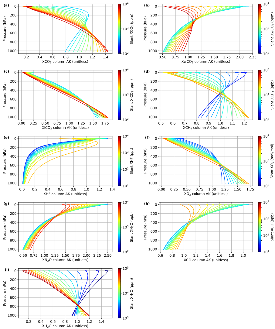
Figure 5. Precomputed column AKs for TCCON X_{\text{gas}} products: (a) X_{\text{CO}_2} , (b) X_{\text{wCO}_2} , (c) X_{\text{ICO}_2} , (d) X_{\text{CH}_4} , (e) X_{\text{HF}} , (f) X_{\text{O}_2} , (g) X_{\text{N}_2\text{O}} , (h) X_{\text{CO}} , (i) X_{\text{H}_2\text{O}} , and (j) X_{\text{HDO}} .
