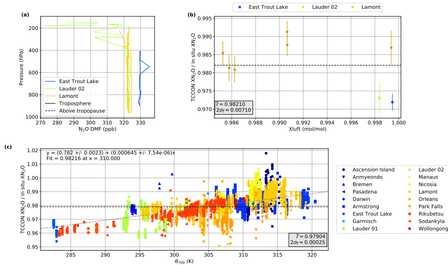
Figure 19. (a) The available N 2 O profiles over TCCON sites from the NOAA CCGG Aircraft Program v1.0 ObsPack (Sweeney et al., 2018). (b) TCCON/in situ ratio vs. X_{\text{lufft}} similar to Fig. 16, but for N 2 O. (c) The TCCON/in situ X_{\text{N}_2\text{O}} ratio derived using surface NOAA N 2 O data versus mid-tropospheric potential temperature. The dashed gray line is a robust fit to the data. The text in the lower right hand corner gives the mean TCCON/in situ ratio (denoted also by the horizontal dashed black line) and its 2\sigma standard deviation. The points are colored by TCCON site.
