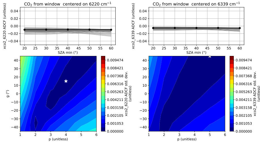
Figure 11. Example of how g and p in Eq. (5) were chosen for the two TCCON \text{CO}_2 windows. The left two panels are for the \text{CO}_2 window centered at 6220 \text{ cm}^{-1} and the right two for the window at 6339 \text{ cm}^{-1} . The line plots at the top show how the value of the ADCF changes as we increase the lower limit in SZA for the data fit to. Each gray line represents one combination of g and p , with the black line representing the combination with the smallest standard deviation in the ADCF. The contour plots show the standard deviation of the ADCF across different minimum SZAs for each combination of g and p . The white star represents the combination with the smallest standard deviation; it corresponds to the test show with the black line in the line plots.
