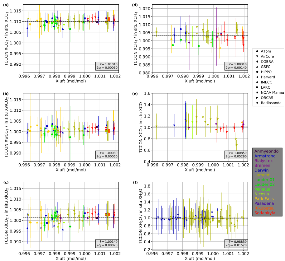
Figure 16. Plots of the TCCON/in situ X_{\text{gas}} ratios for (a) \text{CO}_2 , (b) w\text{CO}_2 , (c) l\text{CO}_2 , (d) \text{CH}_4 , (e) \text{CO} , and (f) \text{H}_2\text{O} . In all plots, the y -axis is the ratio of TCCON/in situ X_{\text{gas}} and the x -axis is the median X_{\text{lufft}} value for the TCCON observations in a comparison (see text for explanation of X_{\text{lufft}} ). The marker style of each comparison indicates the source of the in situ data and the color indicates which TCCON site the comparison occurred at. The text inset in the lower-right corner of each plot gives the uncertainty-weighted mean TCCON/in situ ratio and its 2\sigma uncertainty. The dashed black lines mark the mean ratio. Panels a, b, and c are set to use the same y -limits; some of the error bars in (b) go outside the y -limits.
