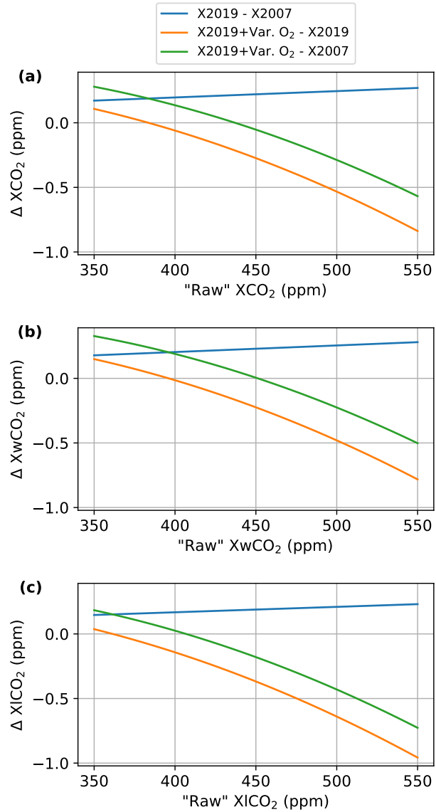
Figure 17. The change in TCCON (a) X_{\text{CO}_2} , (b) X_{\text{wCO}_2} , and (c) X_{\text{ICO}_2} due to the WMO scale change, change in assumed \text{O}_2 dry mole fraction, and the combination of both. The x -axis is the “raw” X_{\text{CO}_2} value that has no in situ bias correction and assumes a fixed \text{O}_2 dry mole fraction. The “X2019 – X2007” line shows the difference due to only the \text{CO}_2 WMO scale change, the “X2019+Var \text{O}_2 – X2019” shows the difference due to only the change from fixed to variable \text{O}_2 dry mole fraction, and the “X2019+Var. \text{O}_2 – X2007” line shows the total change from both effects combined.
