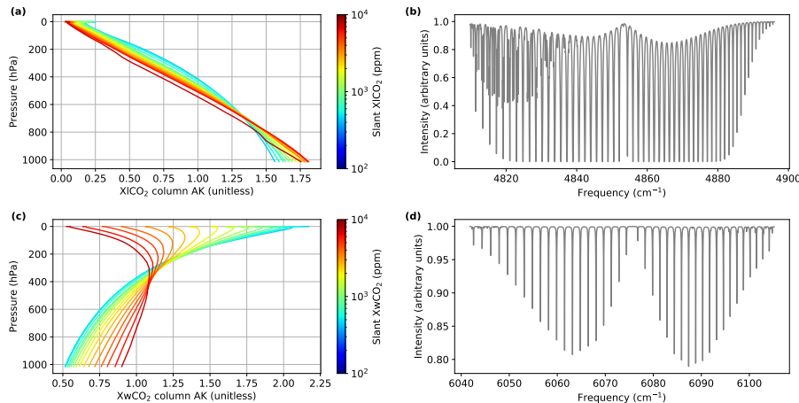
Figure 3. Column averaging kernels (panels a , c ) and calculated CO 2 absorption lines (panels b , d ) in the ICO 2 (panels a , b ) and wCO 2 (panels c , d ) windows, respectively. The absorption lines in panels (b) and (d) are for a TCCON spectrum measured at solar zenith angle = 39.684° in Jul 2004 at Park Falls, WI, USA. In panels (a) and (c), the different colors indicate AKs for different slant X_{\text{gas}} amounts. “Slant X_{\text{gas}} ” is a measure of total absorber column along the light path. See §3.1 for details.
