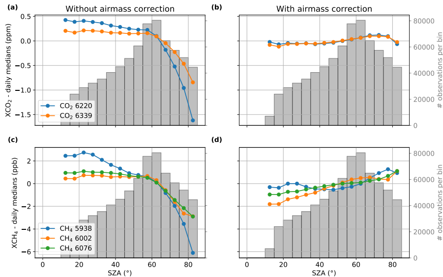
Figure 10. Variation of (a,b) the two CO 2 and (c,d) three CH 4 windows used by TCCON with SZA. (a) and (c) are without the airmass correction applied, (b) and (d) are with the correction applied. In all panels, the y -axis is column-average dry mole fraction of CO 2 or CH 4 derived from a single spectral window, with the central wavenumber given in the legend. The y values have the daily median values subtracted (to remove day-to-day variability), and each point represents the median of all such values in a 5° SZA bin. The grey bars give the number of observations in each 5° SZA bin (this is the same in all panels).
