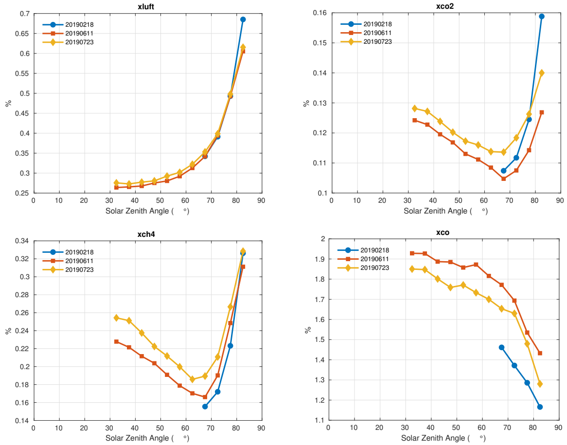
Figure 26. These figures show the sum in quadrature of all the errors plotted in Figure 23 for all three dates. The errors plotted here are for X_{\text{luf}t} , X_{\text{CO}_2} , X_{\text{CH}_4} , and X_{\text{CO}} .
