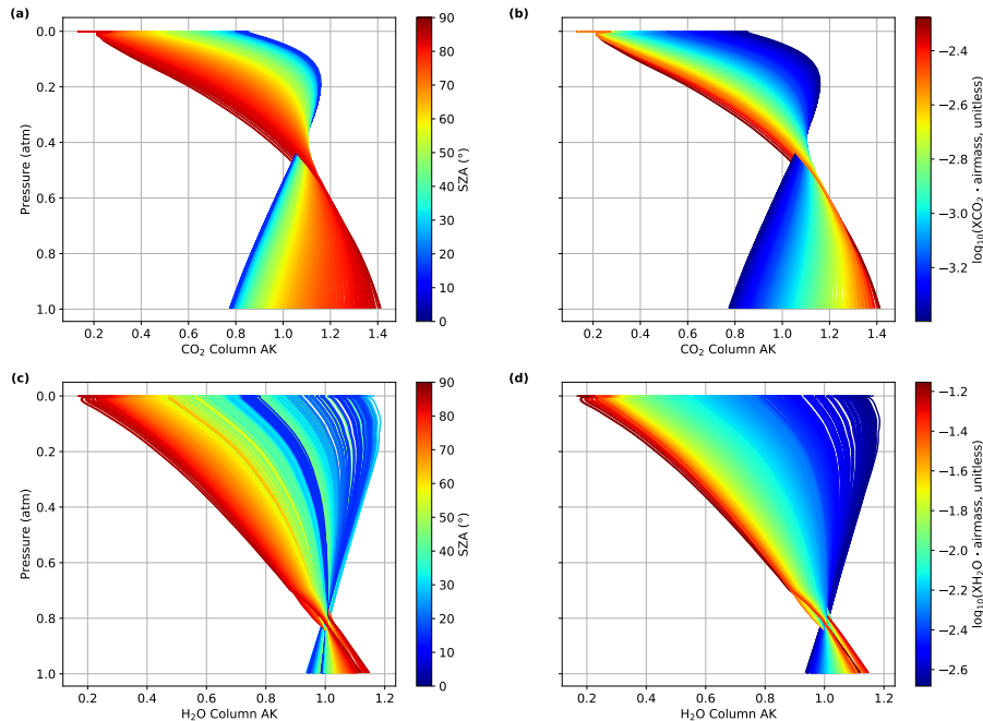
Figure 4. CO 2 and H 2 O AKs from four days’ measurements at the TCCON site in Lamont, OK, USA. (a) CO 2 AKs binned by SZA. (b) CO 2 AKs binned by slant X_{\text{CO}_2} . (c) H 2 O AKs binned by SZA. (d) H 2 O AKs binned by slant X_{\text{H}_2\text{O}} .
