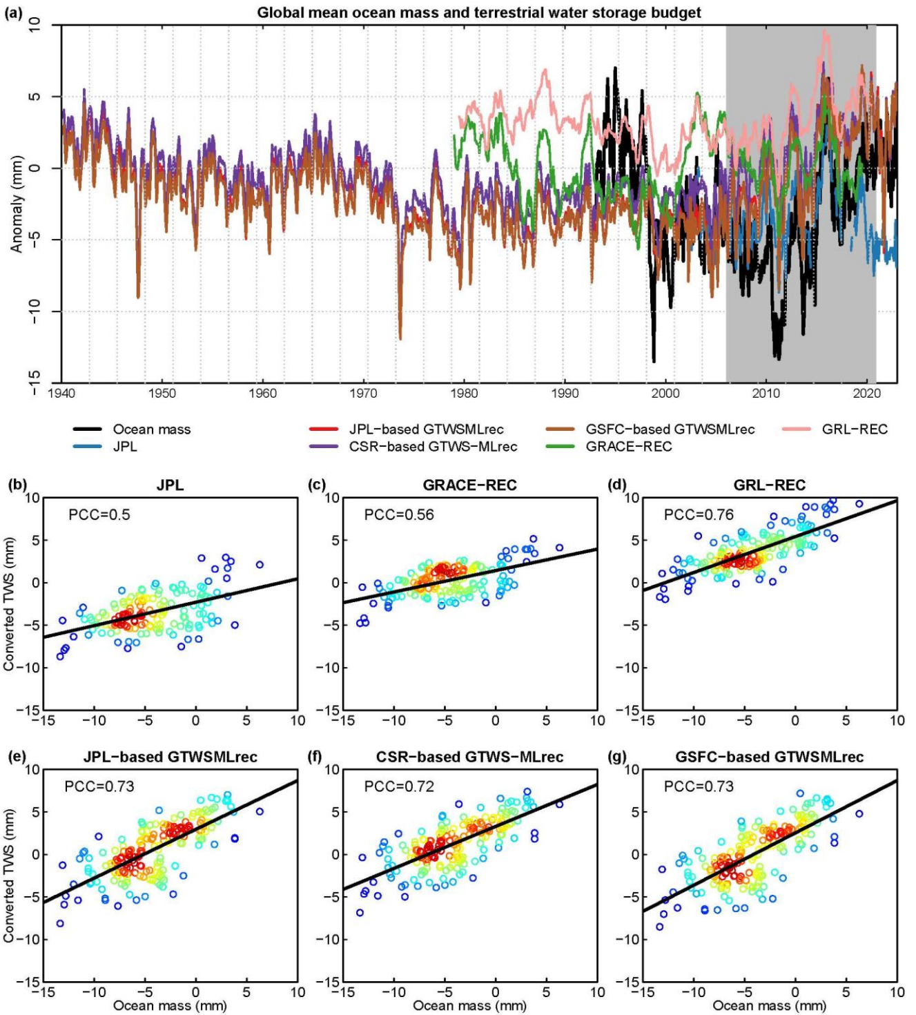
Figure 5. Comparison of the global average TWS variations (converted to equivalent sea level; unit: mm) against ocean mass changes derived from the sea level budget. a , the temporal dynamics of global average sea level and TWS. b-g , the regression plots of sea level and converted TWS; warmer (colder) colour indicates higher (lower) density of points; the black line denotes the linear regression. The converted TWS is estimated after extracting the trend and seasonal signals from the negative values of primary datasets by considering land-ocean area ratio.
