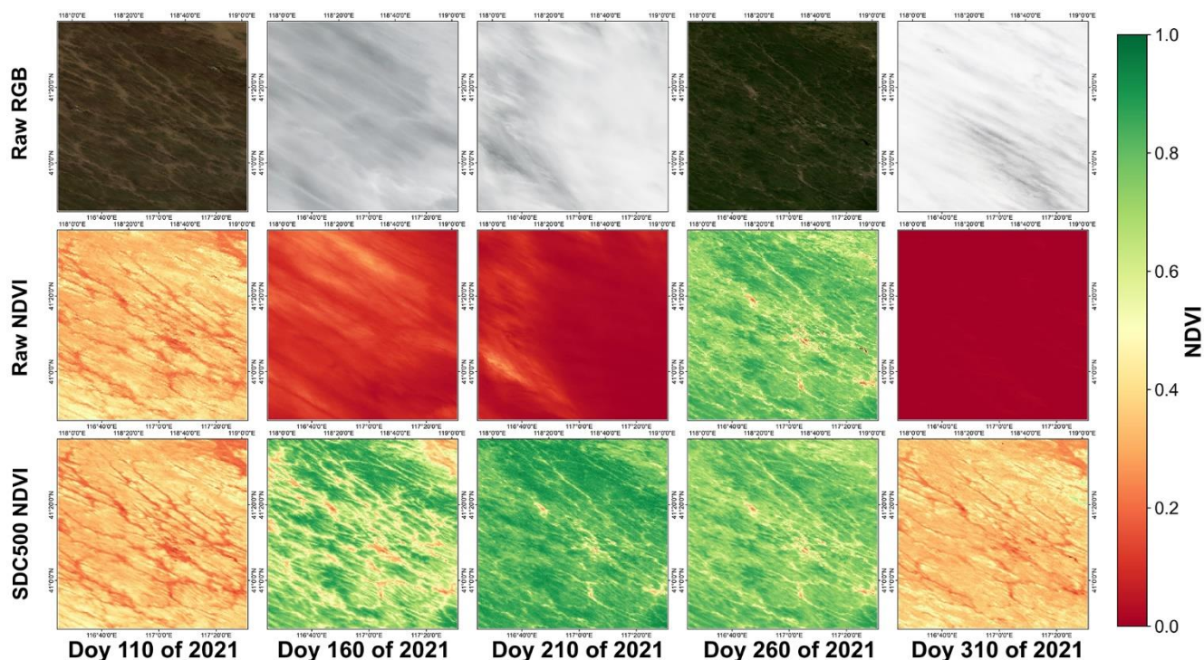
385 Figure 13: Assessment of spatial pattern on a cropland area (site S5). True-colour composite (R: Band 1; G: Band 4; B: Band 3) and Raw MODIS NDVI and SDC500 NDVI imagerys on 5 dates in 2021.
