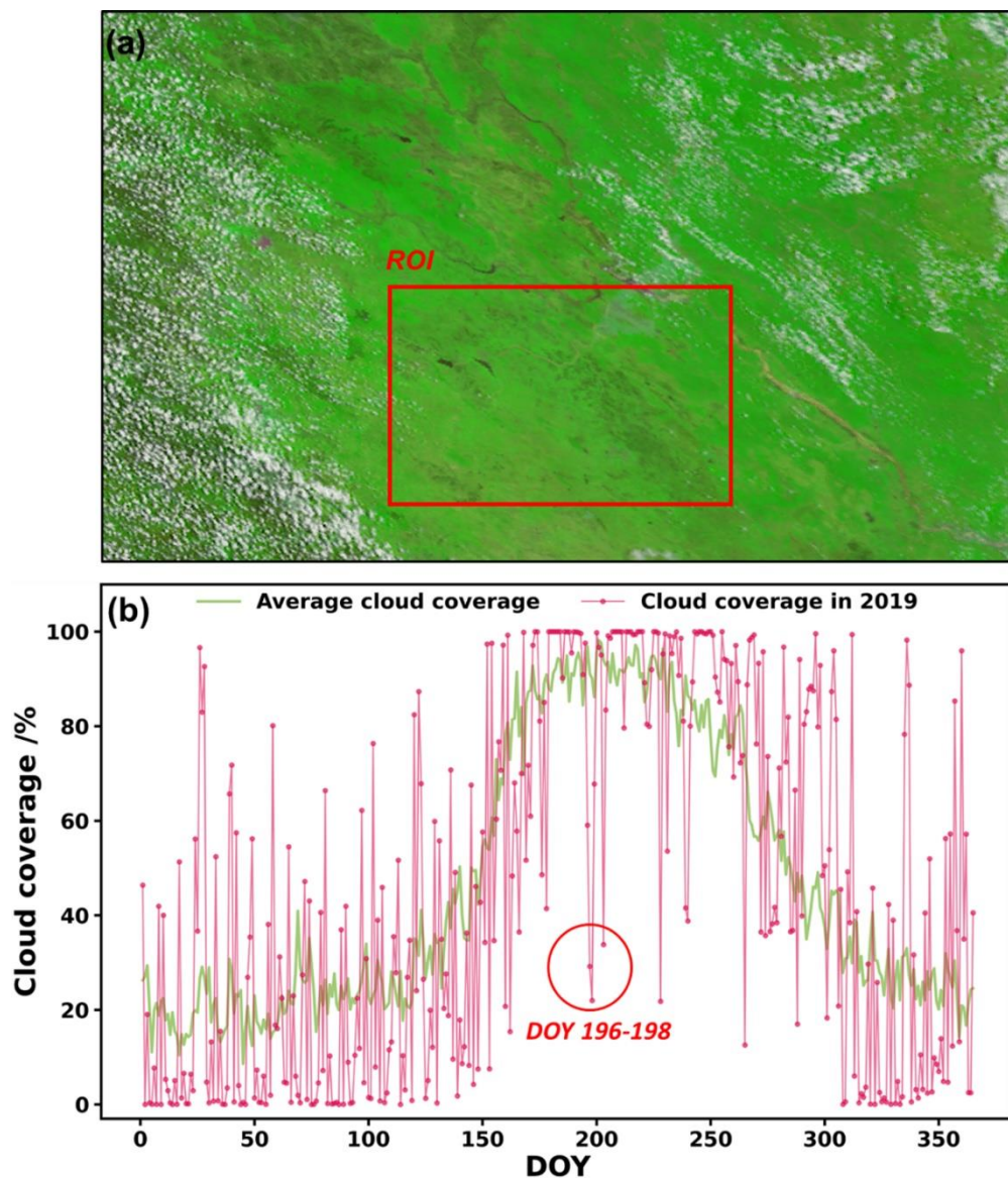
465 Figure 19: Study area of quantitative validation. (a) Original MODIS observation on 2019/197, in tile h25v07, line 1-600, column 801-1800. (R: Band 1; G: Band 2; B: Band 3) The region of interest (ROI) outlined by the red box indicates the clear area to derive validation statistics. (b) Average cloud coverage in the period of 2000-2022 and cloud coverage in 2019.
