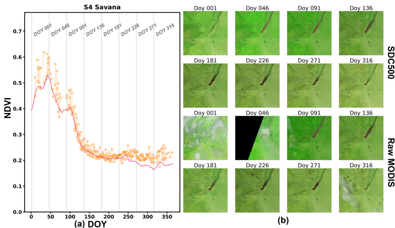
350 Figure 9: Performance of SDC in site S4: (a) The NDVI curves for the central pixel, the orange points indicate the valid MODIS observation and the red line indicates the SDC500 results. (b) The spatial pattern of image blocks of 200*200 pixels centred around the site (R: Band 1; G: Band 2; B: Band 3).
