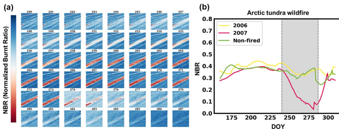
Figure 22: The performance of SDC500 during the Arctic tundra wildfire in 2007 summer. (a) The spatial pattern of NBR. (b) The NBR series for a central pixel of burned area in 2006(before burn) and 2007(burn), and a non-fired pixel in 2007.
