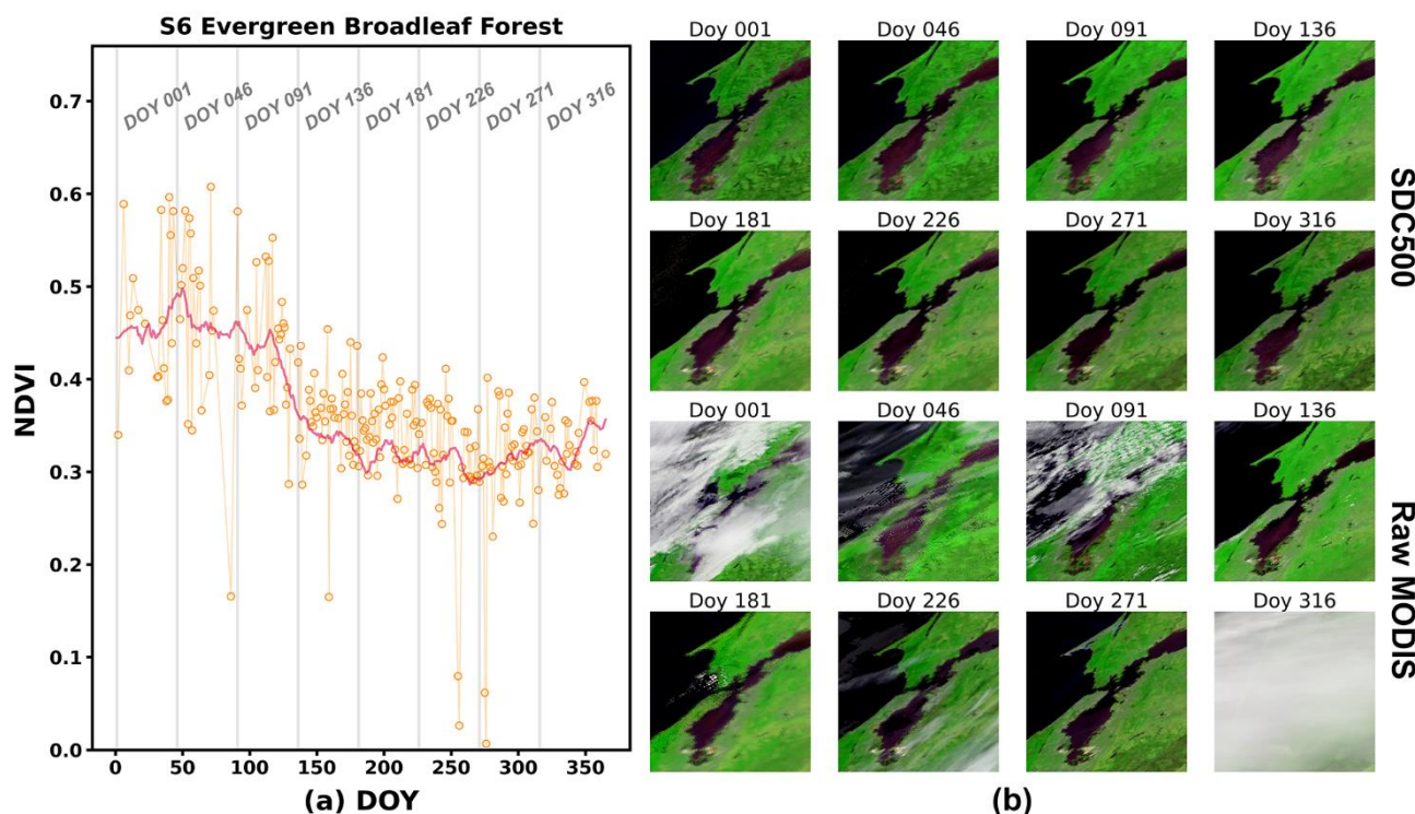
395 Figure 14: Performance of SDC in site S6. (a) The NDVI curves for the central pixel, the orange points indicate the valid MODIS observation and the red line indicates the SDC500 results. (b) The spatial pattern of image blocks of 200*200 pixels centred around the site (R: Band 1; G: Band 2; B: Band 3).
