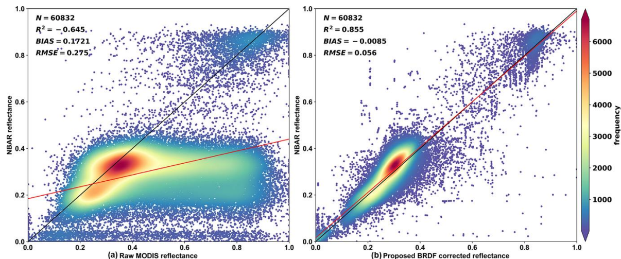
445 Figure 18: Quantitative evaluation of our proposed BRDF correction method: (a) raw MODIS reflectance vs. MODIS NBAR product, and (b) SDC500 dataset vs. MODIS NBAR product.
