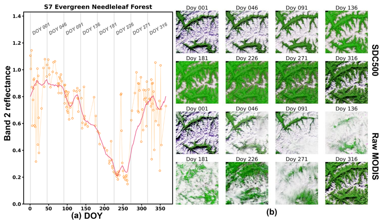
405 Figure 15: Performance of SDC in site S7: (a) The band 2 reflectance curves for the central pixel, the orange points indicate the valid MODIS observation and the red line indicates the SDC500 results. (b) The spatial pattern of image blocks of 200*200 pixels centred around the site (R: Band 1; G: Band 2; B: Band 3).
