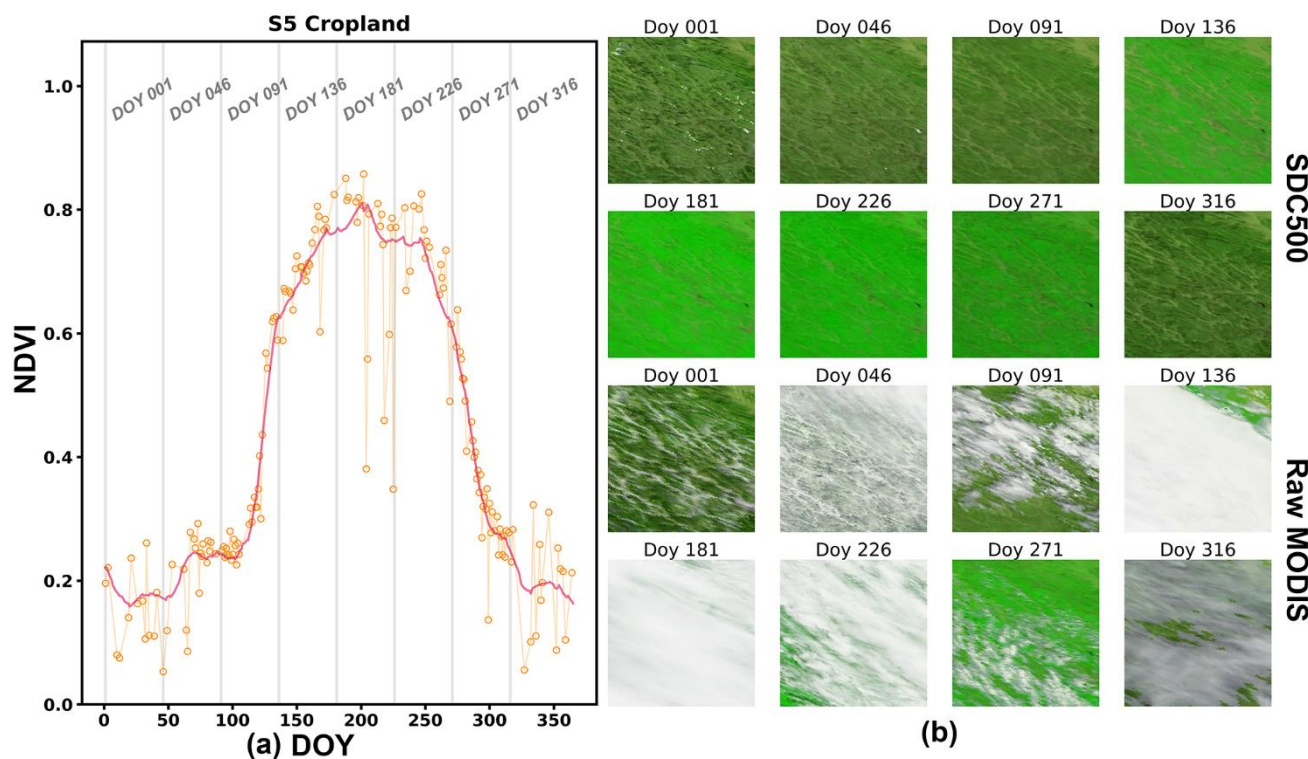
375 Figure 10: Performance of SDC in site S5: (a) The NDVI curves for the central pixel, the orange points indicate the valid MODIS observation and the red line indicates the SDC500 results. (b) The spatial pattern of image blocks of 200*200 pixels centred around the site (R: Band 1; G: Band 2; B: Band 3).
