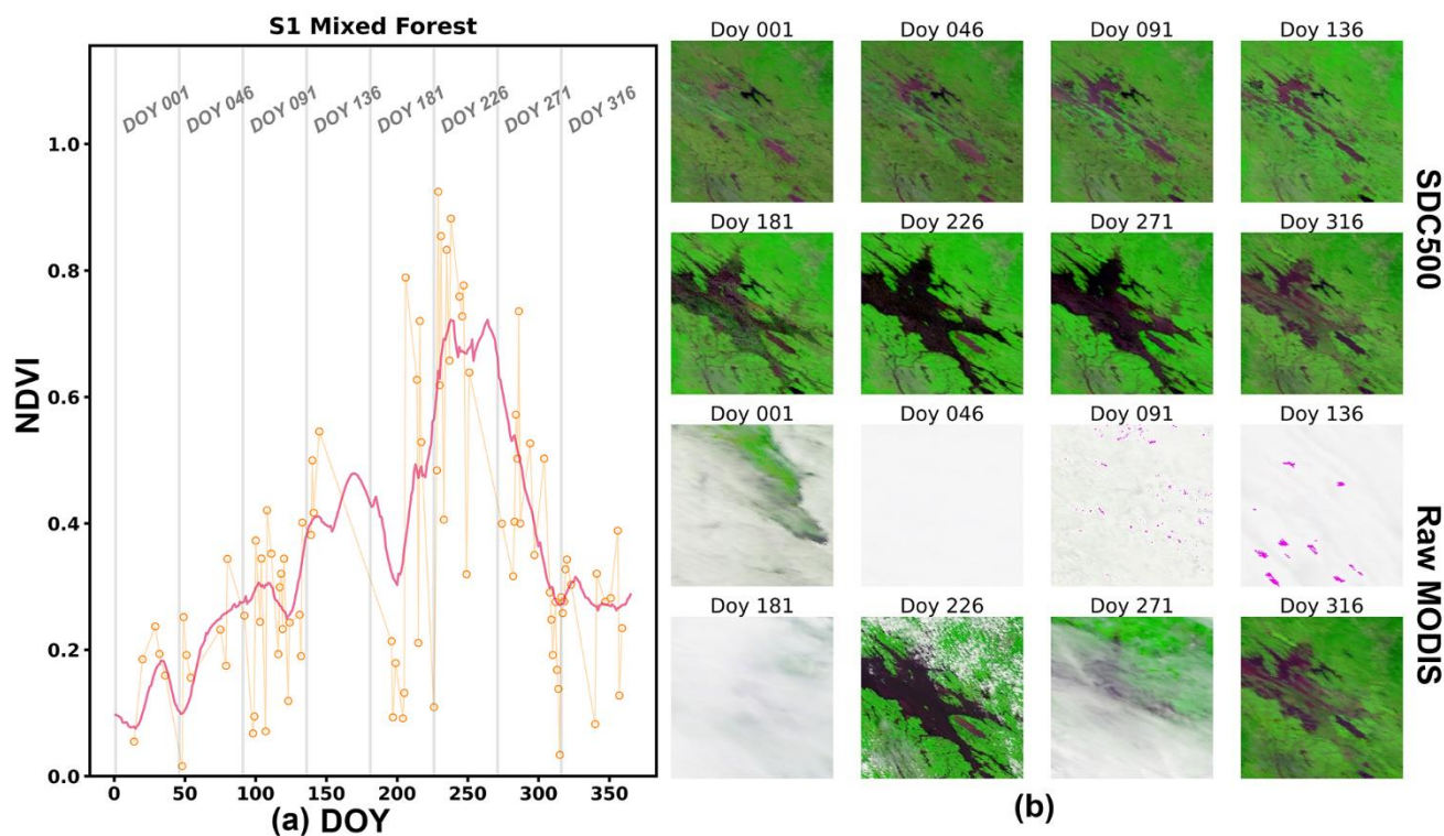
325 Figure 6: Performance of SDC in site S1: (a) The NDVI curves for the central pixel, the orange points indicate the valid MODIS observation and the red line indicates the SDC500 results. (b) The spatial pattern of reconstructed and raw image blocks of 200*200 pixels centred around the site (R: Band 1; G: Band 2; B: Band 3).
