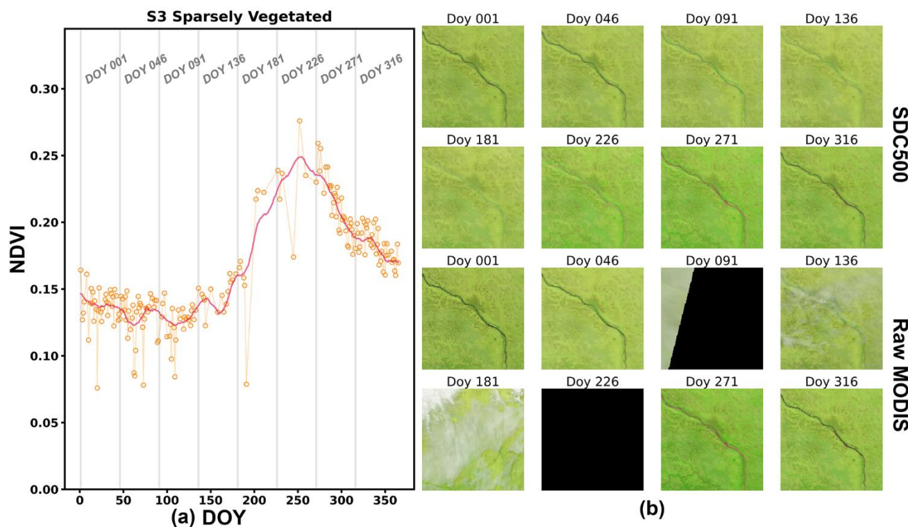
345 Figure 8: Performance of SDC in site S3: (a) The NDVI curves for the central pixel, the orange points indicate the valid MODIS observation and the red line indicates the SDC500 results. (b) The spatial pattern of image blocks of 200*200 pixels centred around the site (R: Band 1; G: Band 2; B: Band 3).
