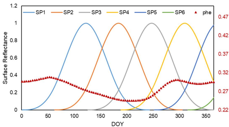
220 Figure 2: Illustration of the B-spline base functions (SP1, ..., SP6) and the surface reflectance phenology curve (PHE) of MODIS band 1.
