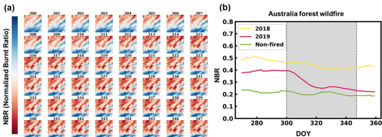
505 Figure 23: The performance of SDC500 during the Australia forest wildfire. (a) The spatial pattern of NBR. (b) A central pixel of burned area in 2018(before burn) and 2019(burn), and a non-fired pixel in 2019.
