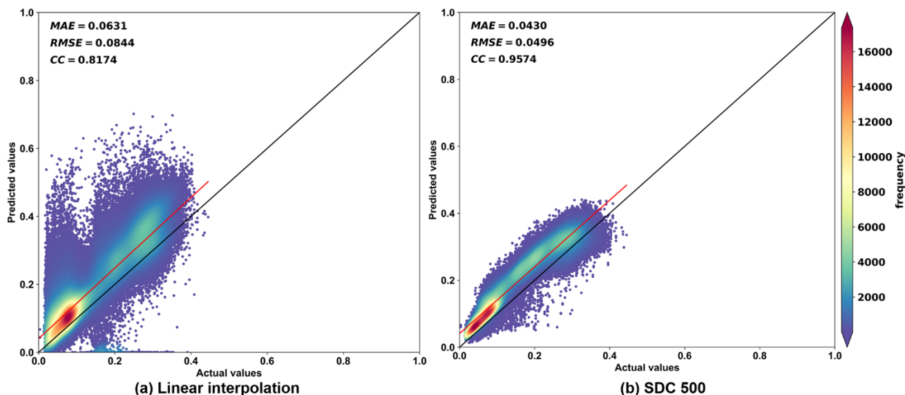
475 Figure 21: Quantitative comparison between actual values and predicted values of Linear interpolation (a) and SDC500 (b).
