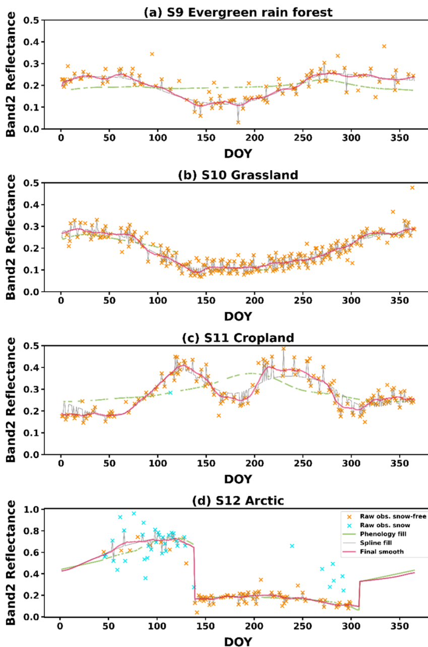
305 Figure 5: Comparison of BRDF adjusted raw MODIS observations, gap-filled values with phenology curve, gap-filled values with B-spline, and the final smoothed series in typical sites: Site S9 Evergreen rain forest (a), Site S10 Grassland (b), Site S11 Cropland (c) and Site S12 Arctic (d).
