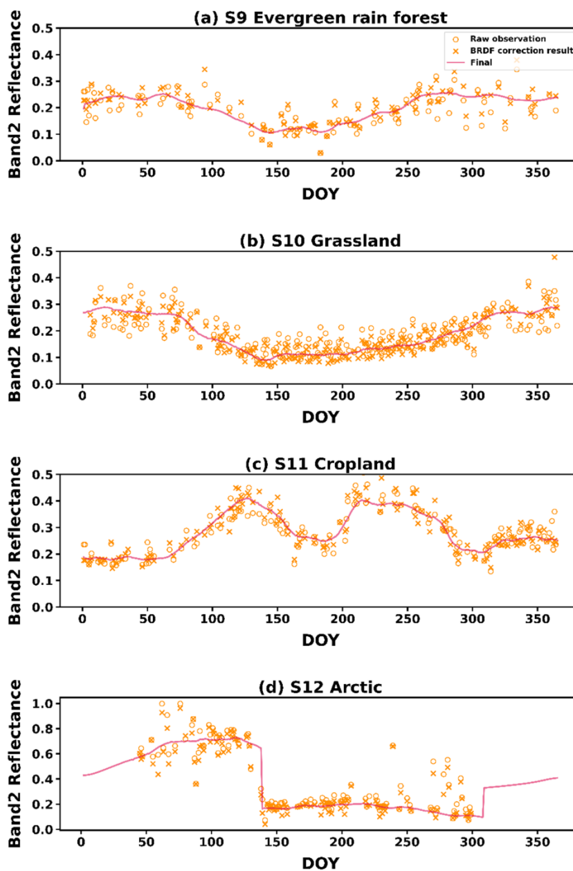
440 Figure 17: Example of series of raw MODIS observations, BRDF corrected observations, and the final smoothed series in four typical sites: Site S9 Evergreen rain forest (a), Site S10 Grassland (b), Site S11 Cropland (c), and Site S12 Arctic (d).
