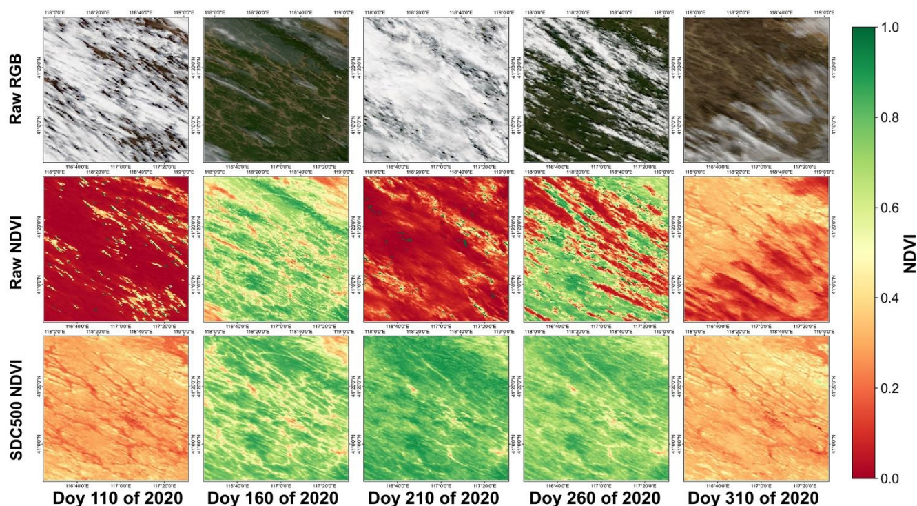
Figure 12: Assessment of spatial pattern on a cropland area (site S5). True-colour composite (R: Band 1; G: Band 4; B: Band 3) and Raw MODIS NDVI and SDC500 NDVI imageries on 5 dates in 2020.
