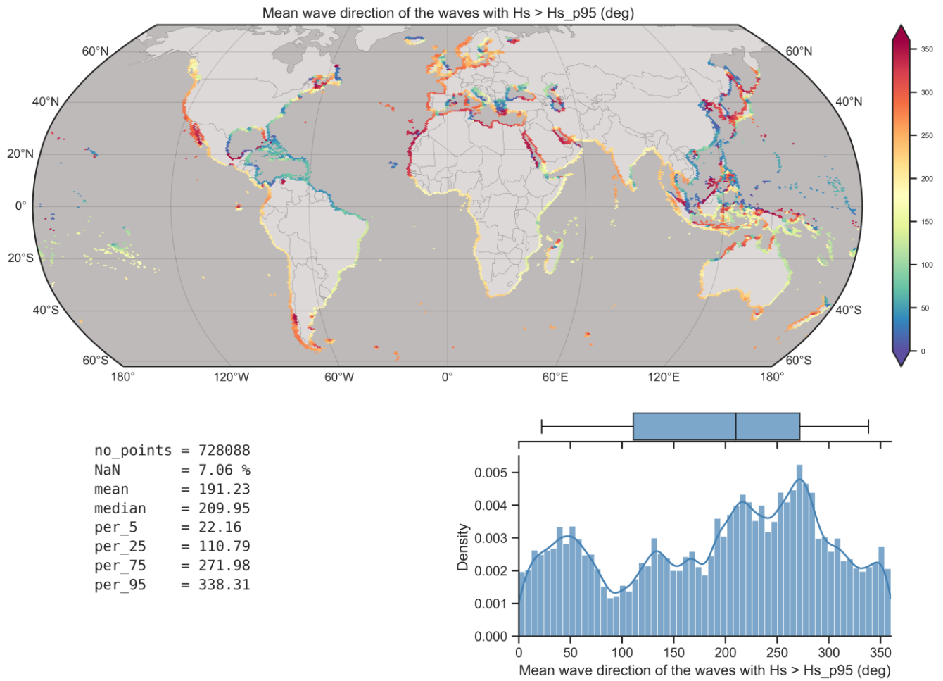
Figure 8: Global map and statistics of Average Mean Wave Direction (MWD) relative to true North, when H_s \geq H_{s\_p95} (1979-2019). Top: Global map showing the median values in hexagons with a size of \sim 1 degree. Bottom right: Histogram and boxplot (with the lines showing the 5th and 95th percentiles, the box the 25th and 75th percentiles, and the vertical line the median) of Average Mean Wave Direction (MWD) at the transect level. Bottom left: various global statistics.
