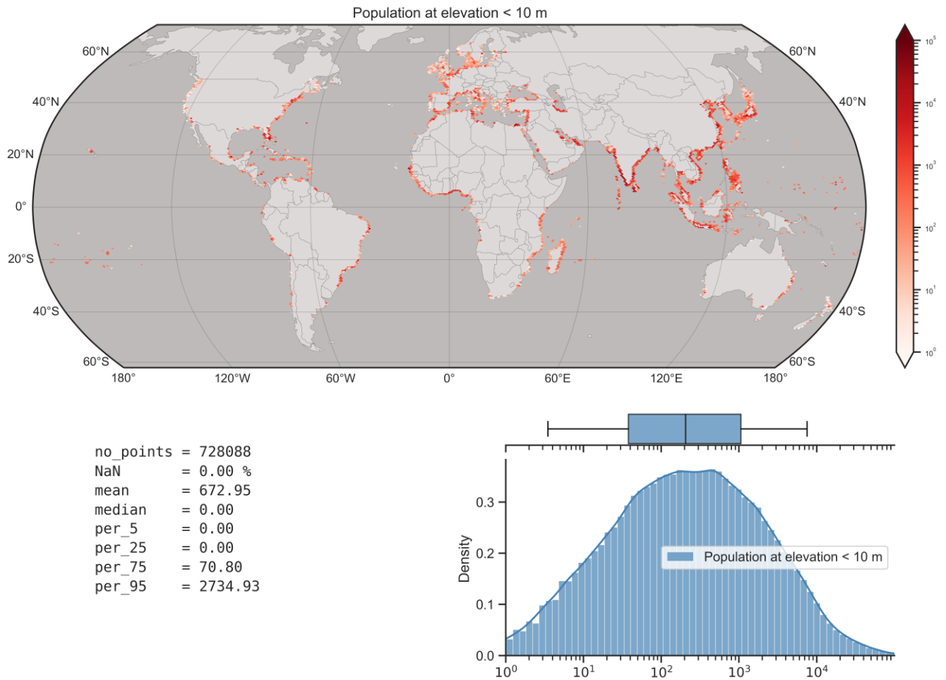
Figure 98: Global map and statistics of population at elevation < 10 m. Top: Global map showing the median values in hexagons with a size of ~1 degree. Hexagons with no population are not plotted. Colorbar is given in a logarithmic scale. Bottom right: Histogram and boxplot (with the lines showing the 5th and 95 percentiles, the box the 25th and 75th percentiles, and the vertical line the median) describing the transects with at least one person. The x axis is plotted in logarithmic scale. Bottom left: various global statistics (including transects with 0 population at elevation < 10 m).
