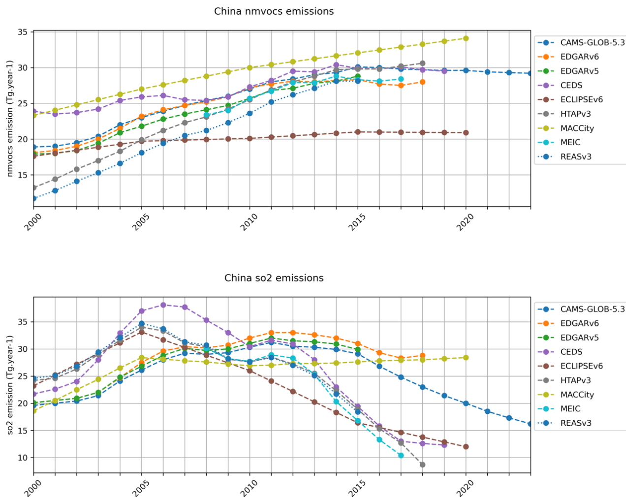
840 Figure 12: comparisons of the CAMS-GLOB-ANT_v5.3 emissions for CO, NO x , NMVOCs and SO 2 with other global datasets and two regional inventories for China
