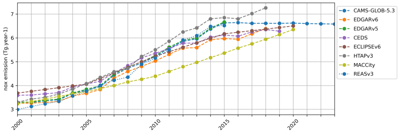
India nox emissions
